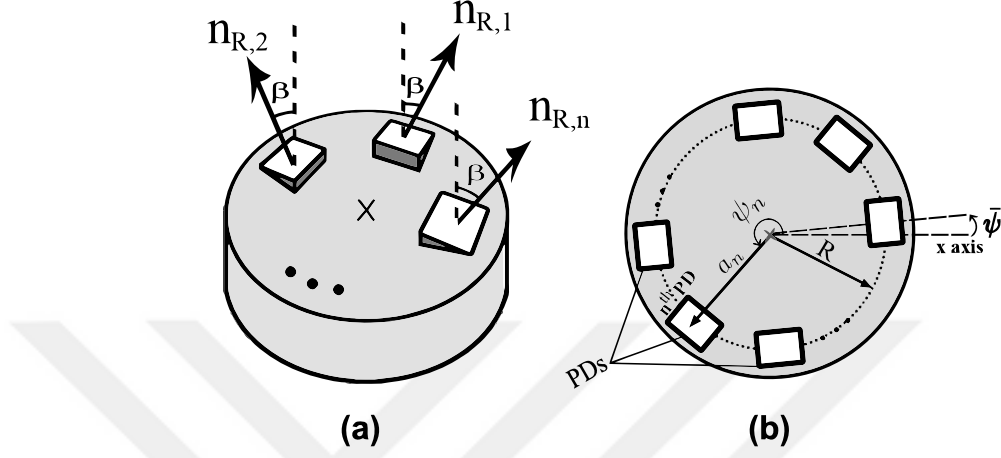
Figure 3.1: Uniform circular layout. (a) Three-dimensional view. (b) Top view.
