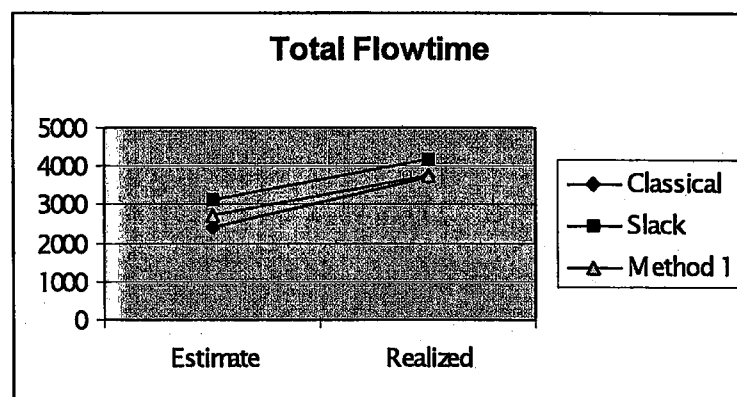
c) Total Flow Time Estimate-Realized Graph
