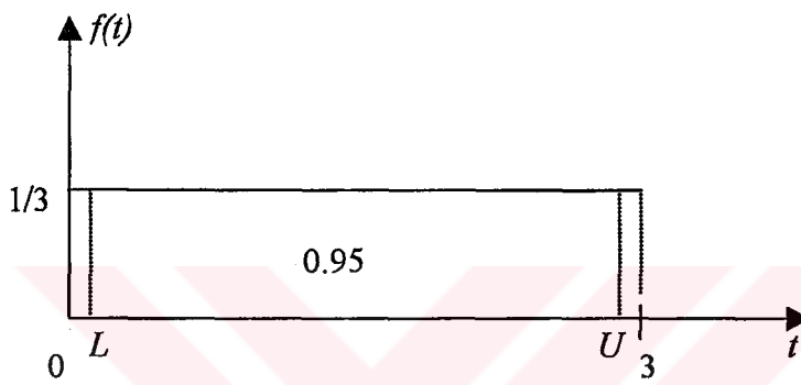
Figure 8. L and U Parameters of Method 1
