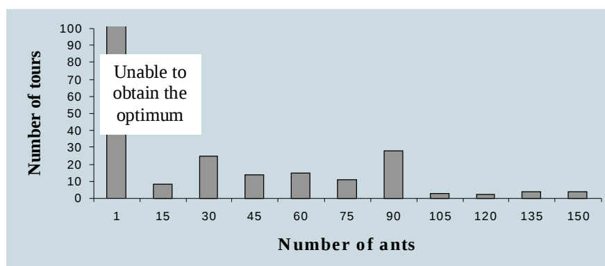
Figure 5.3.c: Number of tours required to obtain the optimum number of stations. Barthold problem with 148 tasks, C=805 . The experiment has been carried out for (1 replications • 100 ant tours).
