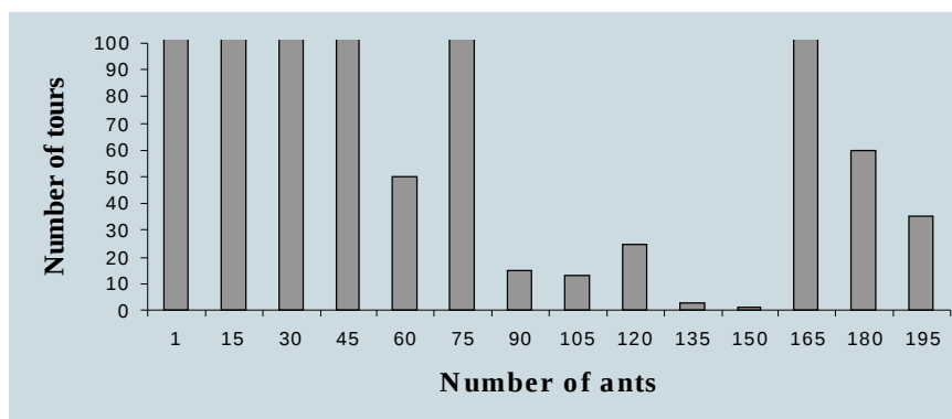
Figure 5.1.c: Number of tours required to obtain the optimum number of stations. Barthold problem with 148 tasks, C=805 . The experiment has been carried out for (1 replications • 100 ant tours).
