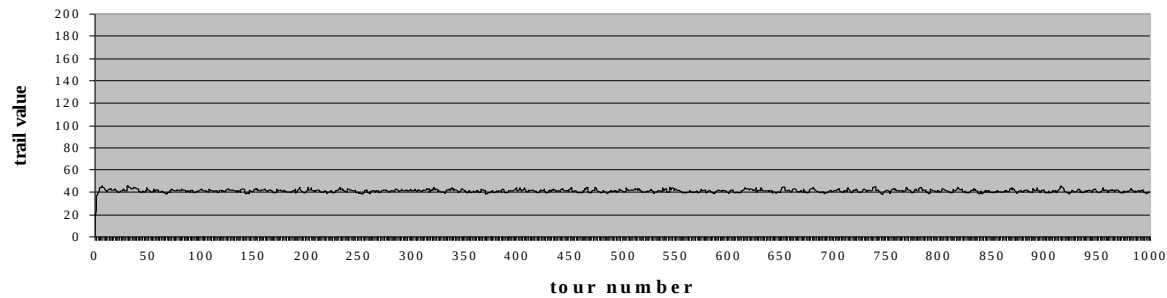
Figure 4.9.c: Trail accumulation for the new method, a = 1 , b = 1 , r_1 = r_2 = 0.95 , q_0 = 0.3 , initial trail = 1
