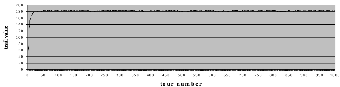
Figure 4.9.d: Trail accumulation for the new method, a = 1 , b = 1 , r_1 = r_2 = 0.99 , q_0 = 0.3 , initial trail = 1
