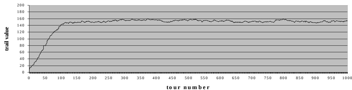
Figure 4.9.e: Trail accumulation for the new method, a = 1 , b = 1 , r_1 = r_2 = 0.99 , q_0 = 0.8 , initial trail = 1
