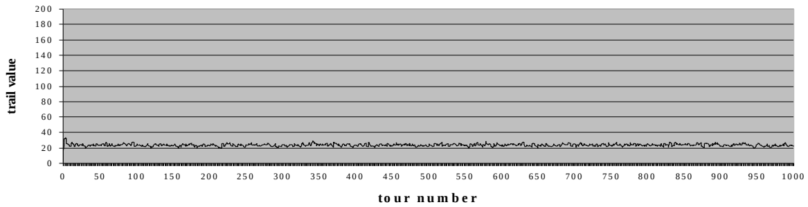
Figure 4.9.b: Trail accumulation for the new method, a = 1 , b = 1 , r_1 = r_2 = 0.9 , q_0 = 0.3 , initial trail = 1
