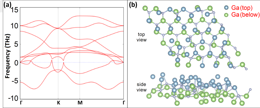
Figure 5.6: a) Phonon dispersion curves for Ga-Ga DB + GaN monolayer for 1x1 unitcell, b) Snapshots of atomic configurations at 1 ps (300 K), in which honeycomb-like structures are not maintained.
