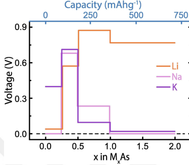
Figure 4.5: Average open-circuit voltages for SL- hb -As coated with alkali metals (Li, Na, and K) with varying concentration ( M_x As ). The optimized (amorphous) structures are obtained with ab initio molecular dynamics calculations performed at ambient temperature.
