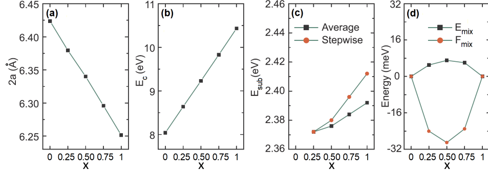
Figure 3.2: The variation of (a) Lattice constant, (b) Cohesive energy, E_c (c) Substitution energy, E_{sub} , and (d) Mixing energy, E_{mix} with x .
