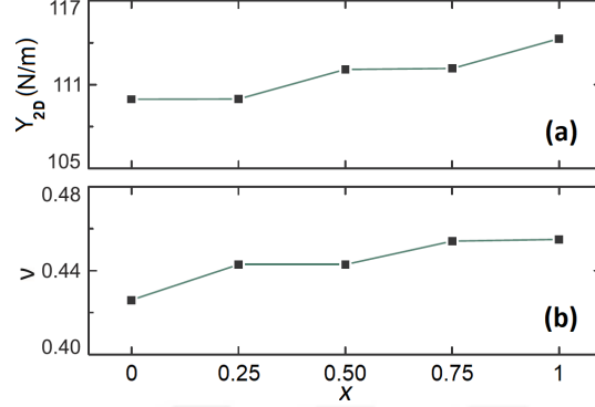
Figure 3.6: The variation of (a) in-plane stiffness ( Y_{2D} ) and (b) Poisson's ratio ( \nu ) with x .
