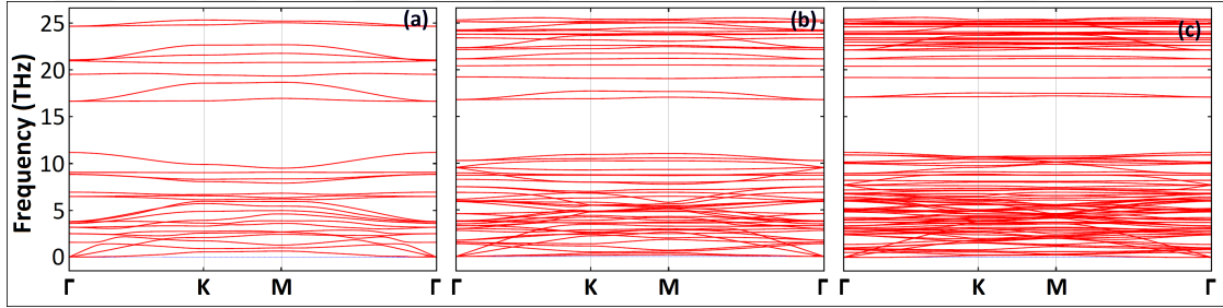
Figure 5.8: Phonon dispersion curves for Ga-Ga DB + GaN monolayer for (a) 2x2, (b) 3x3, (c) 4x4 unitcells.
