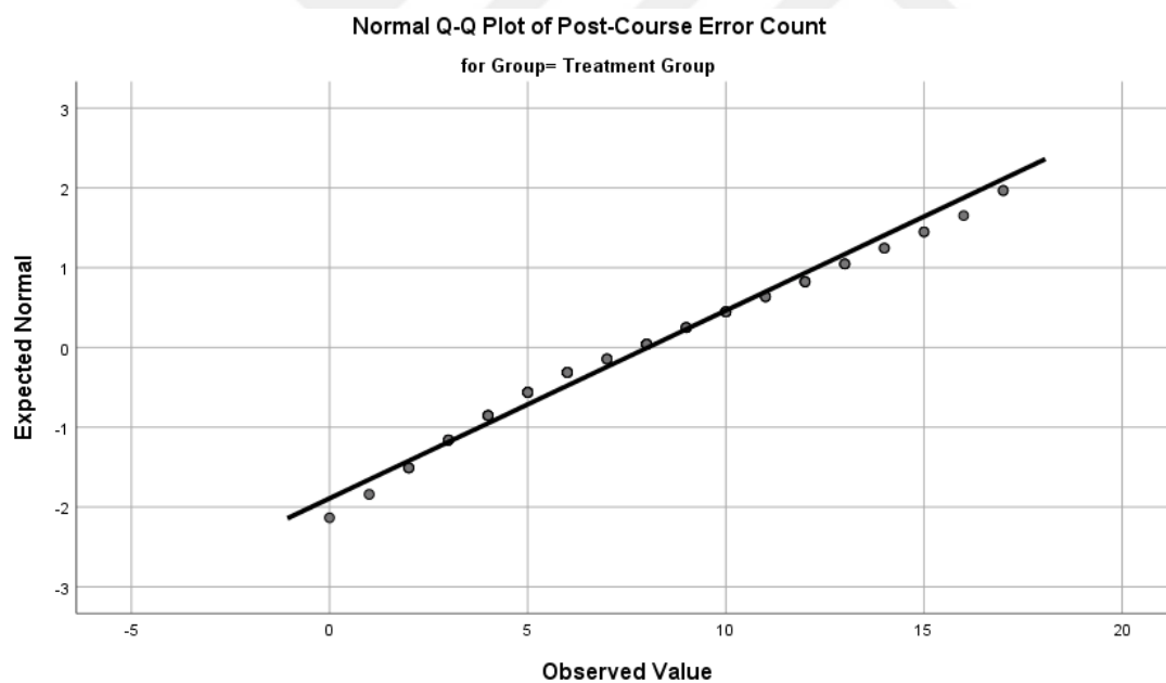
Figure 4.7. Q-Q Plot Of The Post-course Error Count For The Treatment Group
