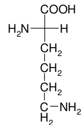
α,ε-Diamino-kapronik asit L (+) Lisin (Lys)
