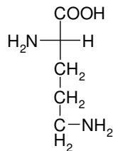
α,δ-Diamino-valerik asit L(+)-Ornithin (Orn)
