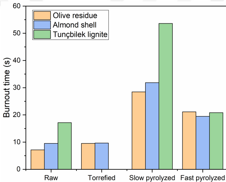
Figure 4.17 Burnout times for selected particles with 2 ( \pm 0.2 ) mg mass, for all studied fuels
