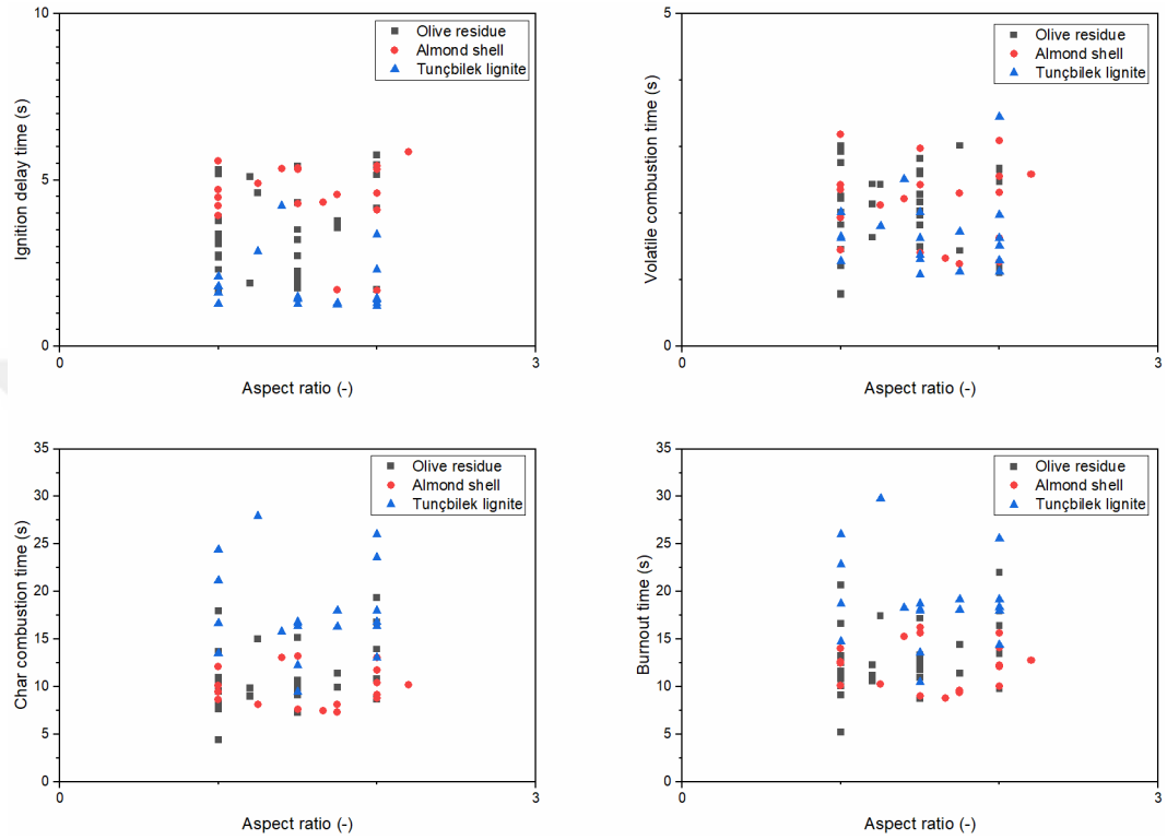
Figure 4.18 Ignition delay time, volatile combustion time, char combustion time, and burnout combustion time as a function of the particle aspect ratio for all raw fuels studied.
