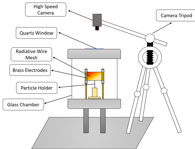
Figure 3.12 Schematic of the vertical wire mesh reactor used for single-particle combustion trials.
