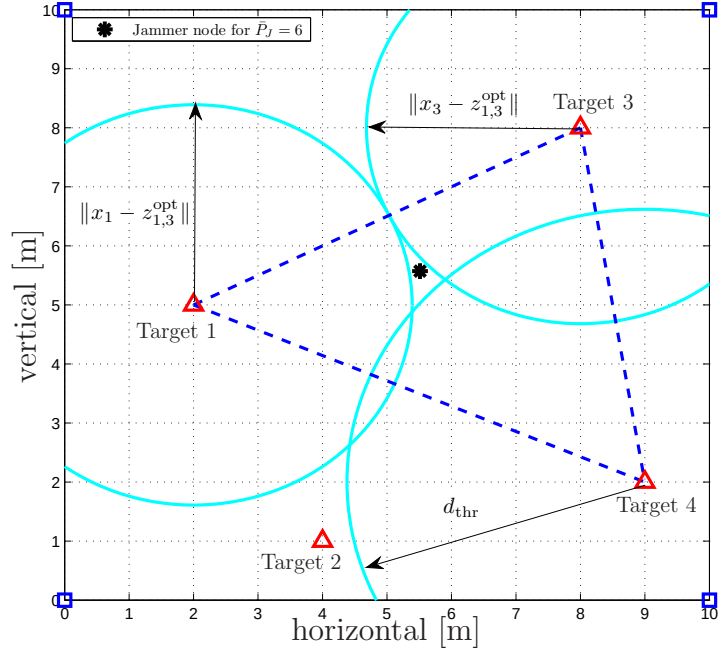
Figure 6.4: Illustration of Corollary 2 for the scenario in Fig. 6.3.
