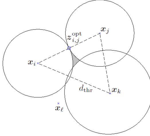
Figure 4.2: The scenario in Corollary 2, where the optimal location for the jammer node corresponds to a point in the shaded (gray) area.
