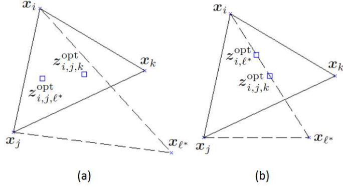
Figure A.4: Illustration for Case 1 of the proof of Proposition 7: (a) Case 1-(a), (b) Case 1-(b).
