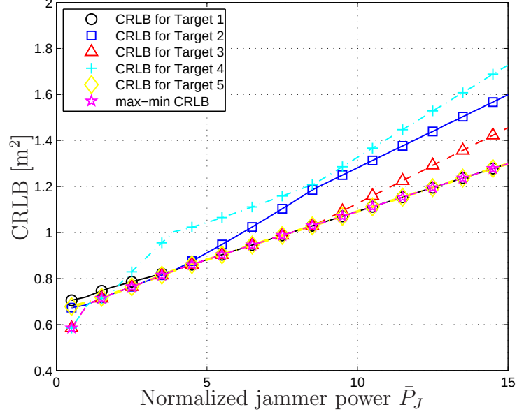
Figure 6.7: CRLB corresponding to each target node and max-min CRLB for the whole network for the scenario in Fig. 6.6.
