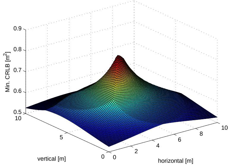
Figure 7.4: The minimum CRLB of the target nodes versus the location of the jammer node for the network presented in Fig. 7.3-(a).
