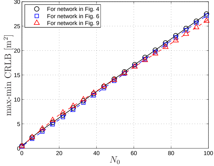
Figure 6.8: Max-min CRLB for the networks in Fig. 6.1, Fig. 6.3, and Fig. 6.6 versus the spectral density level of the measurement noise, N_0 , where P_J = 10 .
