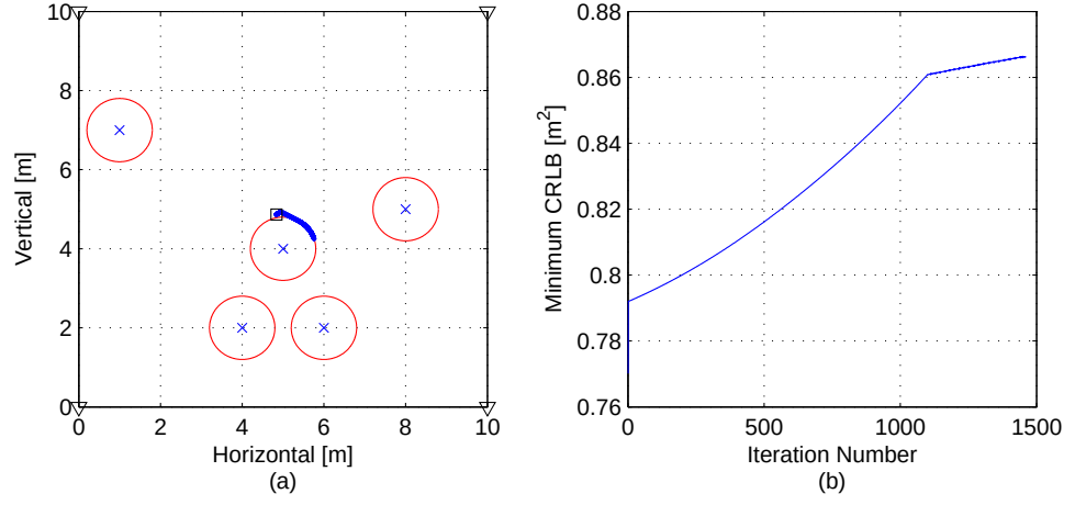
Figure 7.5: An illustration of the algorithm for a network in which the target nodes are at [1 \ 7] , [4 \ 2] , [5 \ 4] , [6 \ 2] , and [8 \ 5] m. (a) The network and the jammer path. (b) The minimum CRLB in the system during the iterations of the algorithm.
