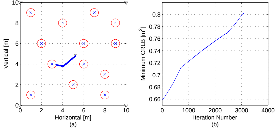
Figure 7.3: An illustration of the algorithm for a network in which the target nodes are at [1 1], [1 9], [2 6], [3 4], [4 8], [5 2], [6 4], [6 6], [7 9], [8 1], [8 3], [9 6], and [9 8] m. (a) The network and the jammer path. (b) The minimum CRLB in the system during the iterations of the algorithm.
