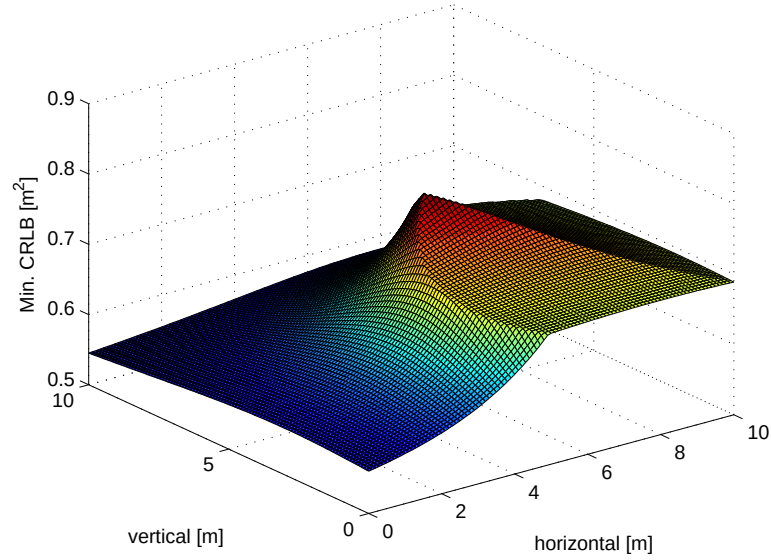
Figure 7.2: The minimum CRLB of the target nodes versus the location of the jammer node for the network given in Fig. 7.1-(a).
