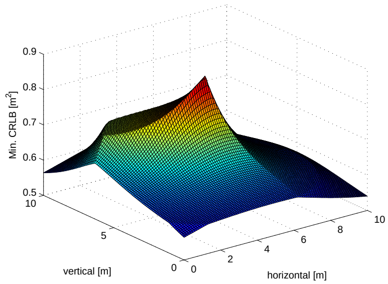
Figure 7.6: The minimum CRLB of the target nodes versus the location of the jammer node for the network presented in Fig. 7.5-(a).
