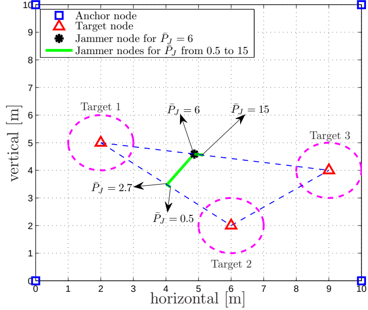
Figure 6.1: The network consisting of anchor nodes at [0\ 0] , [10\ 0] , [0\ 10] , and [10\ 10] m., and target nodes at [2\ 5] , [6\ 2] , and [9\ 4] m.
