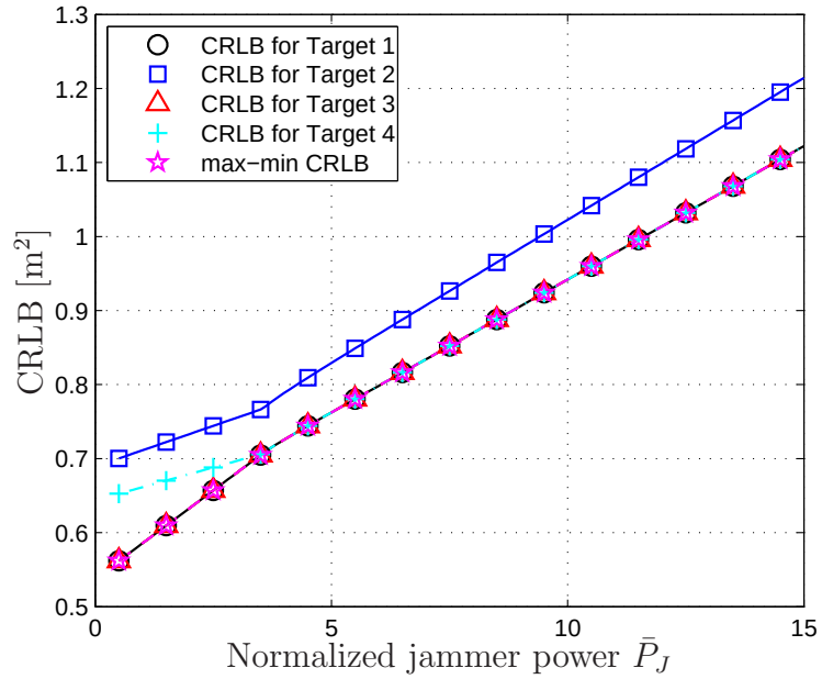
Figure 6.5: CRLB corresponding to each target node and max-min CRLB for the whole network for the scenario in Fig. 6.3.
