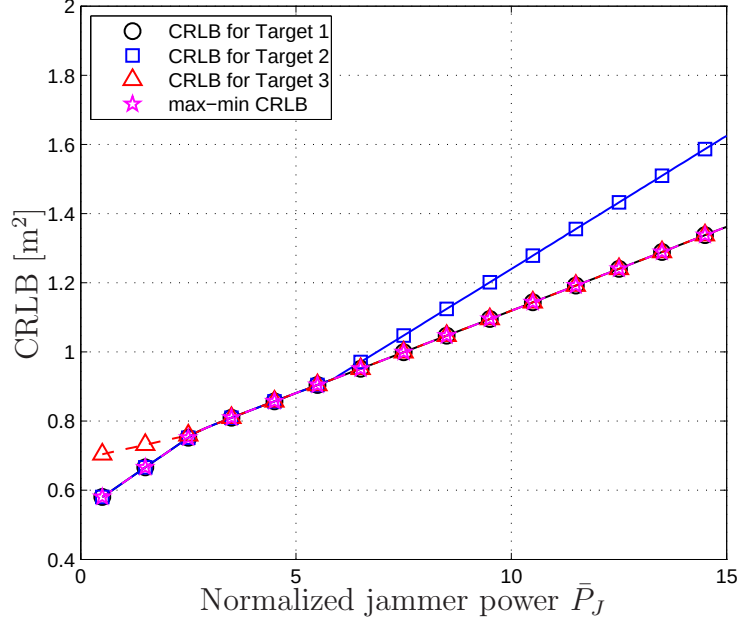
Figure 6.2: CRLB corresponding to each target node and max-min CRLB for the whole network for the scenario in Fig. 6.1.
