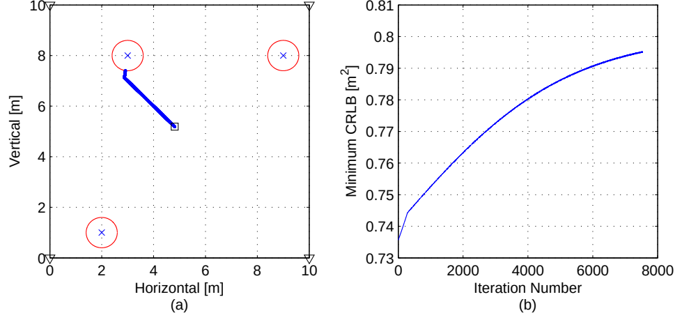
Figure 7.1: An illustration of the algorithm for a network in which the target nodes are at [2 1], [3 8], and [9 8] m. (a) The network and the jammer path. (b) The minimum CRLB in the system during the iterations of the algorithm.
