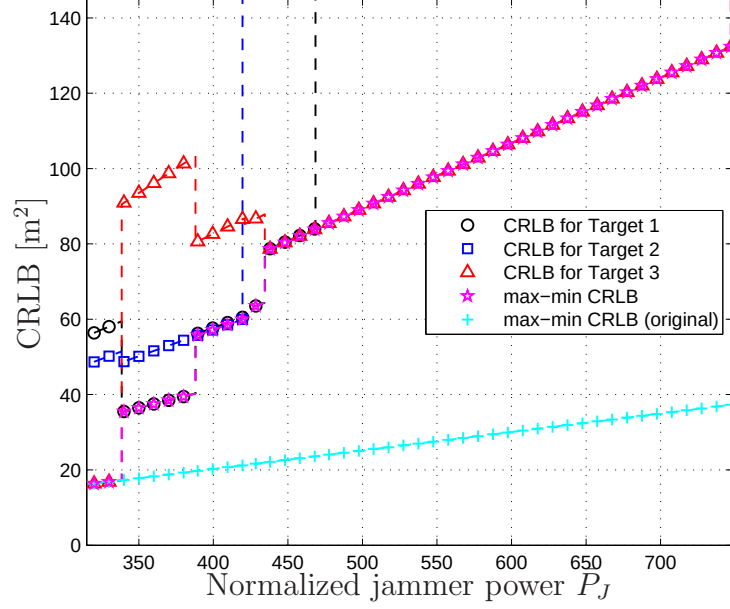
Figure 6.10: CRLB of each target node and the max-min CRLB of the network for the scenario in Fig. 6.1, where the optimal locations for the jammer node are obtained based on the CRLB expression in (5.3) and (5.4). The max-min CRLB corresponding to the optimal locations based on the CRLB expression in (4.3) and (4.4) is also shown ('original').
