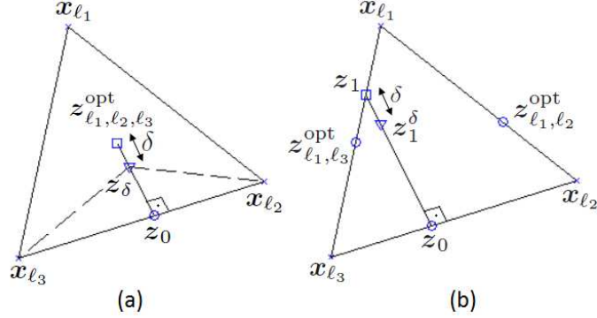
Figure A.2: (a) Illustration for the proof of Proposition 5. (b) Illustration for the proof of Proposition 6.
