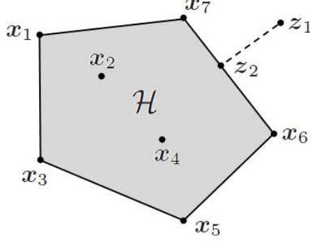
Figure 4.1: A scenario with N_T = 7 target nodes, where \mathcal{H} denotes the convex hull formed by the locations of the target nodes (the gray area). Point \mathbf{z}_2 is the projection of \mathbf{z}_1 onto \mathcal{H} .
