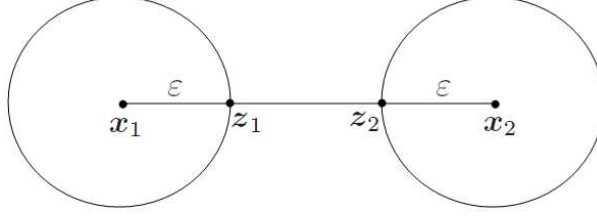
Figure A.1: Illustration of the scenario in Part (ii) of Proposition 3.
