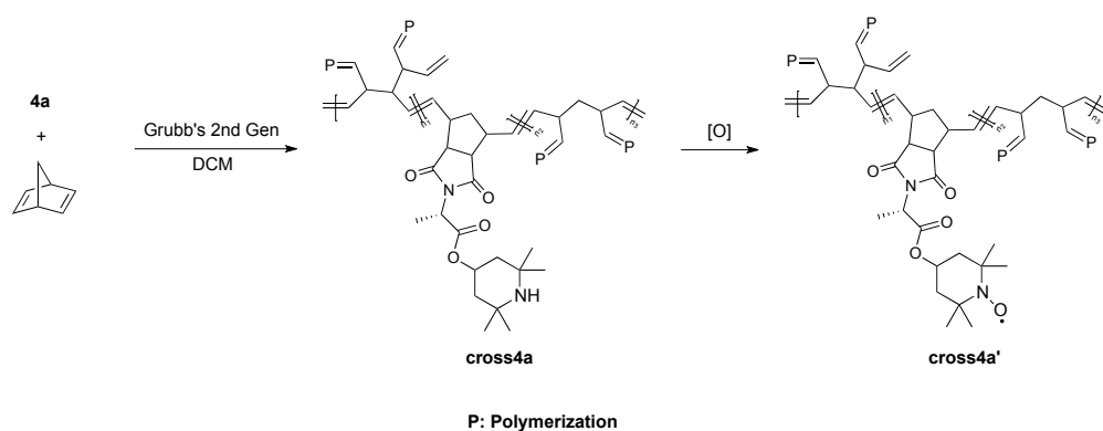
Scheme 32. Synthesis of crosslinked polymer, cross4a
