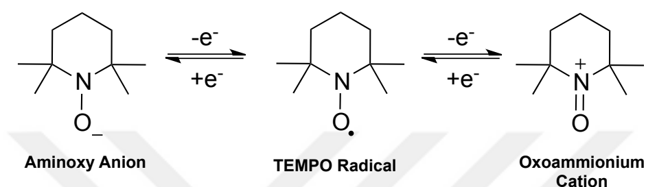
Scheme 14. The two redox couples of TEMPO radical
