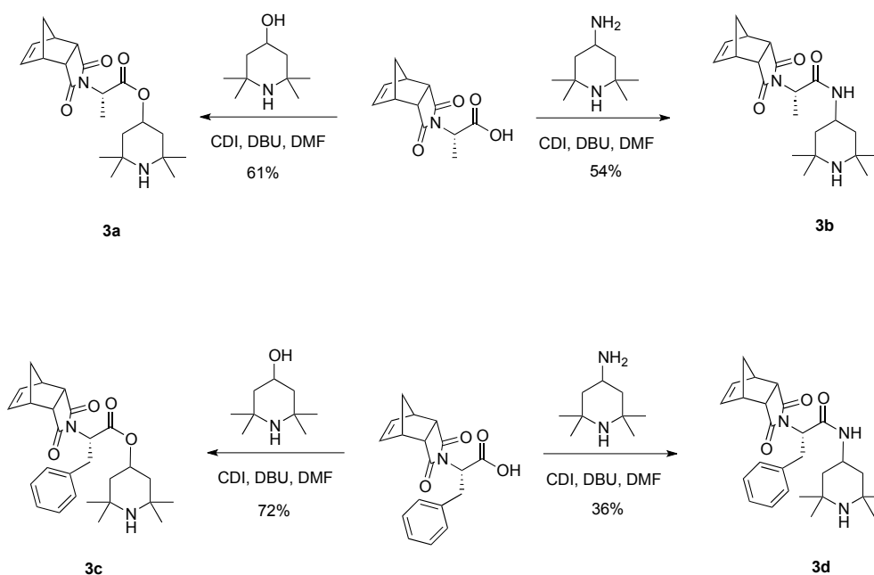
Scheme 26. Esterification and amidation of carboxylic acids
