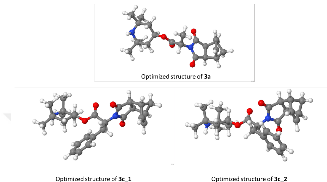
Figure 12. 3D structures of compound 3a and 3c
