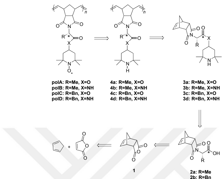
Scheme 20. Retrosynthetic analysis of the synthesized polymers
