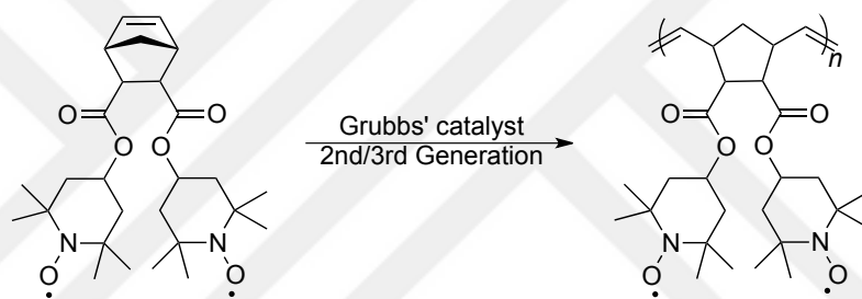
Scheme 18. Synthesis of PTNB through ROMP
