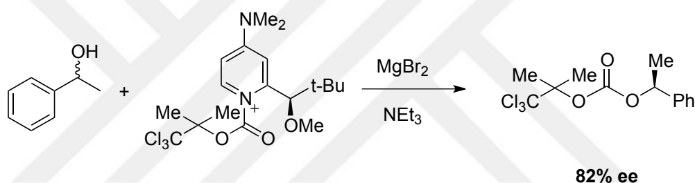
Scheme 6. Kinetic resolution using a DMAP derived salt
