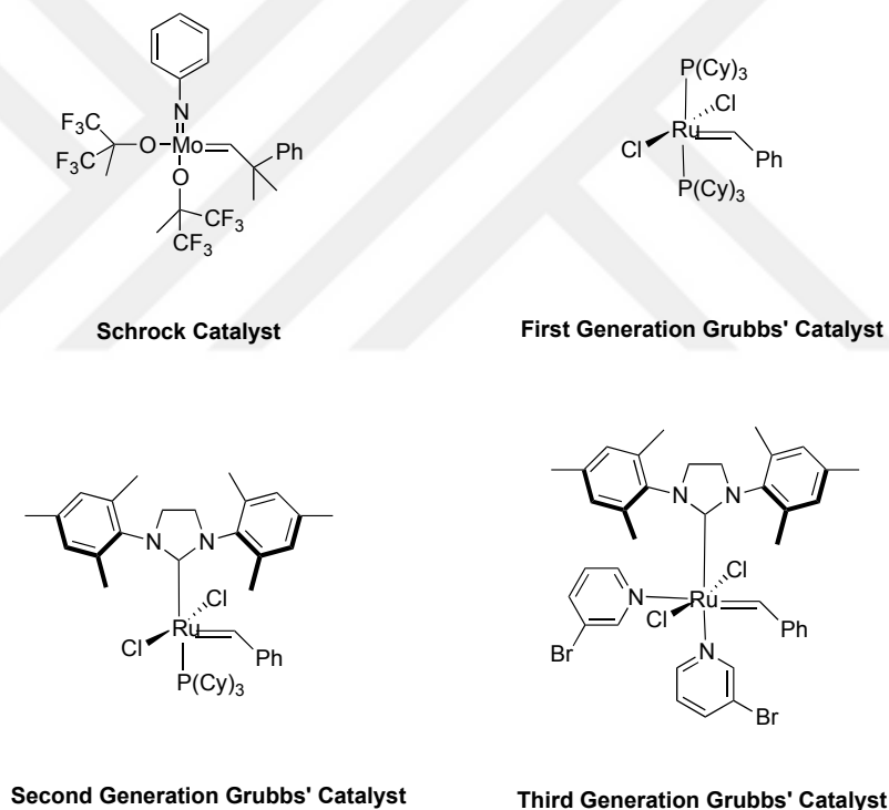
Figure 6. Examples of catalysts used for ROMP
