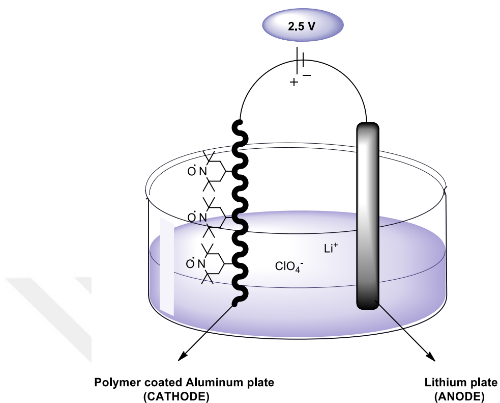
Figure 15. Schematic representation of the assembled cell
