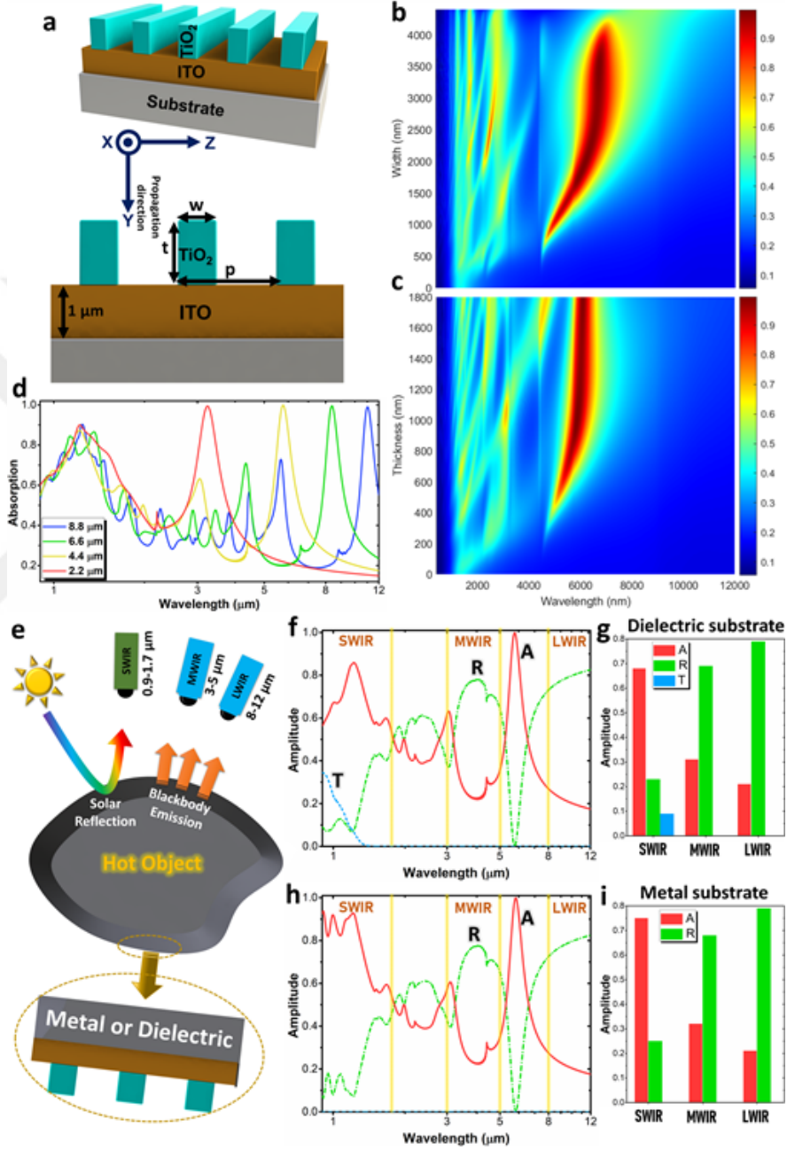
Figure 3.1: (a) Schematic illustration of the nanoantenna design and the absorption contour plots for different (b) w and (c) t . (d) The dependence of the absorption profile to design periodicity. (e) Different detection scenarios of an object. The profiles and their average SWIR, MWIR, and LWIR absorption/reflection/transmission data of the nanoantenna on different substrates of (f)-(g) dielectric and (h)-(i) metal.
