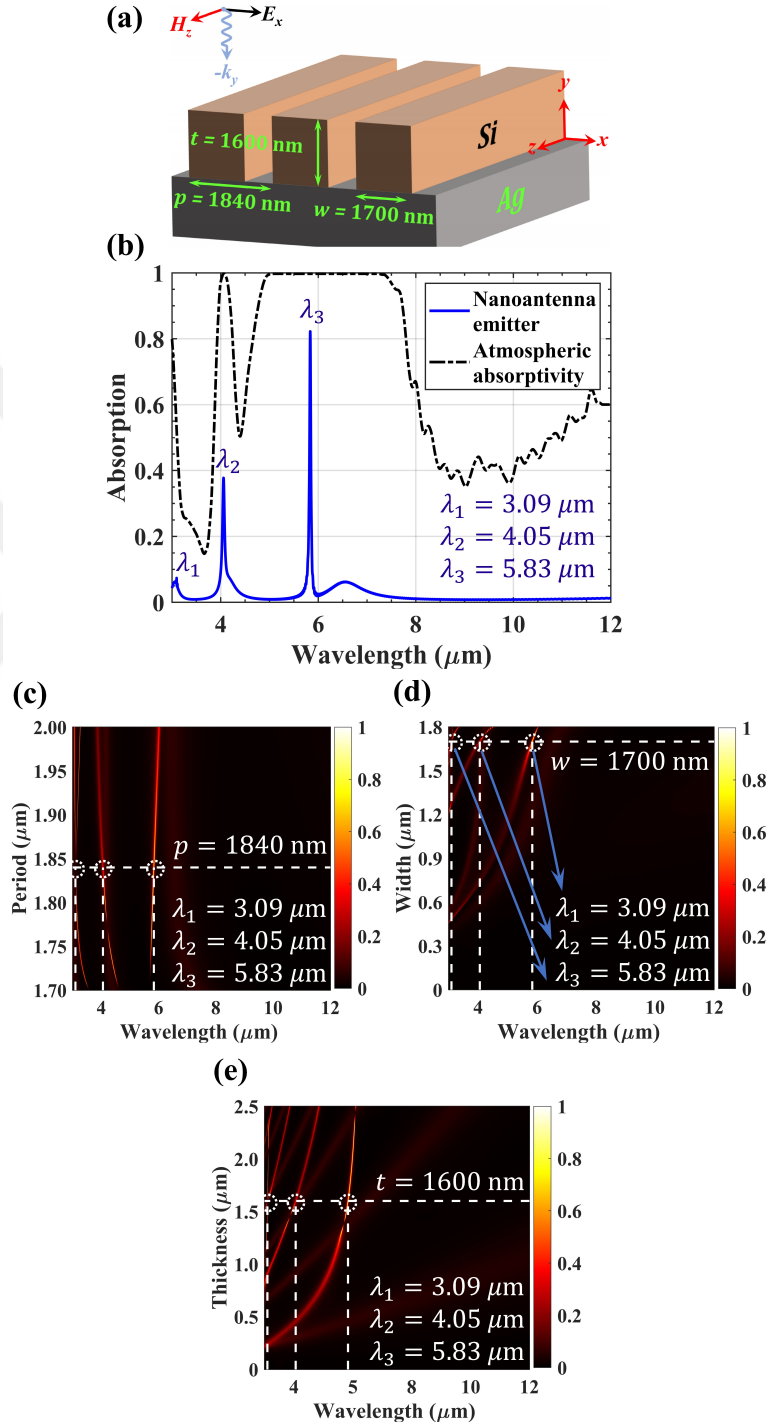
Figure 4.1: (a) Schematic representation and (b) absorption spectra of the proposed nanoantenna emitter. Impact of the nanograting dimensions including (c) the period, (d) width and (e) thickness on the absorption spectra while each parameter of the structure is kept at its optimized value besides the variation of the target parameter.
