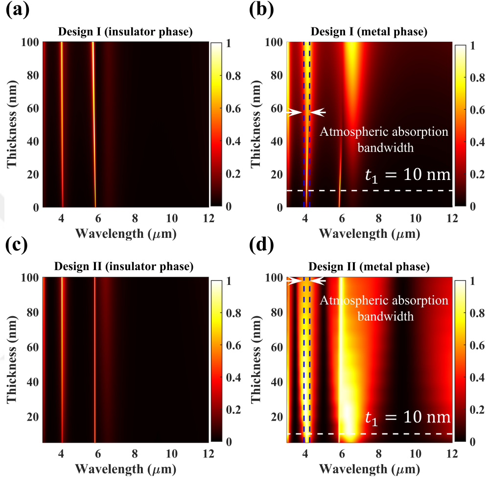
Figure 4.3: Impact of the \text{VO}_2 thickness on the absorption spectrum of design I at (a) the insulator phase, (b) the metallic phase, and on the absorption spectrum of design II at (c) the insulator phase, (d) the metallic phase.
