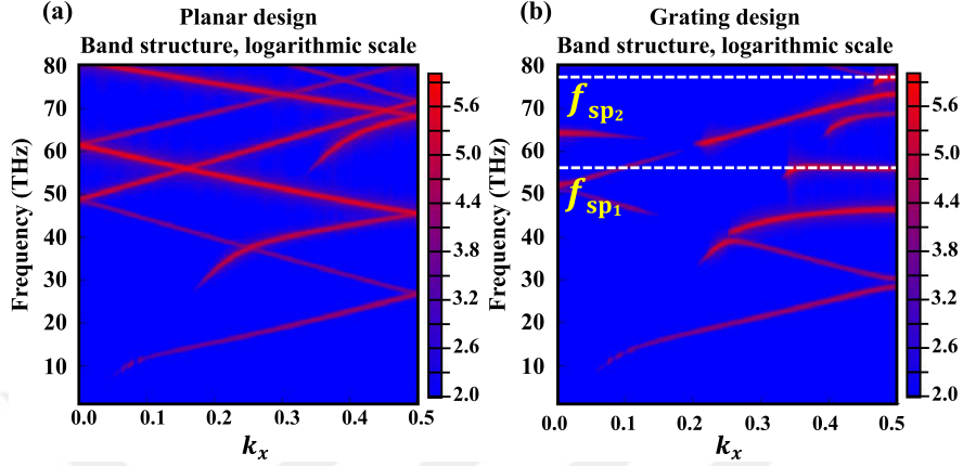
Figure 4.5: Dispersion diagram of the (a) Ag-Si planar structure and the (b) Ag-Si nanograting structure with the dimensions given in Fig. 4.1(a).
