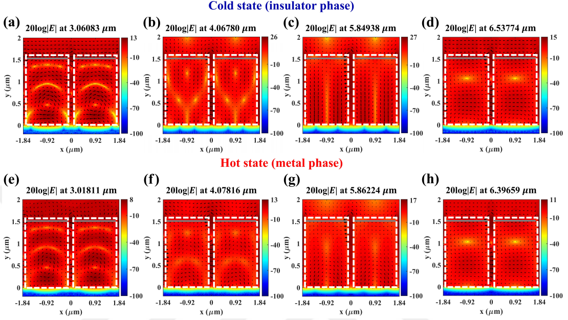
Figure 4.4: On resonance electric-field distributions across the proposed PCM-dielectric based metamaterial nanoantenna emitter (design II) on the x - y plane for (a)–(d) the cold and (e)–(h) hot states when the position of \text{VO}_2 interlayer is d_1 = 1550 nm. The color bar is shown in logarithmic scales for better comparison. The thin \text{VO}_2 interlayer is shown as the gray lines within the structure while the Si boundaries are shown as white dashed lines.
