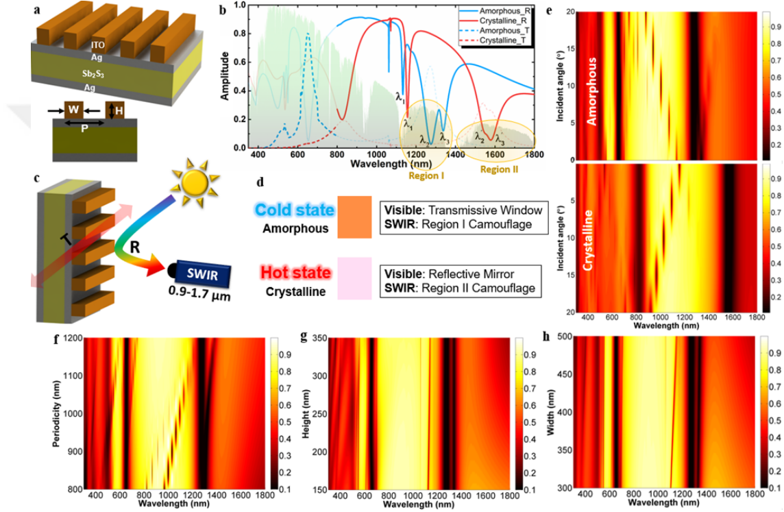
Figure 2.2: (a) Schematic representation of the proposed metasurface with its dimensions P , W , and H . (b) Reflection and transmission data of the metasurface in the amorphous and crystalline phases. The transmission data are bolded in the visible range (350–800 nm), and the reflection data are bolded in the SWIR (900–1800 nm) range. (c) Detection mechanism of the proposed metasurface using a SWIR mode thermal camera. (d) Functionality of the design in the visible and SWIR ranges. The colors shown in this panel are extracted from the Commission Internationale de l’Eclairage (CIE) color map. (e) Angular reflectance response of the metasurface in the amorphous and crystalline phases. The reflection contour plots as a function of the (f) periodicity ( P ), (g) grating height ( H ), and (h) grating width ( W ). In these plots, the other dimensions are kept in their optimal values.
