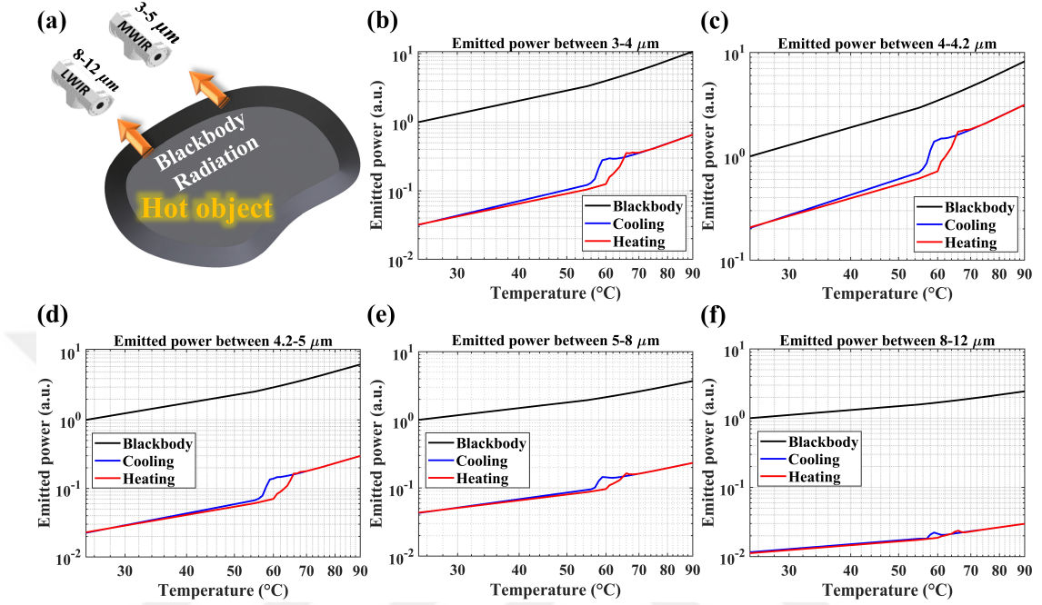
Figure 4.7: . (a) Schematic illustration of the detected optical power density using IR thermal cameras emitted from the proposed PCM-dielectric based metamaterial nanoantenna emitter. Emitted power density calculations of design I given in a logarithmic scale for different intervals including (b) 3 - 4 \mu\text{m} , (c) 4 - 4.2 \mu\text{m} , (d) 4.2 - 5 \mu\text{m} , (e) 5 - 8 \mu\text{m} , and (f) 8 - 12 \mu\text{m} .
