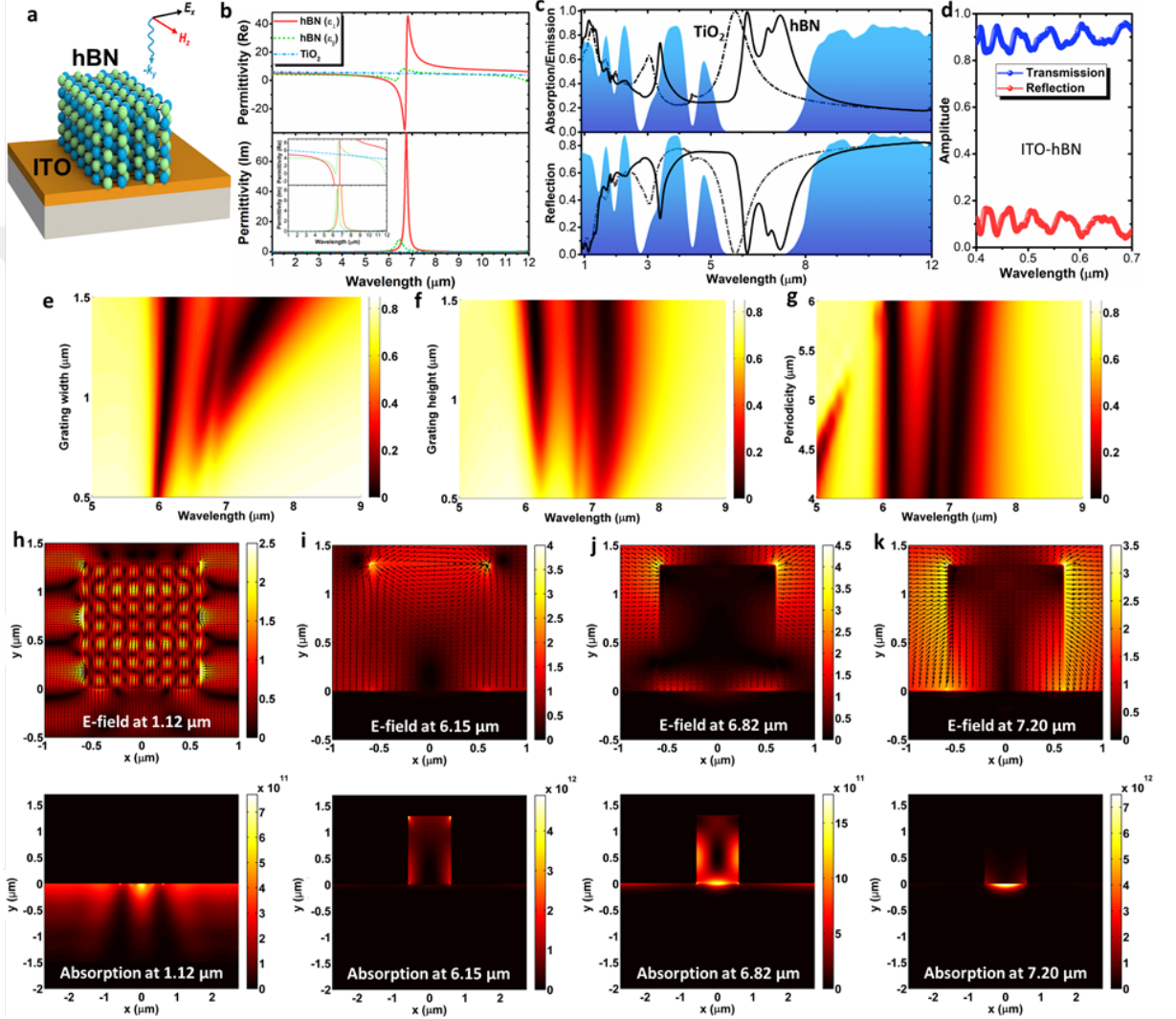
Figure 3.2: (a) Proposed hBN-ITO nanoantenna design, (b) permittivity data of hBN and TiO 2 , and (c) absorption/reflection spectra of the nanoantenna for both hBN and TiO 2 -based designs. (d) Visible light transmission and reflection of ITO-hBN. The reflection contour plots of the nanoantenna design as a function of grating (e) width, (f) height, and (g) periodicity. The E-field and absorption density profiles across the nanoantenna for different resonance wavelengths of (h) 1.12 \mu\text{m} , (i) 6.15 \mu\text{m} , (j) 6.82 \mu\text{m} , and (k) 7.2 \mu\text{m} . The color bar units for E-field and absorption density are V/m and W/m 2 .
