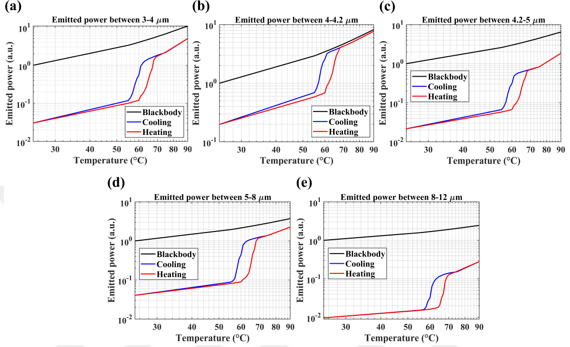
Figure 4.8: Emitted power density calculations of design II given in a logarithmic scale for different intervals including (a) 3 - 4 \mu\text{m} , (b) 4 - 4.2 \mu\text{m} , (c) 4.2 - 5 \mu\text{m} , (d) 5 - 8 \mu\text{m} , and (e) 8 - 12 \mu\text{m} .
