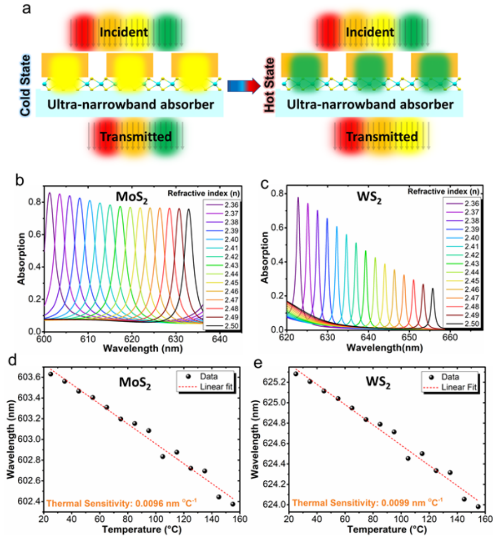
Figure 5.5: (a) Schematic illustration of red-shift of the absorption peak as the temperature is increased. Absorption calculation for varying refractive index of TiO 2 with (b) MoS 2 and (c) WS 2 in the proposed design and thermal sensitivity plots with different temperature for (d) MoS 2 and (e) WS 2
