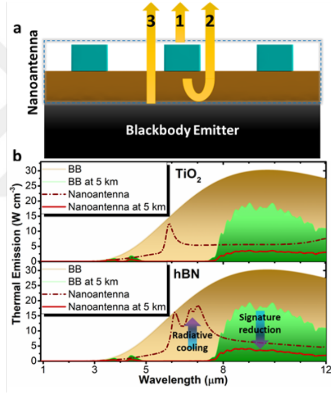
Figure 3.3: (a) Schematic illustration of thermal emission pathways from the design on top of a blackbody. (b) Thermal emission comparison of blackbody radiation at room temperature, blackbody radiation under the atmospheric transmission, metasurface design on top of BB, and the real emission from the design.
