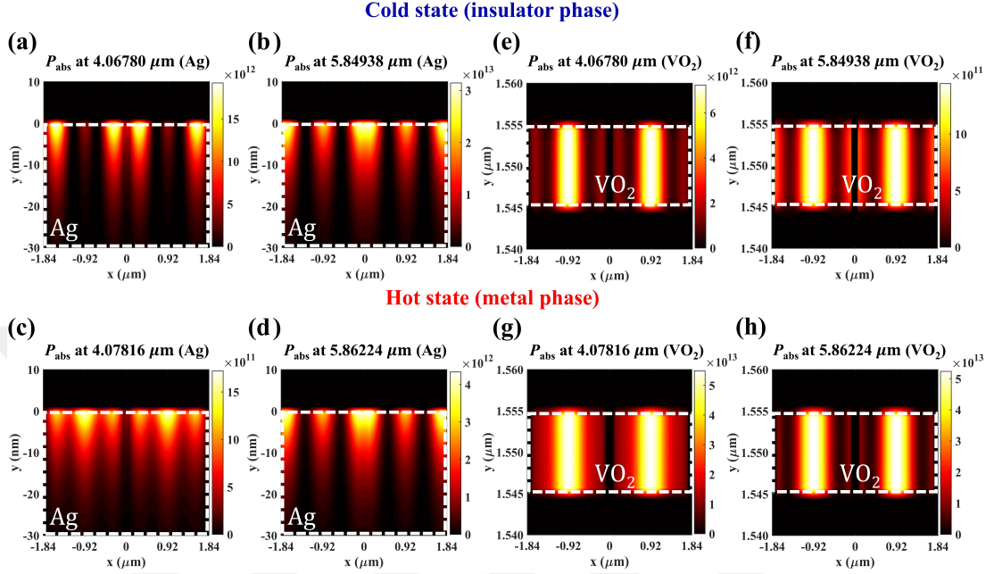
Figure 4.6: On resonance absorbed power density distributions across the Ag layer on the x - y plane considering two periodicities for (a), (b) the cold and (c), (d) hot states when the position of \text{VO}_2 interlayer is d_1 = 1550 nm. On resonance absorbed power density distributions across the \text{VO}_2 layer on the x - y plane considering two periodicities for (e), (f) the cold and (g), (h) hot states when the position of \text{VO}_2 interlayer is d_1 = 1550 nm.
