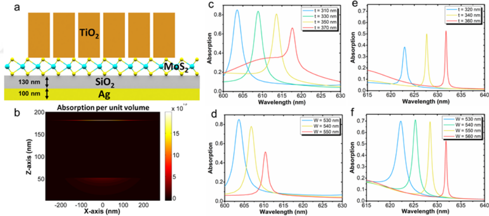
Figure 5.4: (a) Proposed optimized cavity design and (b) its absorption profile across the cavity with \text{MoS}_2 and absorption calculation for varying thickness and width of \text{TiO}_2 with \text{MoS}_2 (c-d) and (e-f) \text{WS}_2
