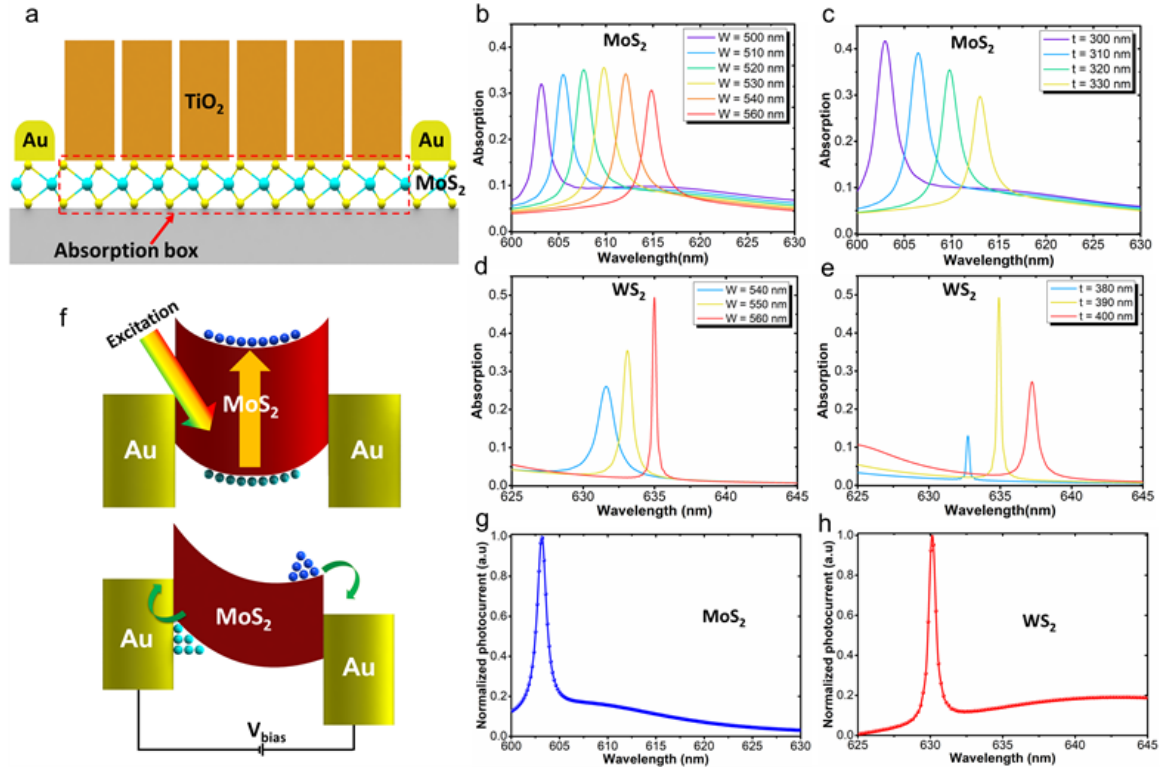
Figure 5.2: (a) Schematic representation of the all-dielectric narrow-band absorber structure, absorption calculation for varying thickness and width of \text{TiO}_2 with \text{MoS}_2 (b–c) and \text{WS}_2 (d–e). (f) The band alignment between Au and \text{MoS}_2 layer before and after applying bias. The simulated photocurrent values generated by TMD monolayers in (g) \text{MoS}_2 and (h) \text{WS}_2 cases.
