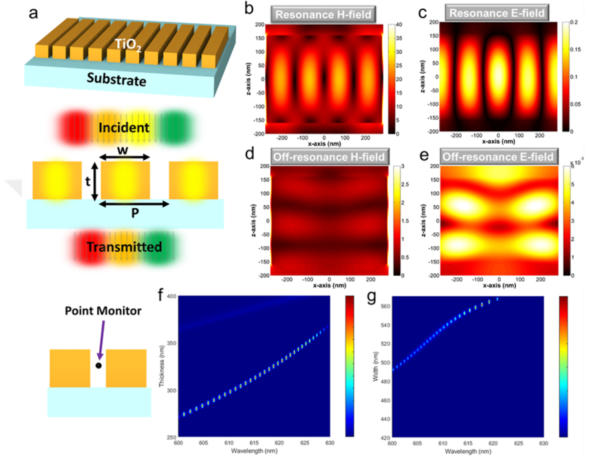
Figure 5.1: (a) Schematic representation of the proposed dielectric metasurface structure. H-field and E-field distributions across the design for (b, c) resonance frequency and (d, e) off-resonance region. Contour plots of magnetic field intensity dependence to (f) thickness and (g) width
