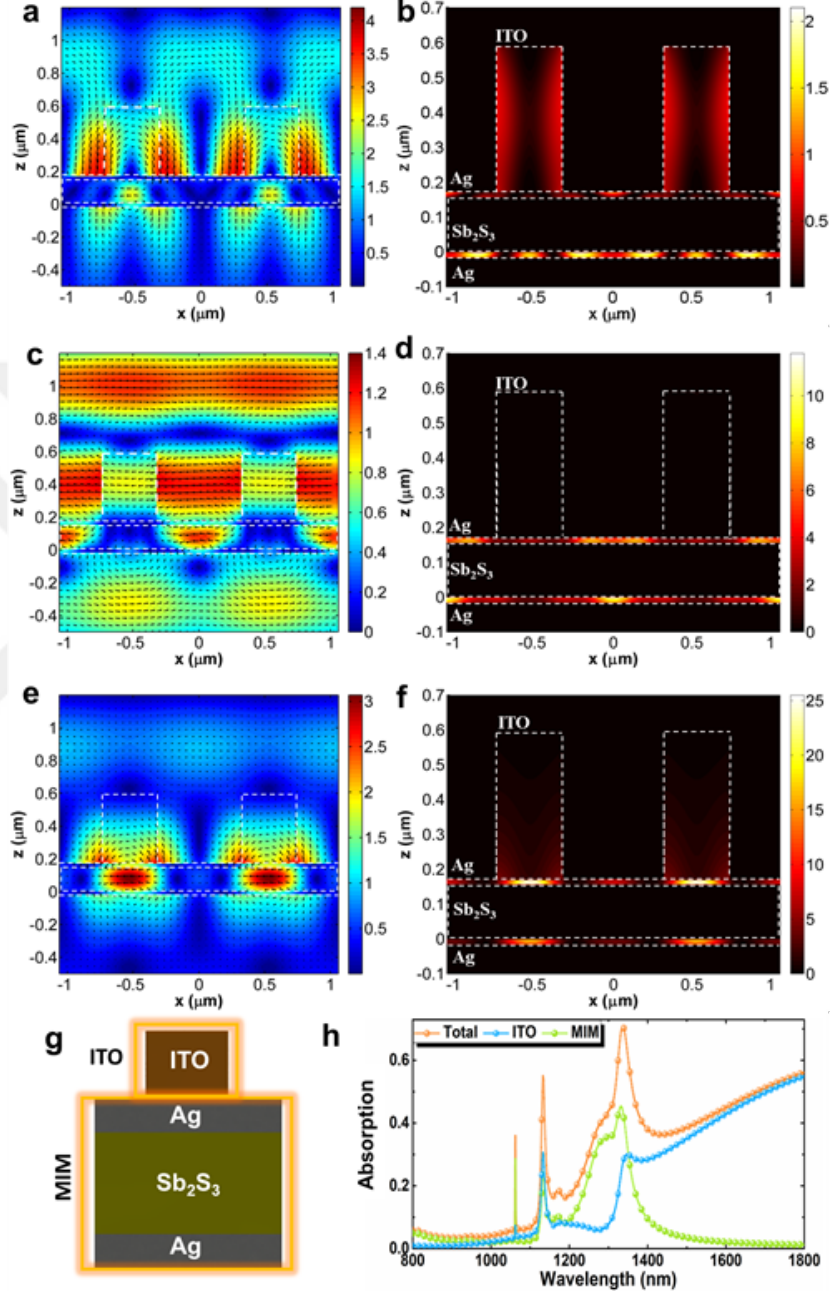
Figure 2.3: (a) E-field and (b) absorption profiles across the design in the first resonance mode of \lambda_1 = 1131 nm demonstrate the simultaneous excitation of ESPs in the metal-insulator interface and GMRs excited inside the cavity design. (c) E-field and (d) absorption profiles across the design in the first resonance mode of \lambda_2 = 1275 nm showing the transmissive FP modes excited in the MIM cavity design. (e) E-field and (f) absorption profiles across the design in the first resonance mode of \lambda_3 = 1338 nm indicates the excitation of GMRs inside the cavity. (g) Position of absorption monitors used in our analysis. (h) Absorption profiles within the ITO grating, MIM cavity, and the whole design.
