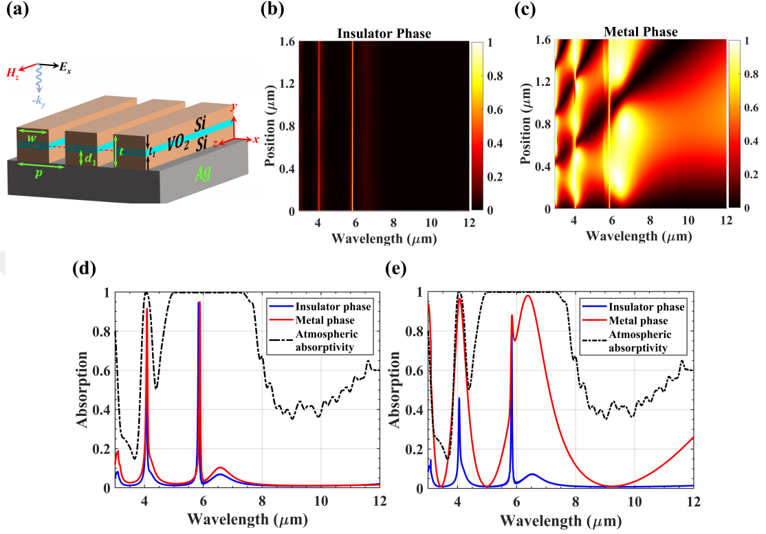
Figure 4.2: (a) Schematic representation of the PCM–dielectric based metamaterial nanoantenna emitter. The contour plots of the absorption amplitude as a function of \text{VO}_2 position for (b) insulator and (c) metal phase conditions. The absorption spectra of the structure in both the metallic and insulator phases for two different \text{VO}_2 positions at (d) d_1 = 5 \text{ nm} (design I) and (e) d_1 = 1550 \text{ nm} (design II).
