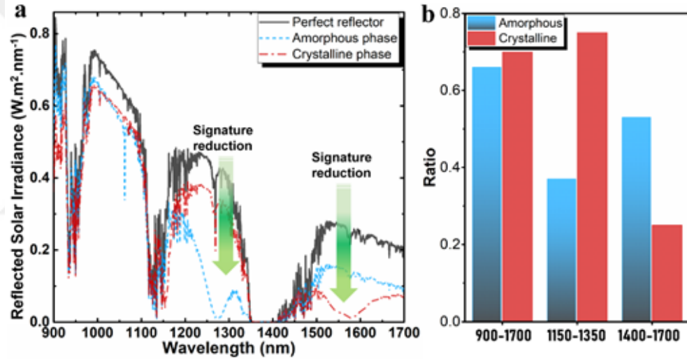
Figure 2.4: (a) Reflected solar irradiance from a metal reflector and the metasurface in the amorphous and crystalline phases. (b) Averaged power ratios in three different SWIR ranges.
