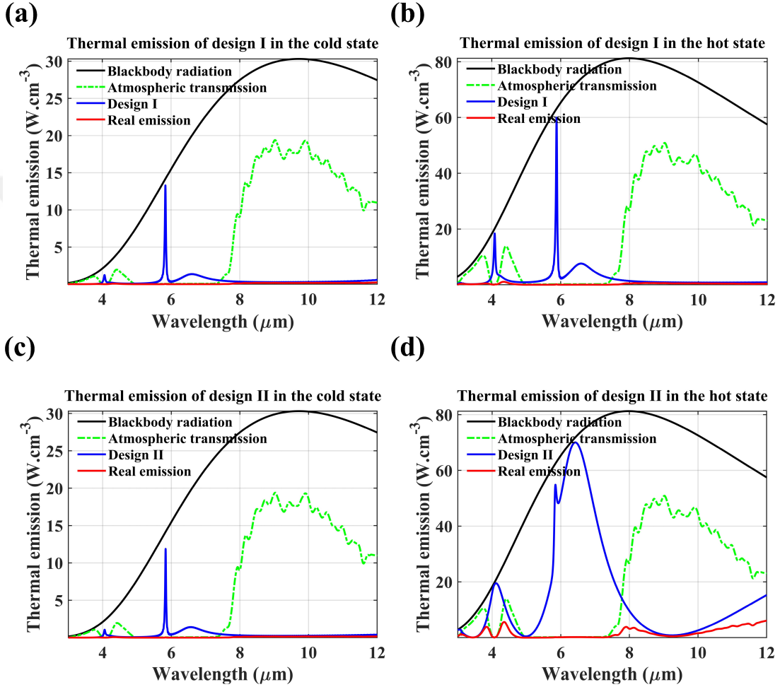
Figure 4.9: Comparisons among the emitted power densities at different temperatures including blackbody radiation (black solid line), atmospheric transmissivity for 5 km long transmission path through the atmosphere at the ground level (green dashed-dotted line) over the corresponding blackbody radiation, the proposed structure without considering atmospheric transmissivity (blue solid line) over the corresponding blackbody radiation, and the real emission response of the proposed design I and II (red solid line). The emitted power densities of the proposed narrowband design at the (a) cold state when the temperature is 25 °C and (b) hot state when the temperature is 90 °C. The emitted power densities of the proposed broadband design at the (c) cold state when the temperature is 25 °C and (d) hot state when the temperature is 90 °C.
