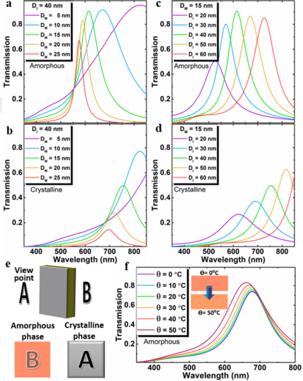
Figure 2.1: Transmission spectra of the MIM cavity for different D_M values for the (a) amorphous and (b) crystalline phases. The impact of spacer thickness ( D_I ) on the transmission spectra of the MIM cavity design for the (c) amorphous and (d) crystalline phases. (e) Schematic representation of the optical response of the MIM cavity in the visible range upon phase transition from amorphous to crystalline. (f) Angular response of the MIM cavity.
