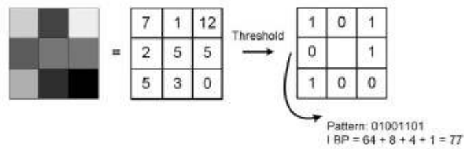
Figure: 3.4 Basic LBP Operator [24].
