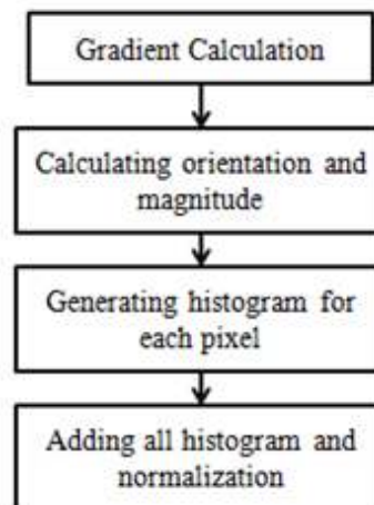
Figure 3.11 Steps of Calculating RIHOG Features.
