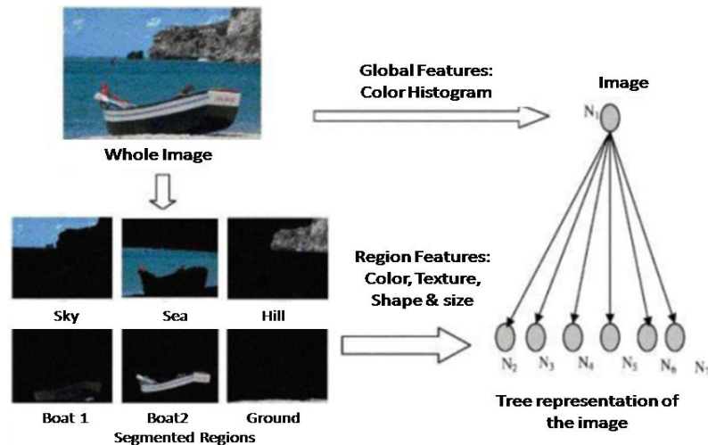
Figure 3.1: Tree Representation of Image Features [22].
