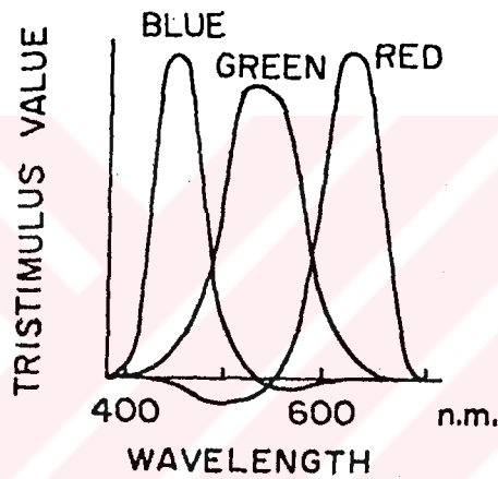
Figure 2.2: Spectral sensitivities of three types of retinal cones.
