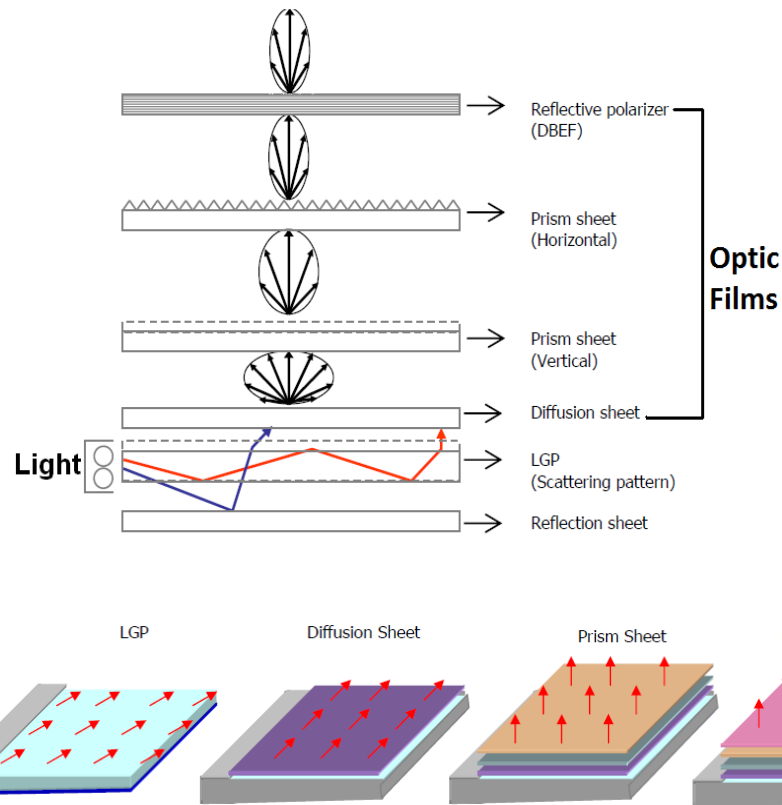
Figure 2.11 The principle of light reflection each films (in the courtesy of Vestel Electronic Inc., from the technical notes)
