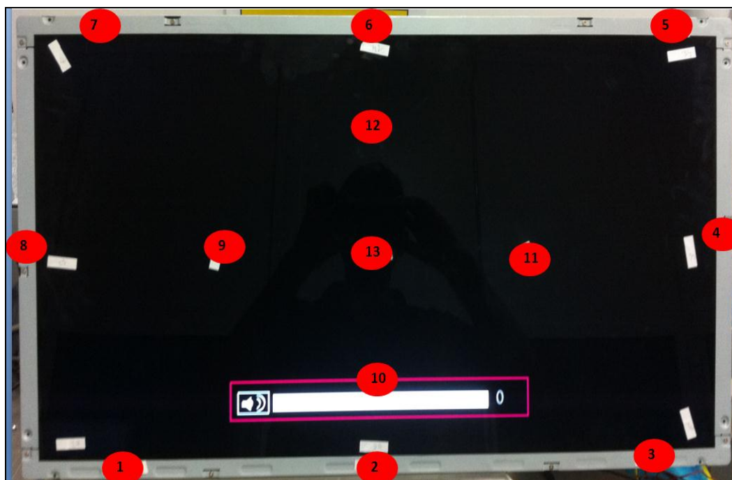
Figure 5.9 Illustration of thermocouple mounting on the TFT LCD Front Metal & CELL surface
