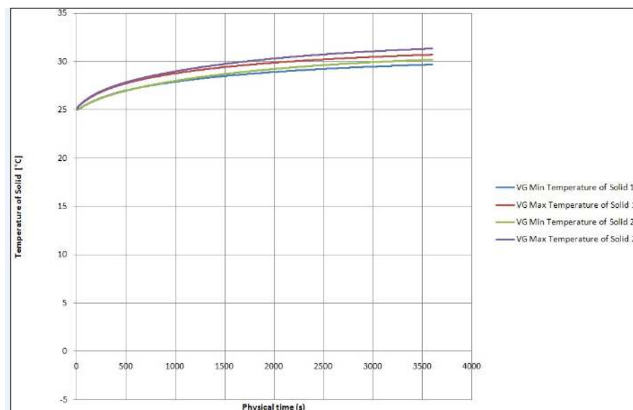
Figure 3.17 Initial result of first computer analysis LED panel
