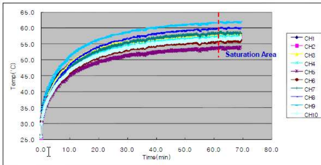
Figure 4.5 180 pcs LED panel experimental study result graph
