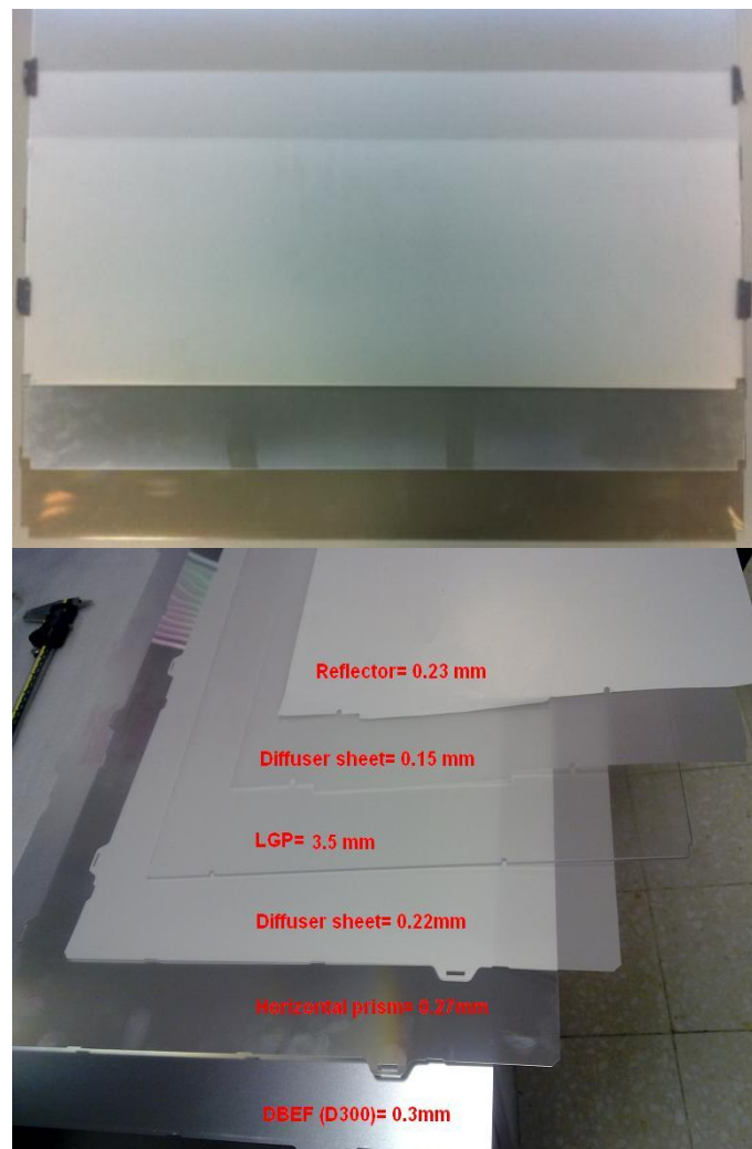
Figure 2.10 Optical film view
