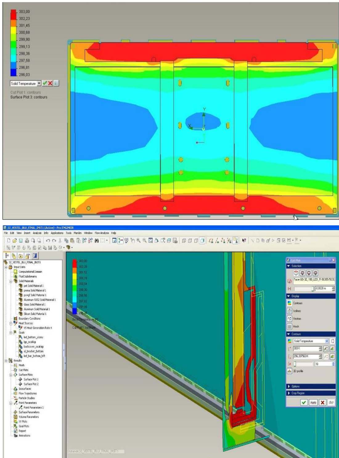
Figure 3.18 Computed temperature distributions on LED panel
