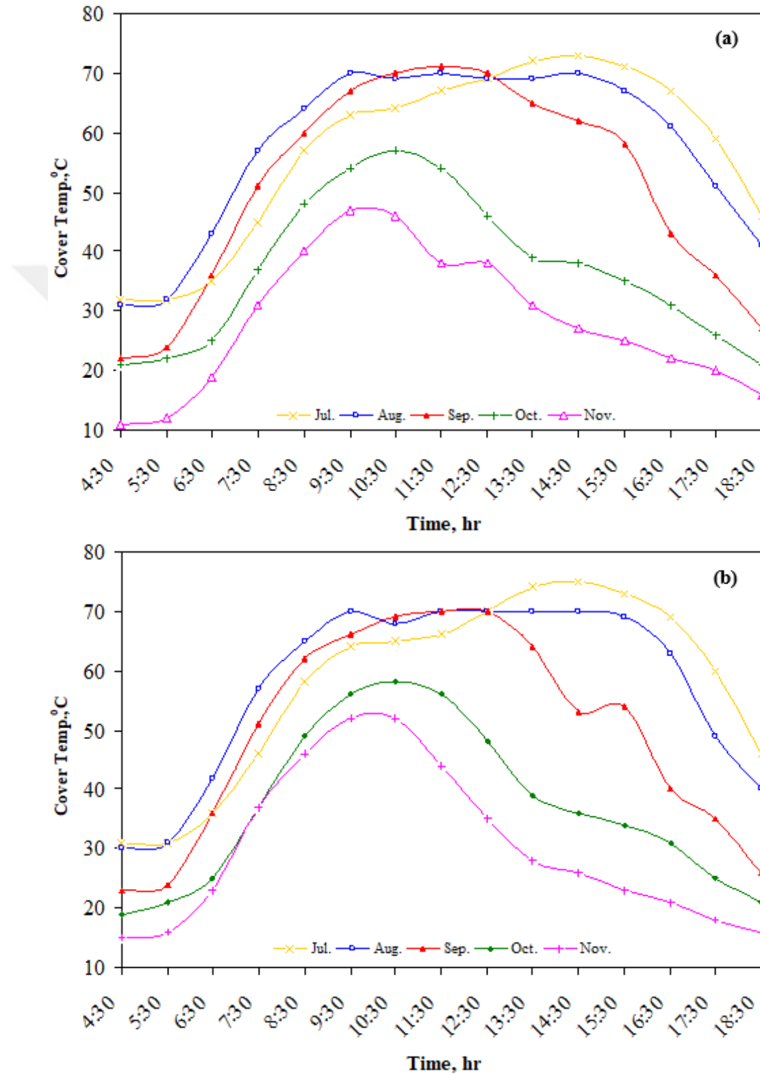
Figure 4.6. Cover temperature for (a) Silica gel, (b) Composite material
