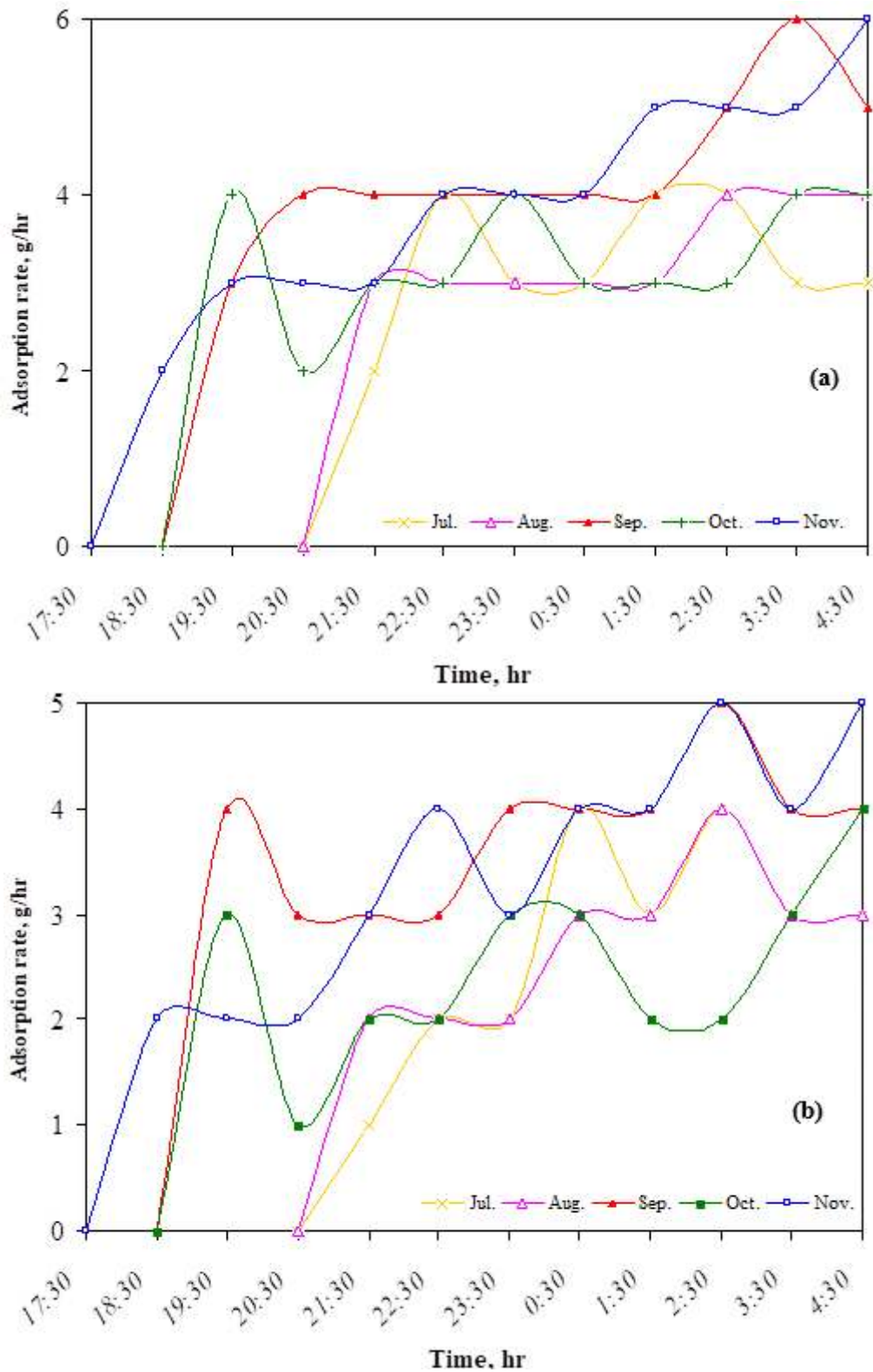
Figure 4.12. Adsorption rate for (a) Silica gel, (b) Composite material
