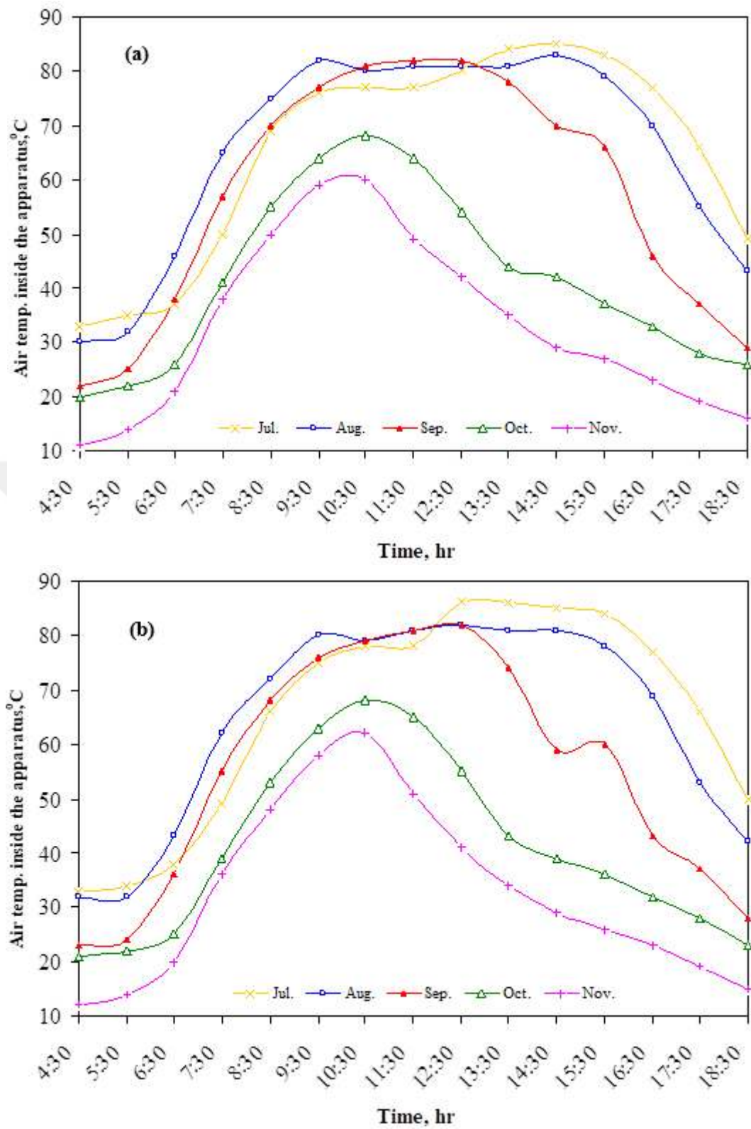
Figure 4.9. Air temperature inside the apparatus for (a) Silica gel, (b) composite material
