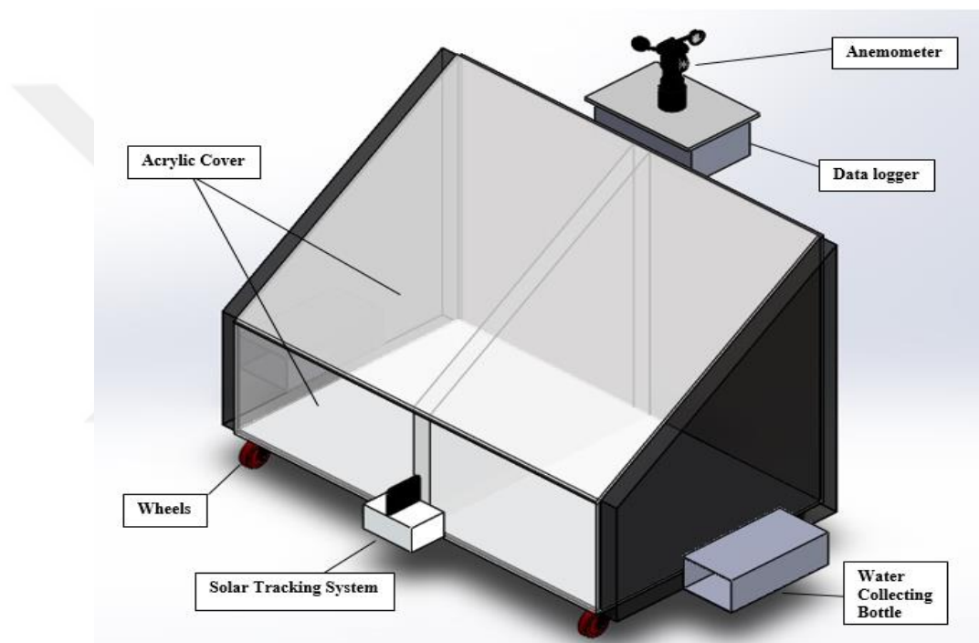
Figure 3.2. Schematic diagram of the apparatus
