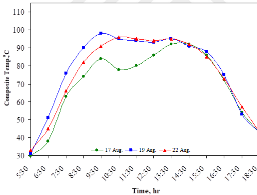
Figure H.8. Change of composite material temperature with time for various days
