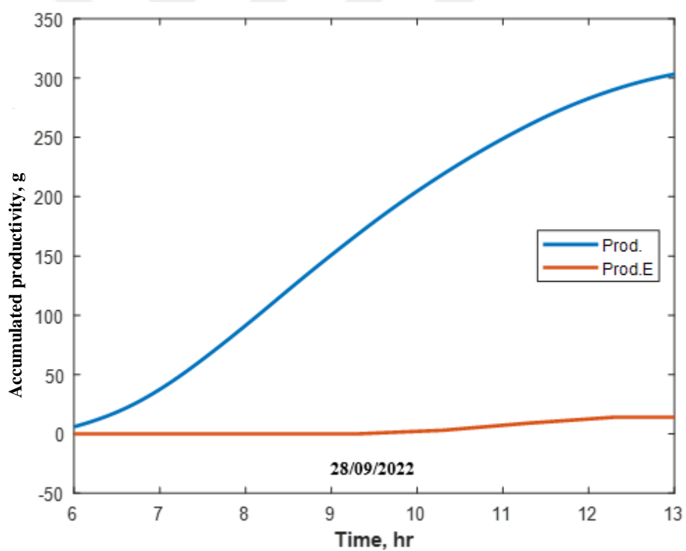
Figure I.3. Comparison between theoretical and experimentally accumulated water productivity for different days
