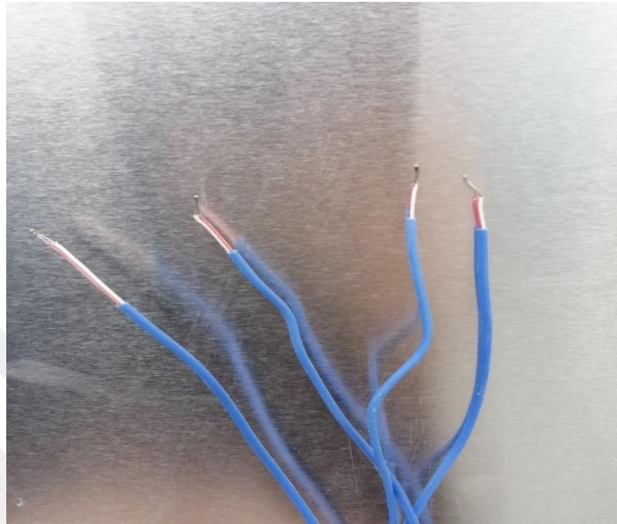
Figure 3.5. K-type thermocouple
