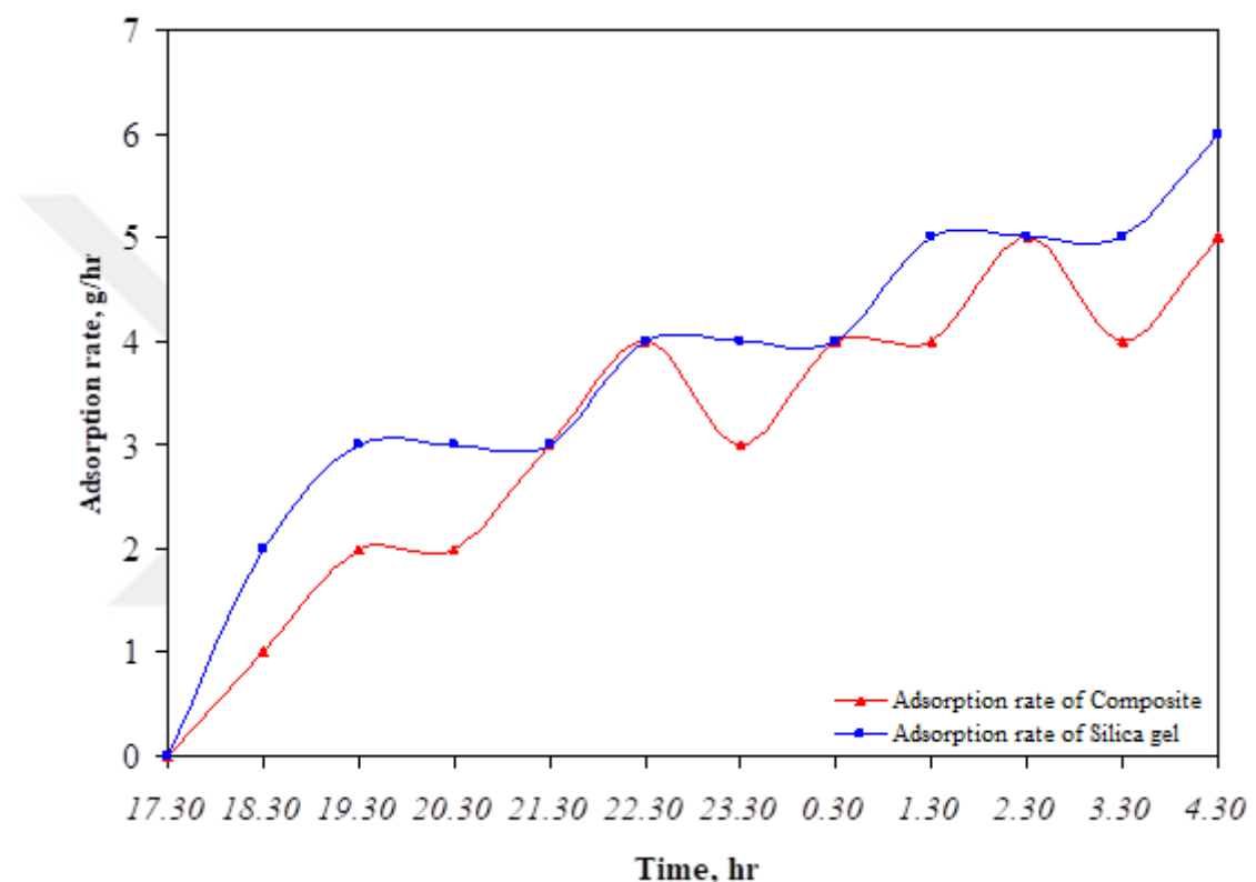
Figure 4.13. Comparison between the adsorption rates of Silica gel and composite material for November
