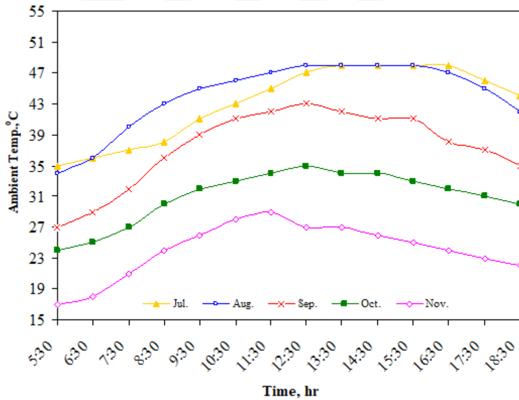
Figure 4.5. Variation of ambient temperature for various months
