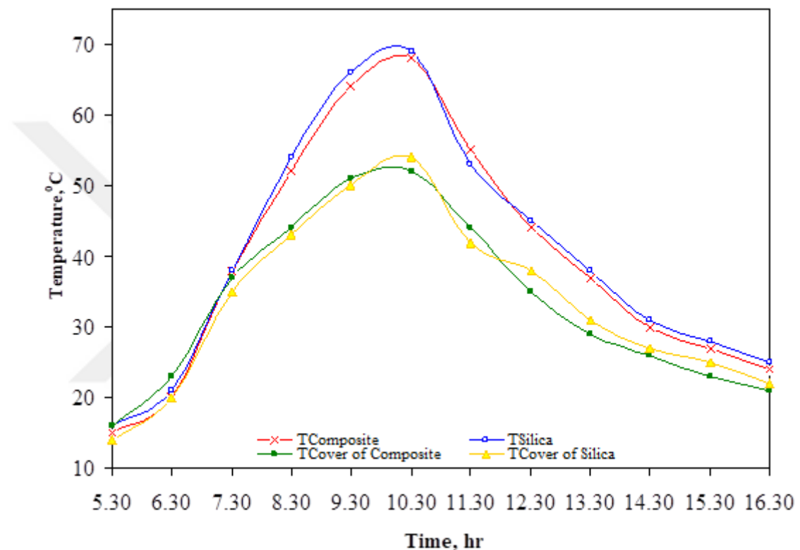
Figure 4.8. Comparison between Silica gel and composite material for desiccant and cover temperatures for November
