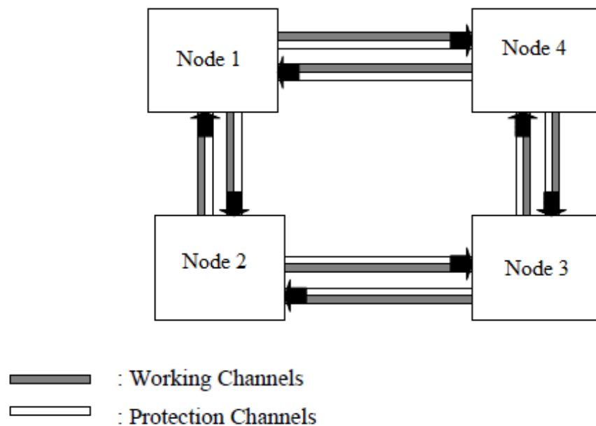
Figure 3.14 Two-fiber MS-SPRing.
