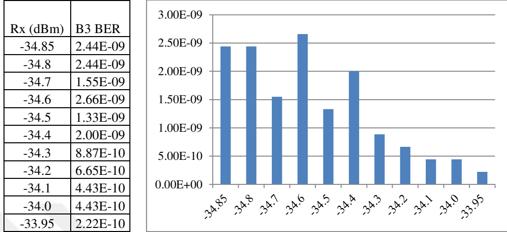
Figure 4.4 BER test results of Konak-Hatay 155 Mb/s STM1.
