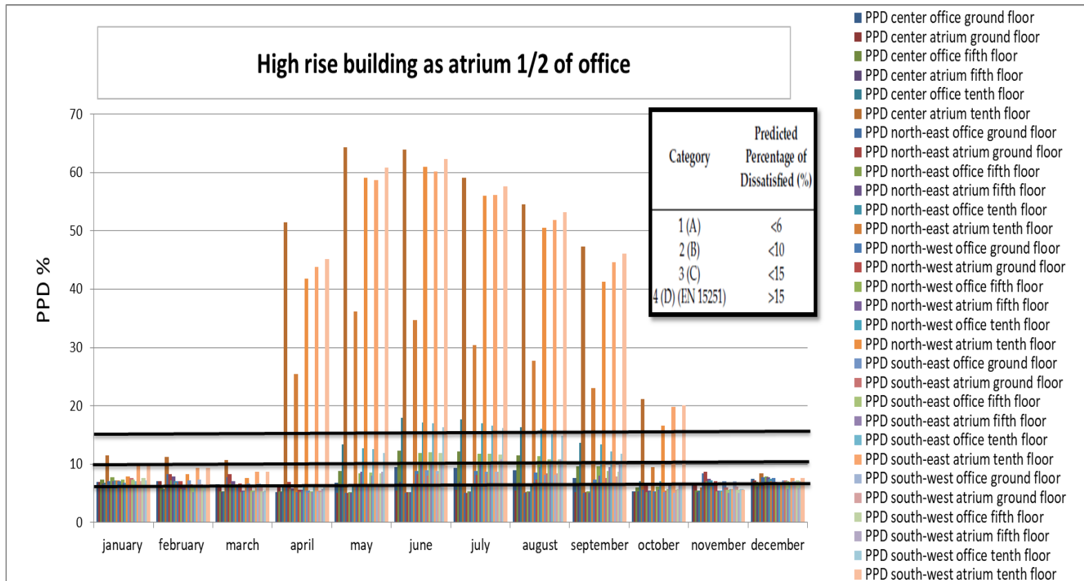
Figure 34: The PPD (predicted percentage dissatisfied) for av mechanically conditioned High-Rise building with atrium proportion 1/2 of the office space.
