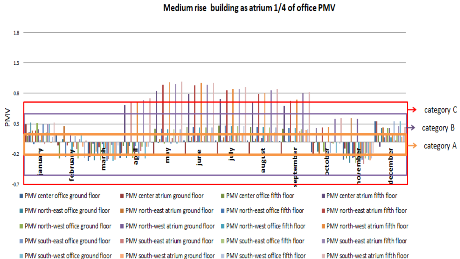
Figure 31: The PMV (predicted mean vote) for a mechanically conditioned Medium-Rise building with atrium proportion 1/4 of the office space.
