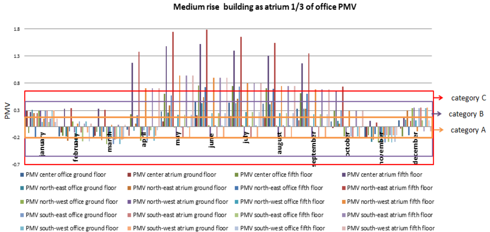
Figure 29: The PMV (predicted mean vote) for a mechanically conditioned Medium-Rise building with atrium proportion 1/3 of the office space.
