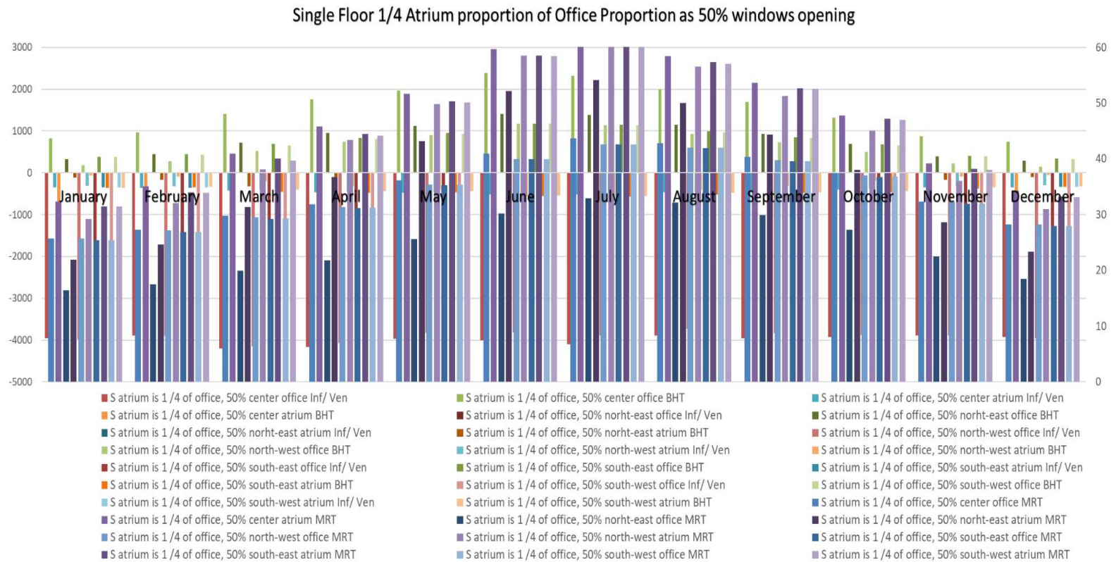
Figure 46. The Single-Floor atrium building with atrium proportion 1/4 of the office proportion and 50% opening ratio for all windows.
