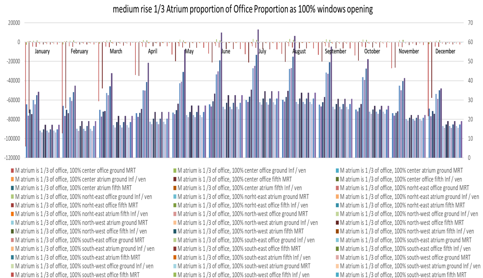
Figure 54: The Medium-Rise atrium building with atrium proportion 1/3 of the office proportion and 100% opening ratio for all windows.
