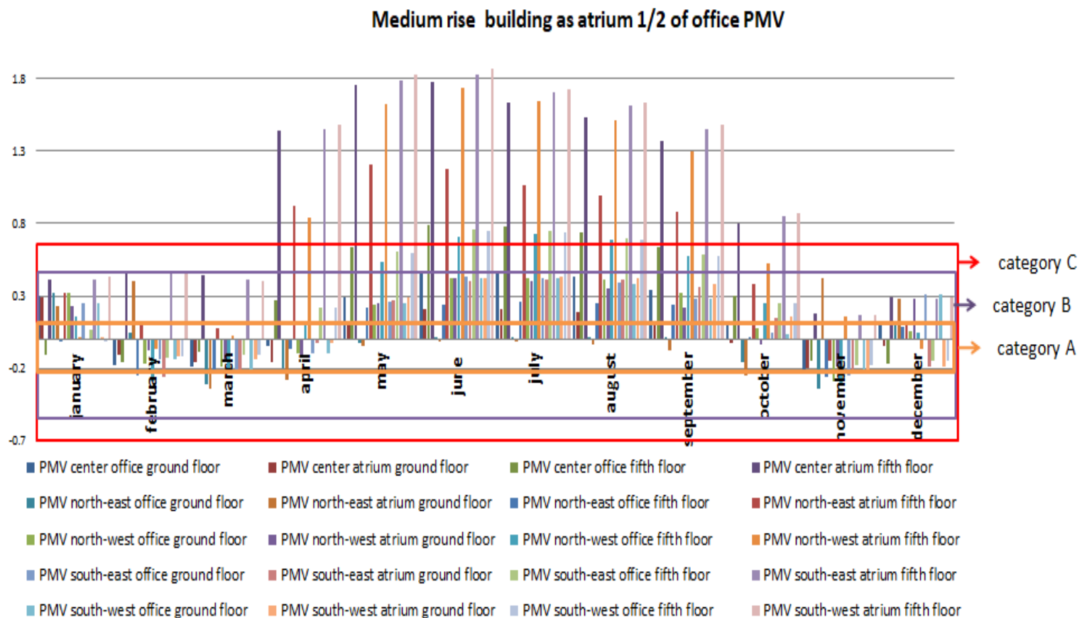
Figure 27: The PMV (predicted mean vote) for a mechanically conditioned Medium-Rise building with atrium proportion 1/2 of the office space.
