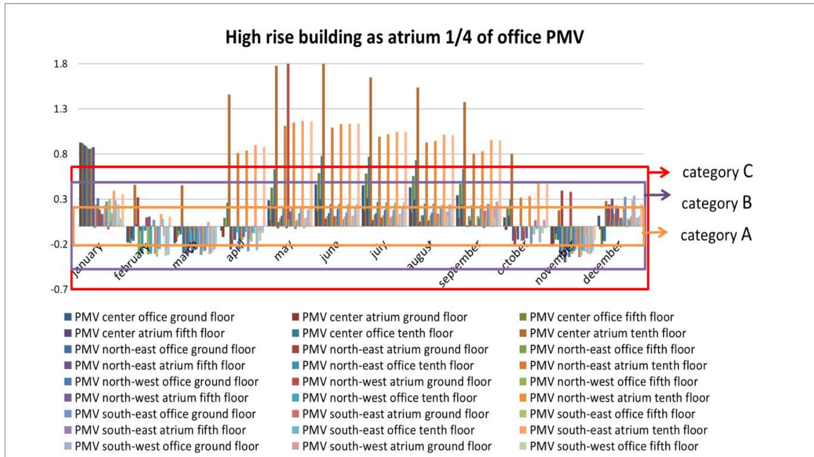
Figure 37: The PMV (predicted mean vote) for a mechanically conditioned High-Rise building with atrium proportion 1/4 of the office space.
