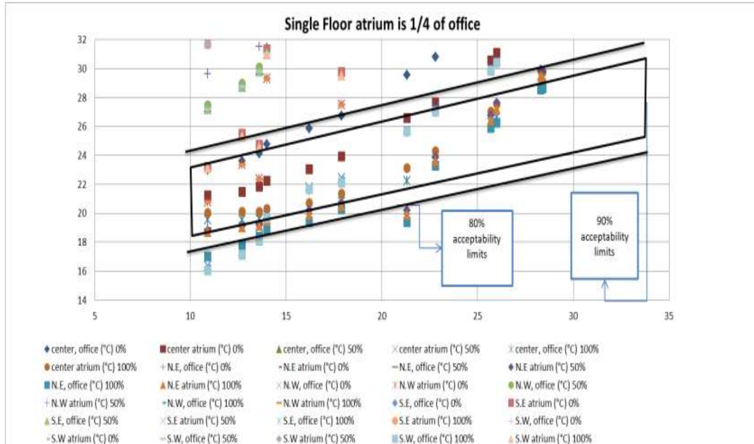
Figure 14: The adaptive model of a naturally conditioned Single-Floor building with atrium proportion 1/4 of the office space (different atrium placements and window opening ratios as 0%, 50% & 100%).
