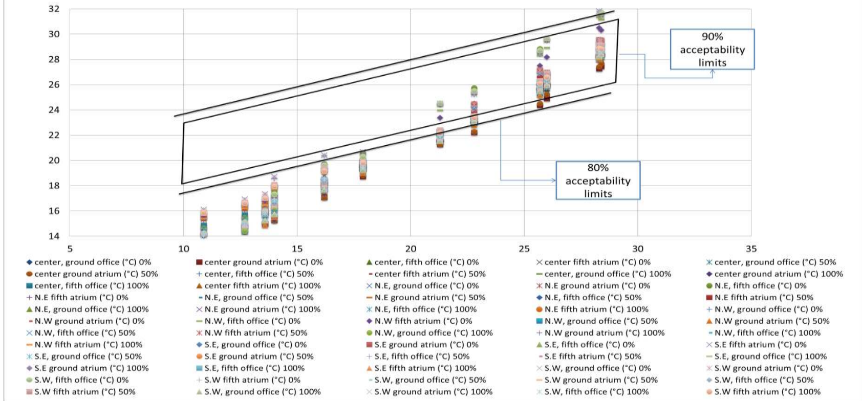
Figure 15: The adaptive model of a naturally conditioned Medium-Rise building with atrium proportion 1/2 of the office space (different atrium placements and window opening ratios as 0%, 50% & 100%).
