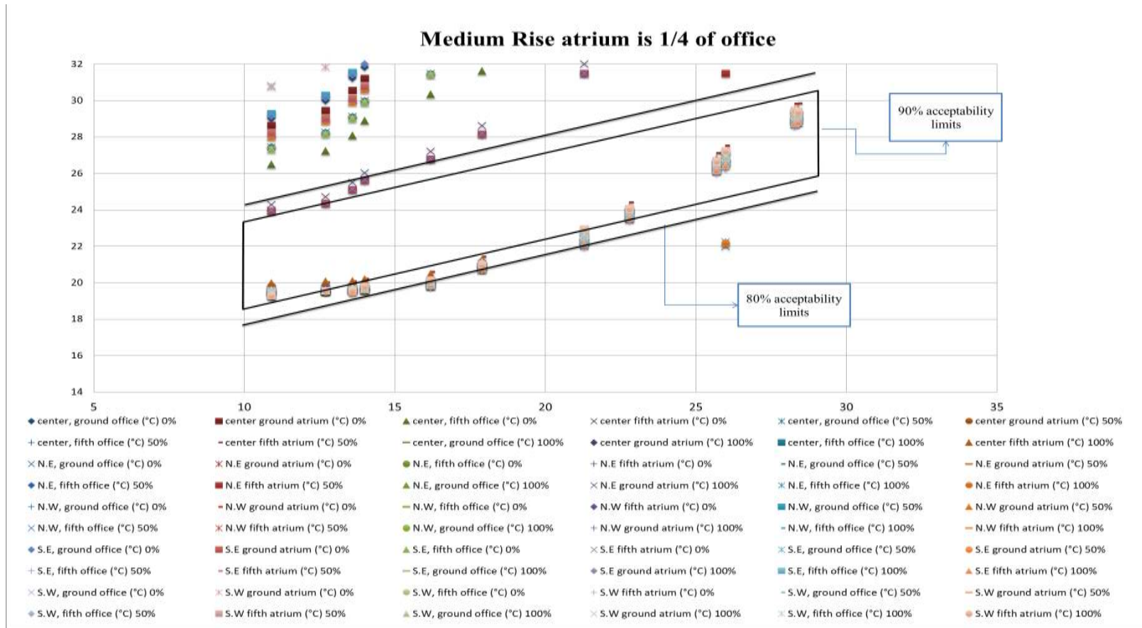
Figure 17: The adaptive model of a naturally conditioned Medium-Rise building with atrium proportion 1/4 of the office space (different atrium placements and window opening ratios as 0%, 50% & 100%).
