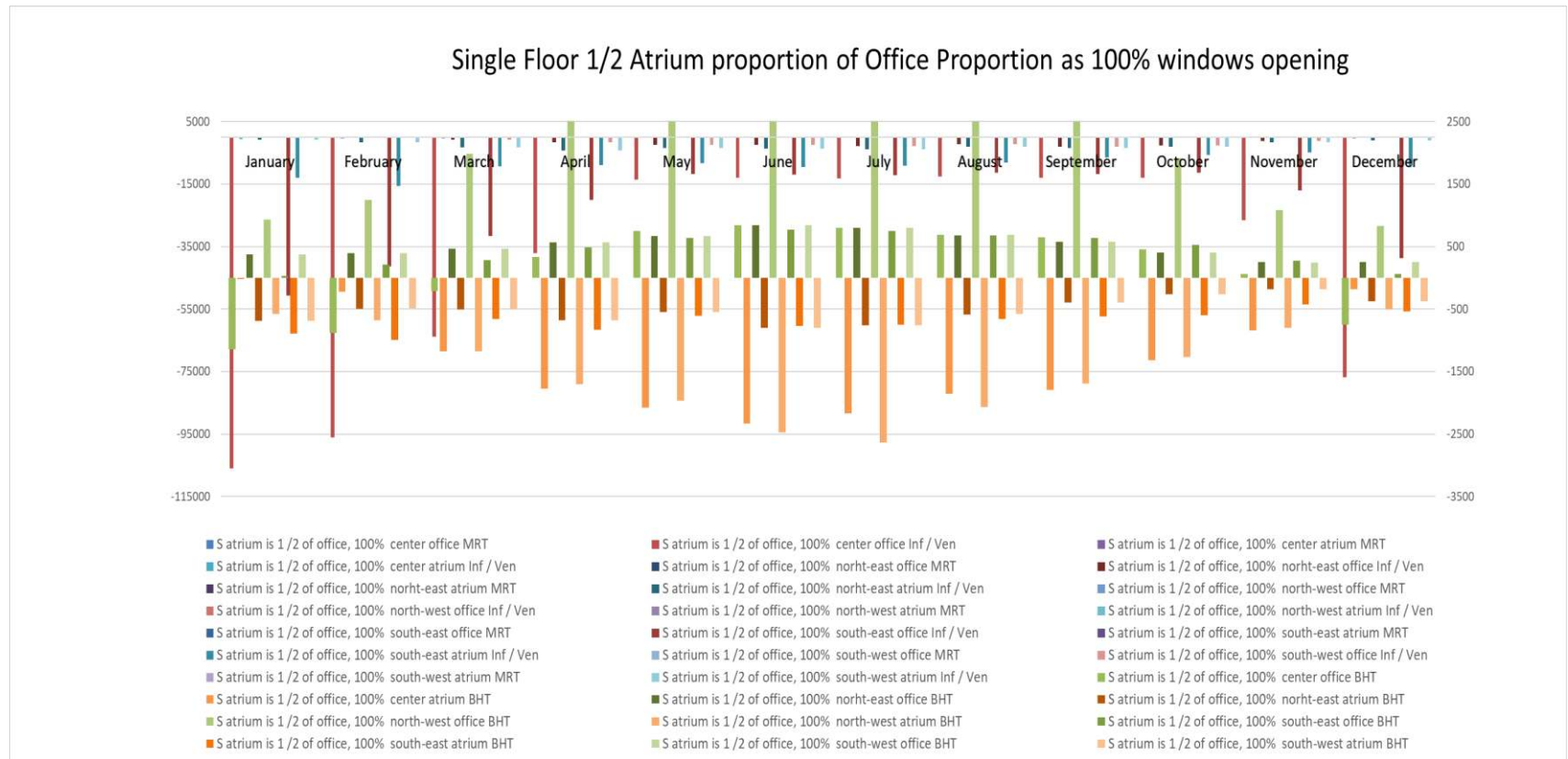
Figure 41: The Single-Floor atrium building with atrium proportion 1/2 of the office proportion and 100% opening ratio for all windows.
