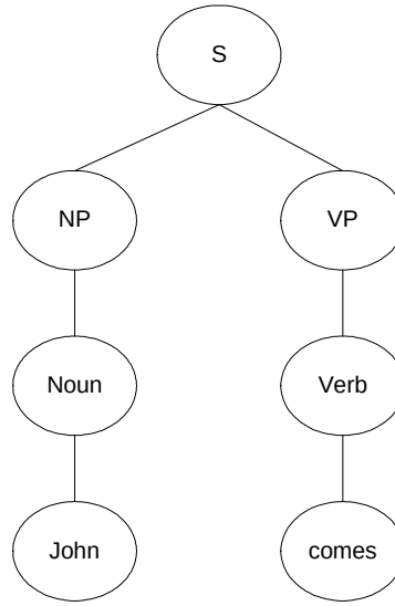
Figure 5.6: Generated Parse Tree for the sentence John comes
