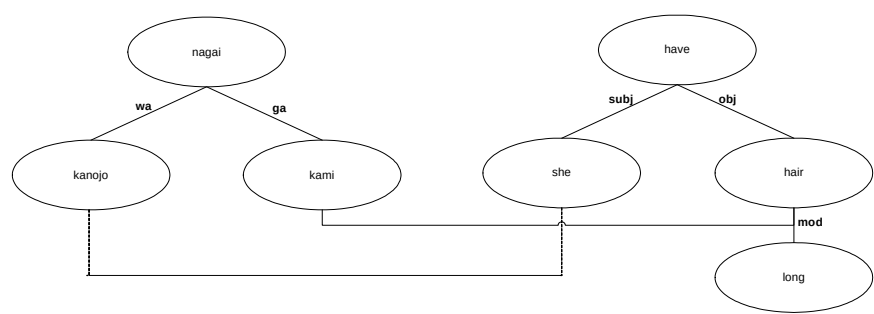
Figure 1.5: Annotated Tree Structure for she have long hair
