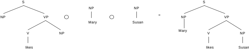
Figure 1.7: Translation of Mary likes Susan using subtrees
