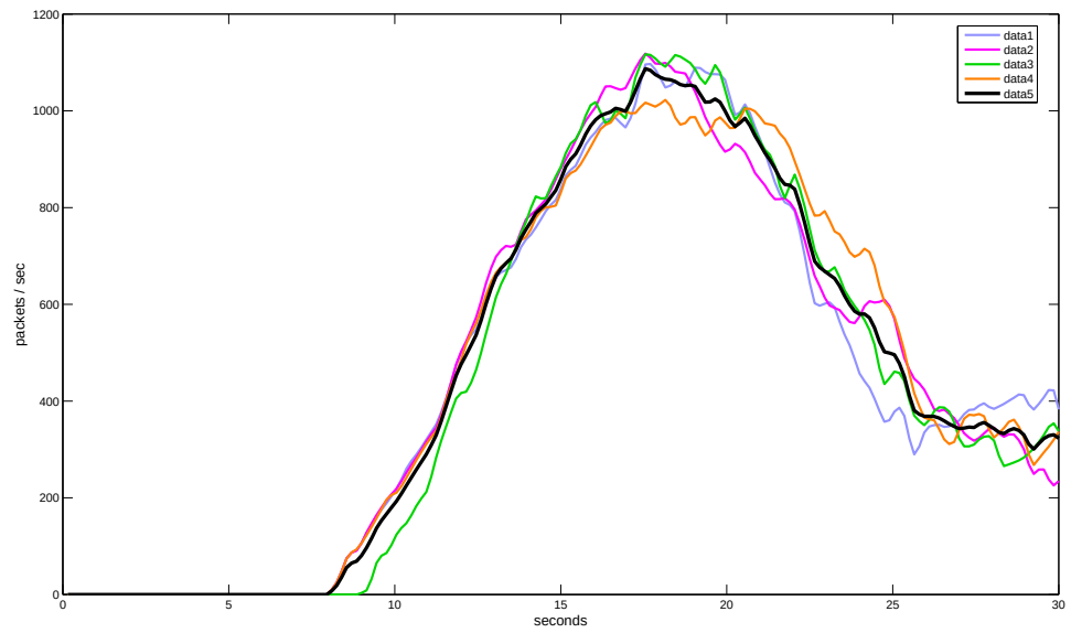
Figure 3.47: Moving average of traffic drop rates for four different simulations and the curve of average values (results for RED applied congested interface)
