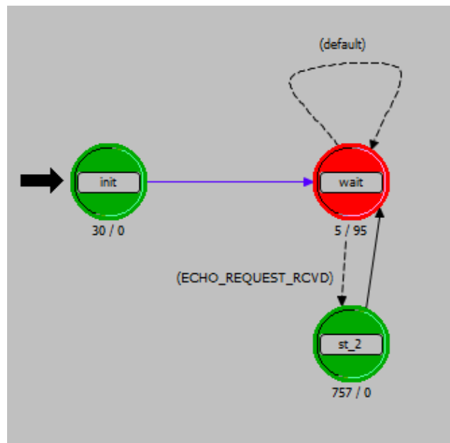
Figure 3.14: Process model for child process ‘controller_icmp.pr.m’
