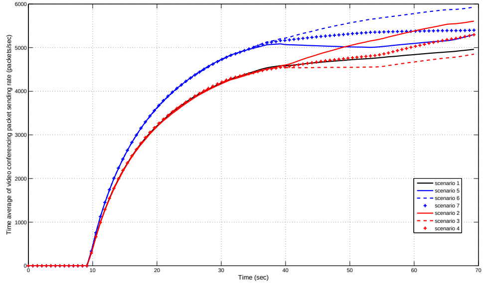
Figure 3.31: Time average of video conferencing packet sending rate (Case 1)
