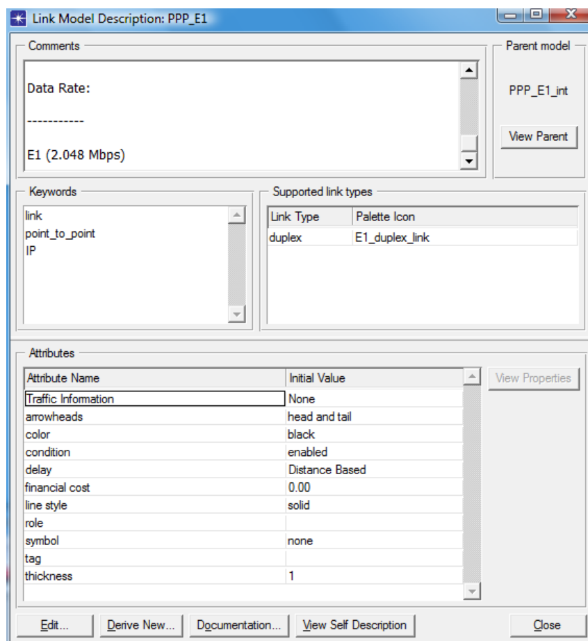
Figure 3.15: Link Editor
