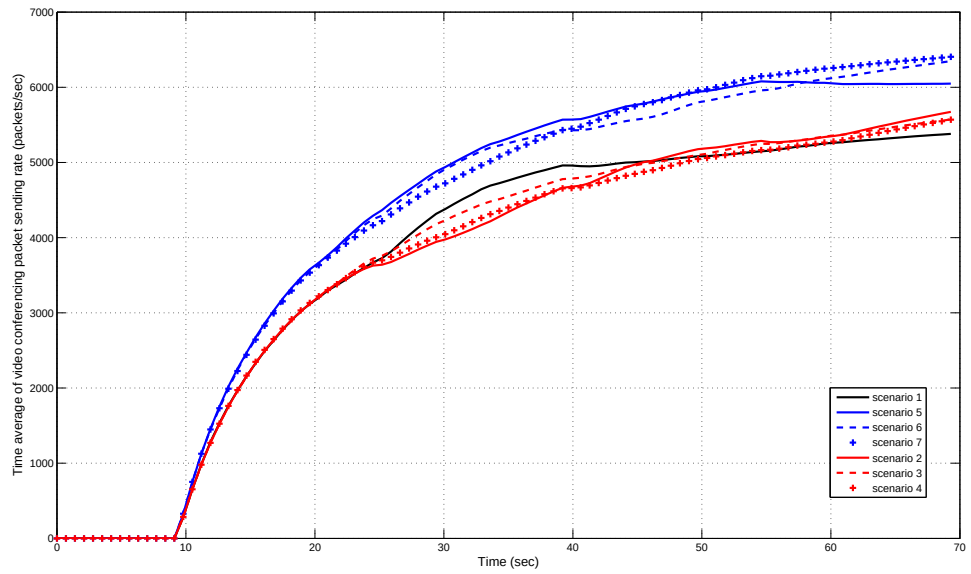
Figure 3.44: Time average of video conferencing packet sending rate (Case 2)
