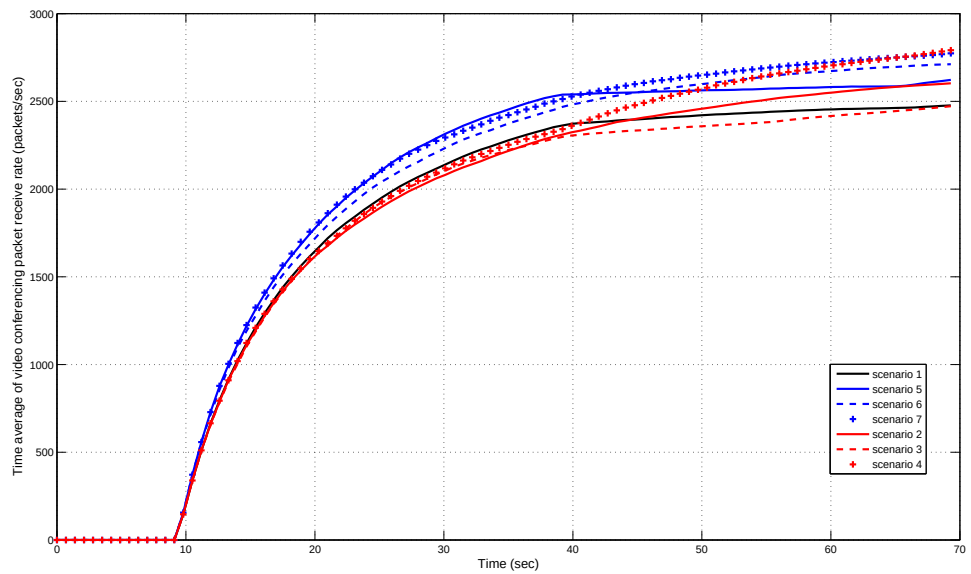
Figure 3.30: Time average of video conferencing packet receive rate (Case 1)
