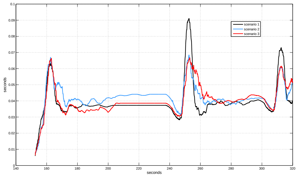
Figure 3.77: Moving average of end-to-end delay variation measured between node_2 and node_4
