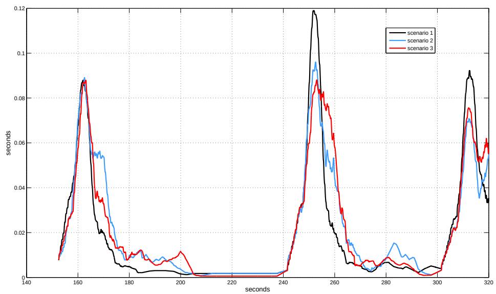
Figure 3.78: Moving average of end-to-end delay measured between node_3 and node_5
