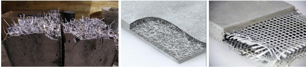
Figure 8: Fiber reinforcement methods with concrete.
