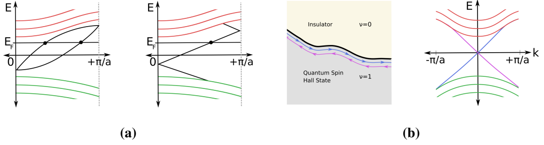
Figure 2.1: Zero-energy crossing of the bands within the band-gap at Fermi energy E_F (Fig. 2.1a) for a \mathbb{Z}_2 topological insulator. Between \Gamma_a and \Gamma_b an even number of crossings occurs for a trivial state. These crossings can be smoothly deformed to a bulk bandgap and are not topologically protected. Odd number of crossings (Fig. 2.1b), on the other hand, cannot be adiabatically transformed to a gapped band structure and thus are topologically protected, resulting in chiral edge-states.
