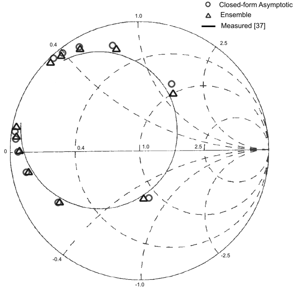
Figure 3.4: Input impedance data of a probe-fed, L = 2 cm by W = 3 cm rectangular antenna on a h = 0.127 cm thick grounded dielectric slab with \epsilon_r = 10.2 . Frequency = 2.2-2.4 GHz.
