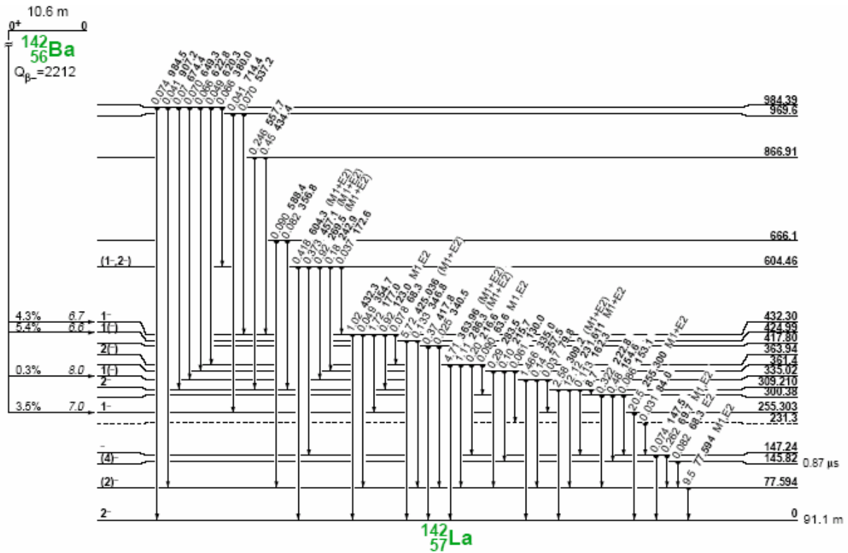
Şekil 5.32 ^{142}\text{Ba} \rightarrow ^{142}\text{La} t_{1/2}=10.6 m 8 \beta - bozunumu
