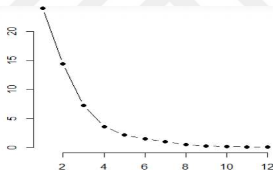
Figure 6. Optimal Number of Clusters Based on Elbow Plot in K-means Analysis
