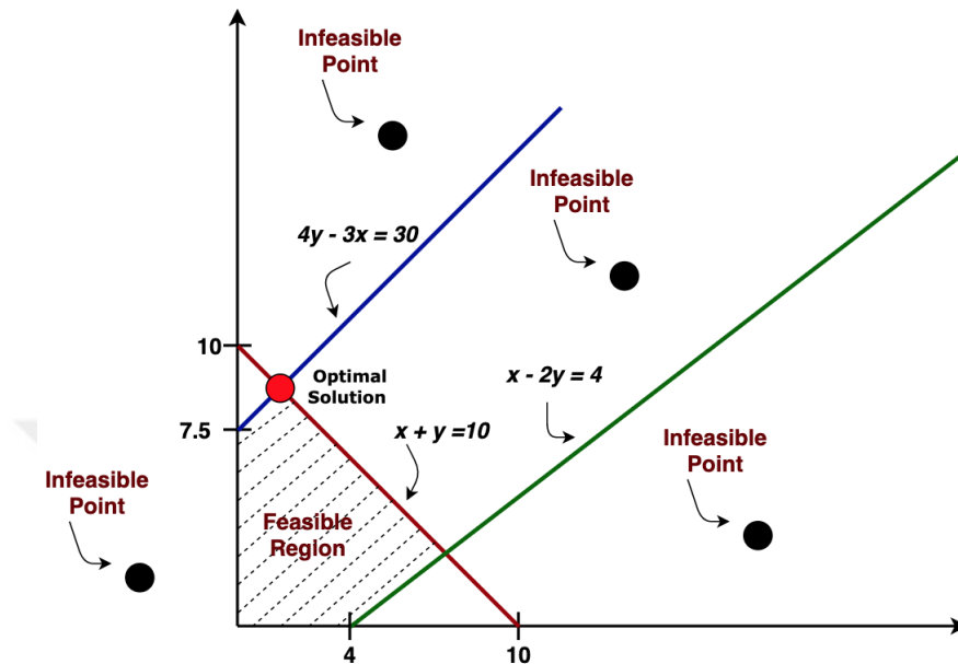
Figure 4.1: Linear Program - Graphical Method
