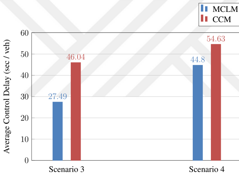
Figure 5.11: 15-Min Average Control Delay of the intersection for Scenario 3 and Scenario 4 - CCM and MCLM
