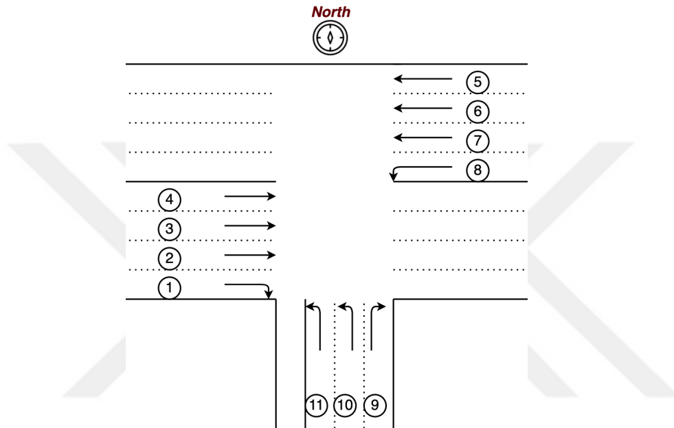
Figure 6.6: Intersection 2 - Geometry
