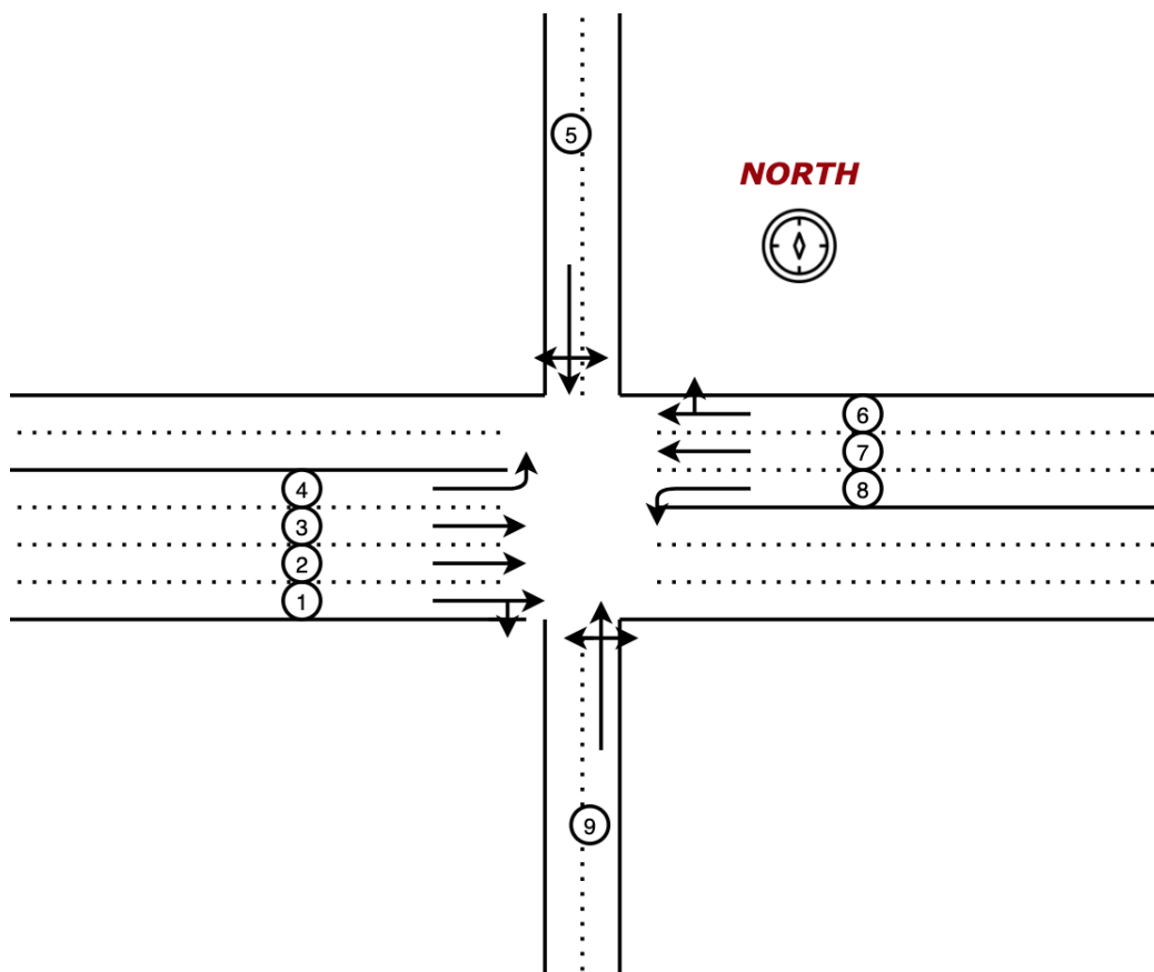
Figure 6.1: Intersection 1 - Geometry
