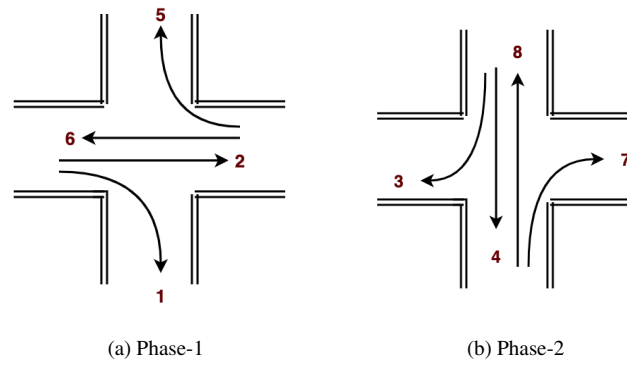
Figure 3.4: A sample phase design with 2 phases
