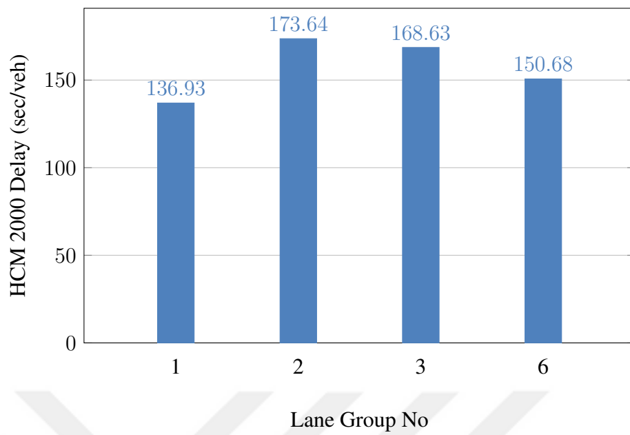
Figure 5.6: 15-Minute HCM Delay For Each Critical Lane Group for Scenario 1 - MMQLM
