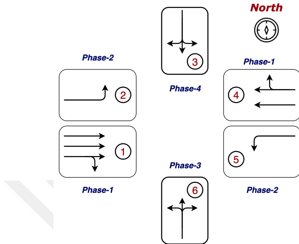
Figure 6.2: Intersection 1 - Phase Design and Lane Groups
