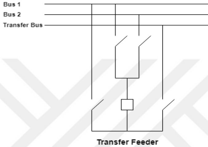
Figure 3.3. A Transfer Feeder Configuration in a Substation
