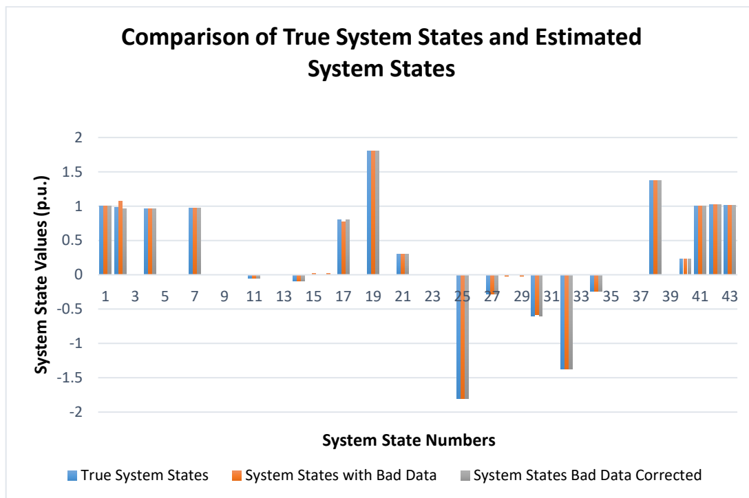
Figure 4.6. Small Scale Substation Scenario Bad Data Analysis - Comparison of System State Values
