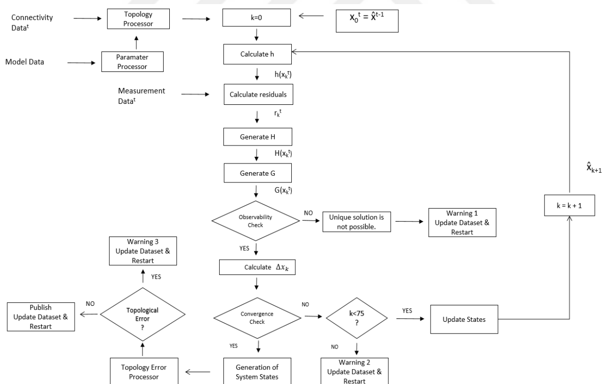
Figure 3.1. Substation Level State Estimation and Topology Error Processing Flow Chart
