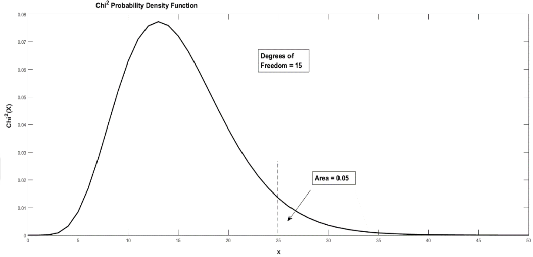
Figure 2.13. \chi^2 Probability Density Function
