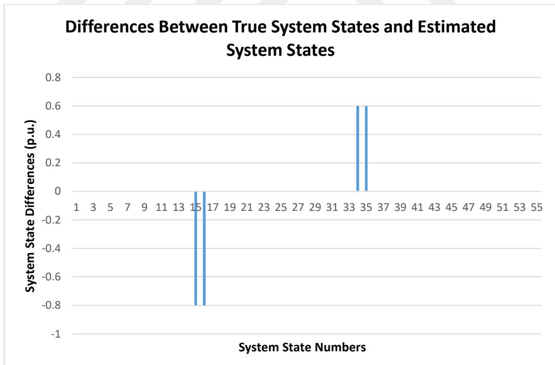
Figure 4.14 Large Scale Substation Scenario Topology Error Detection - Differences Between True System States and Estimated System States for Topological Error in Feeder Bays
