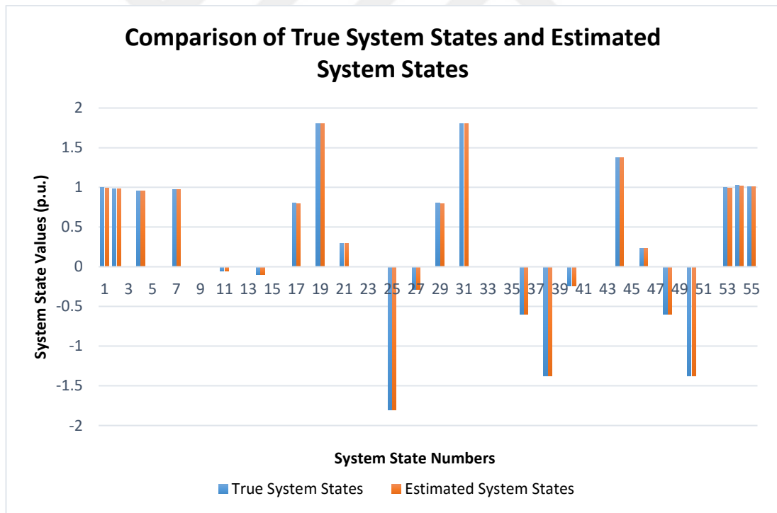
Figure 4.10 Large Scale Substation Scenario Topology Error Detection - Comparison of True System States and Estimated System States for Topological Error in Transfer Feeder
