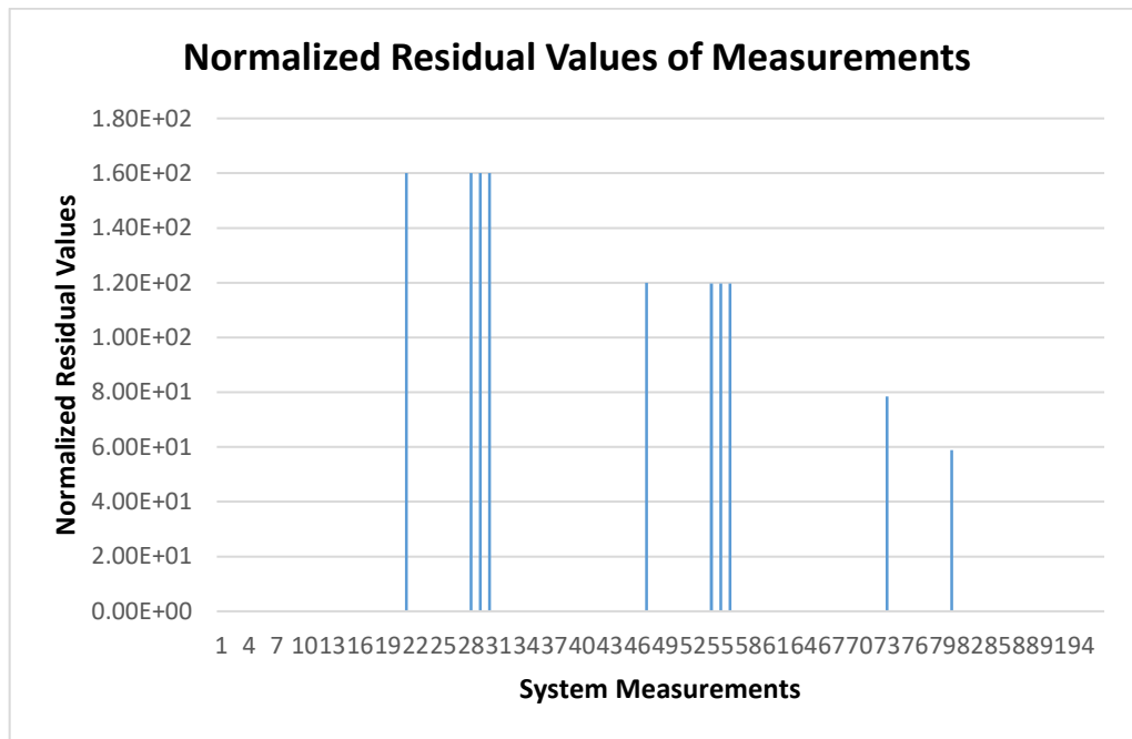
Figure 4.15 Large Scale Substation Scenario Topology Error Detection - Normalized Residual Values of Measurements for Topological Error in Feeder Bays
