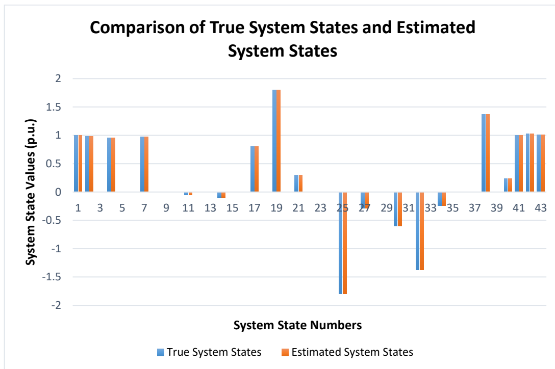
Figure 4.2 Small Scale Scenario Base Case - Comparison of True System States and Estimated System States
