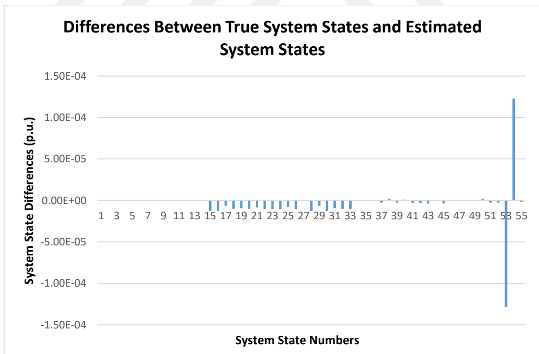
Figure 4.5 Large Scale Base Case - Scenario Differences Between True System States and Estimated System States
