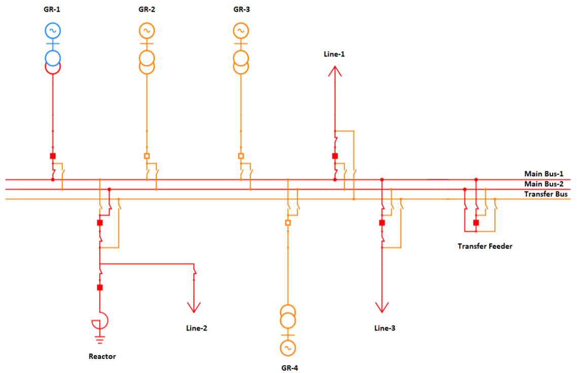
Figure 2.12. A Two Main Buses and a Transfer Bus Configuration Example
