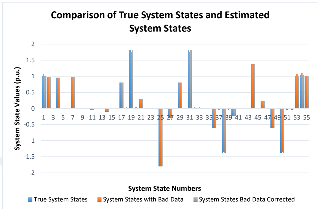
Figure 4.8. Large Scale Substation Scenario Bad Data Analysis - Comparison of System State Values
