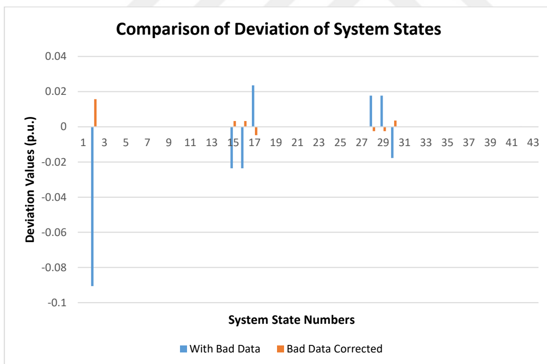
Figure 4.7. Small Scale Substation Scenario Bad Data Analysis - Comparison of Deviation of System States
