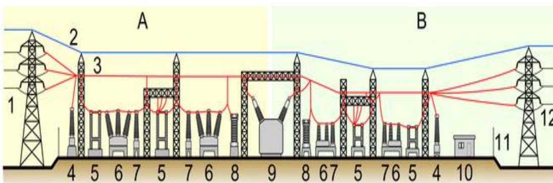
Figure 2.1. Elements of a Power Substation [17]
