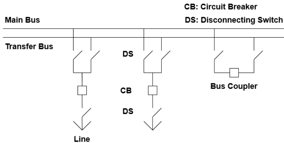
Figure 2.3. Double Busbar Single Circuit Breaker Configuration
