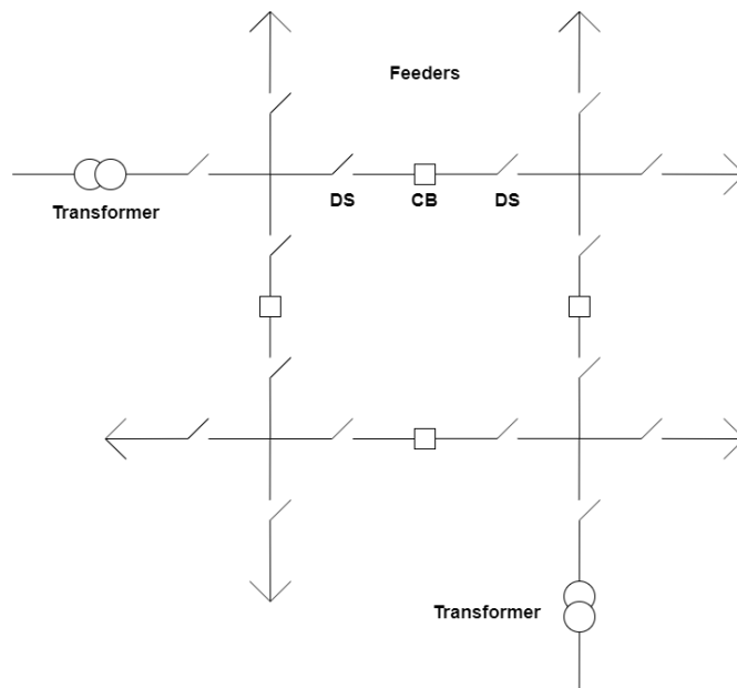
Figure 2.7. Mesh Configuration
