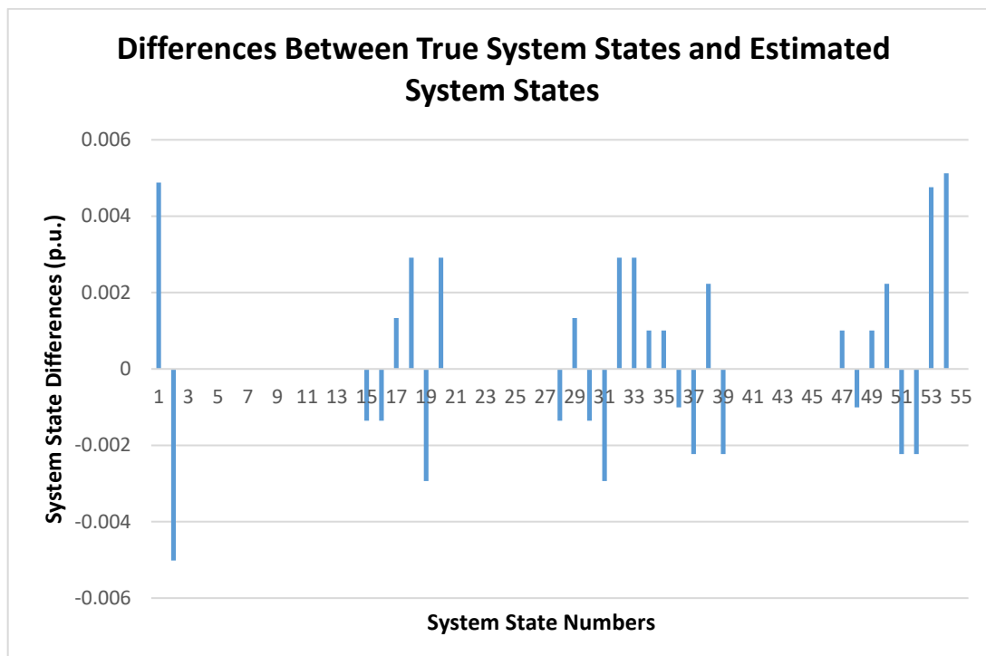
Figure 4.11 Large Scale Substation Scenario Topology Error Detection - Differences Between True System States and Estimated System States for Topological Error in Transfer Feeder
