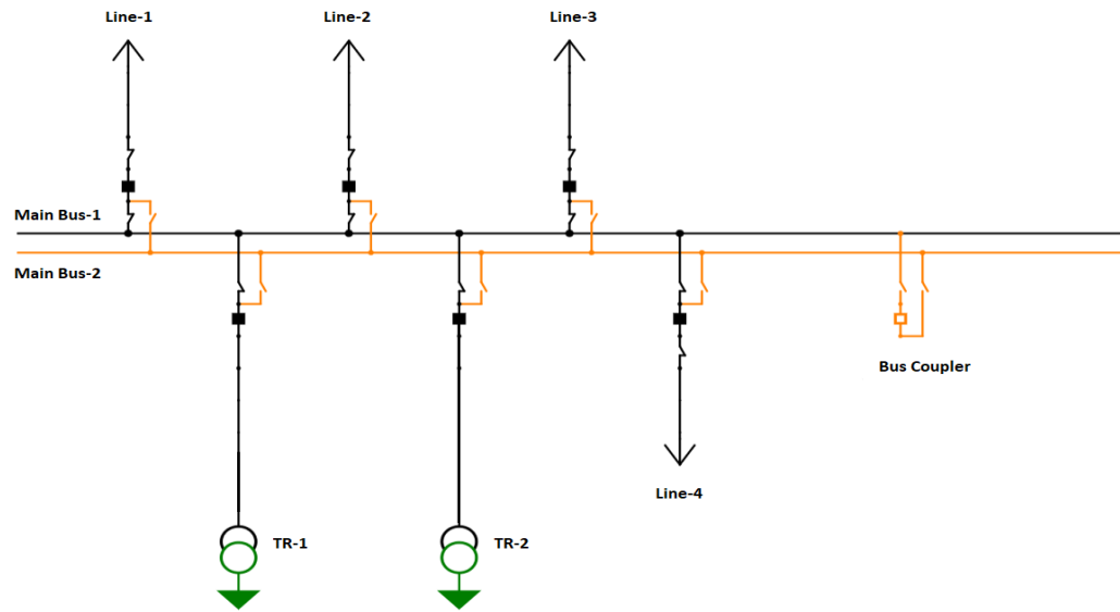
Figure 2.11. A Two Main Buses Configuration Example
