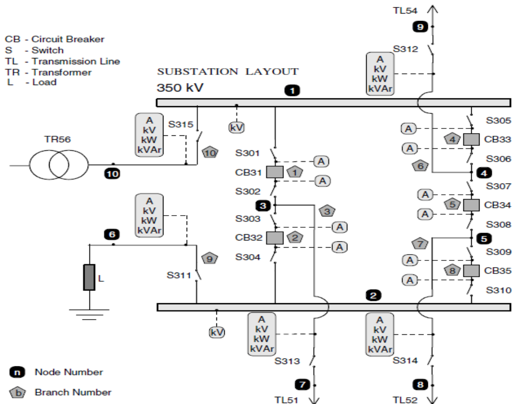
Figure 2.8. One-line diagram of a typical substation layout with measurement device allocation [4]
