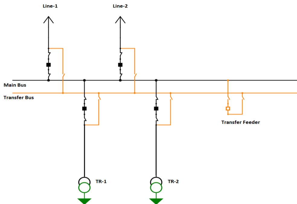
Figure 2.10. A Main Bus and a Transfer Bus Configuration Example
