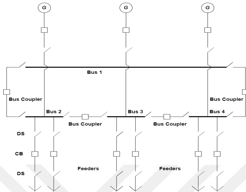
Figure 2.6. Ring Busbar Configuration
