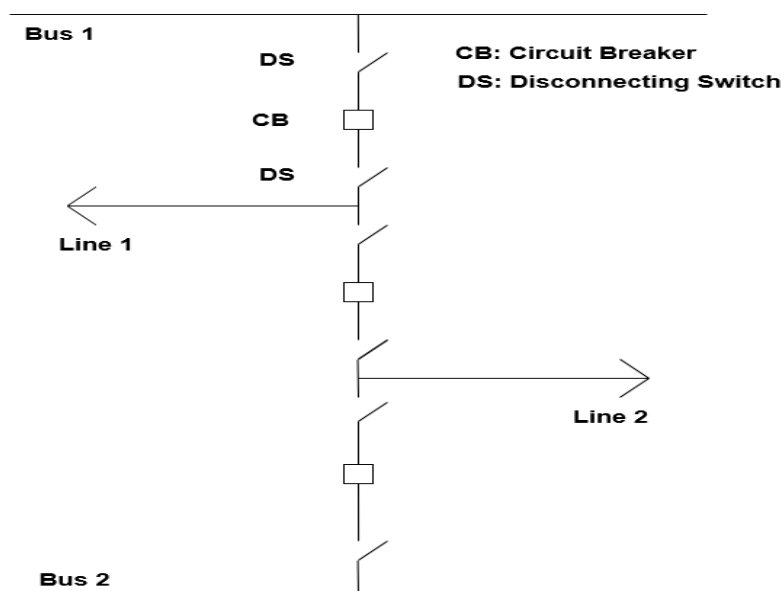
Figure 2.4. One and Half Breaker Configuration
