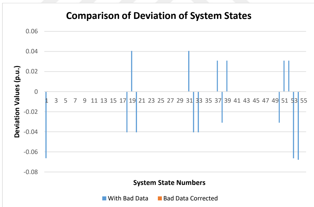
Figure 4.9. Large Scale Substation Scenario Bad Data Analysis - Comparison of Deviation of System States
