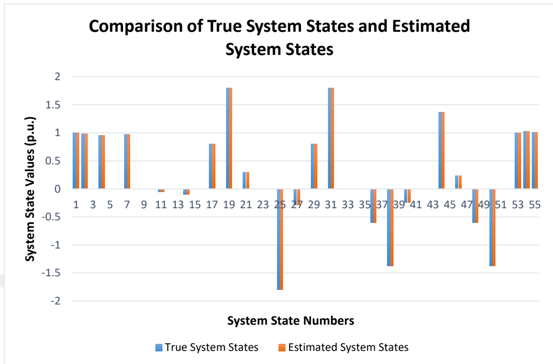
Figure 4.4 Large Scale Scenario Base Case - Comparison of True System States and Estimated System States
