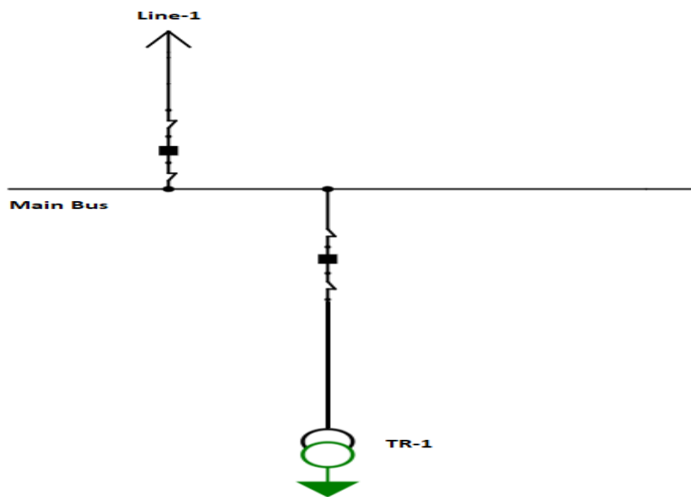
Figure 2.9. A Single Busbar Configuration Example
