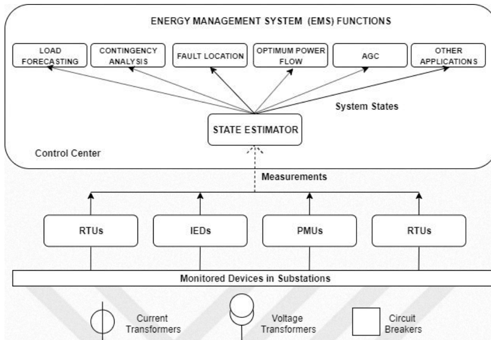
Figure 1.1. The Fundamental EMS System Structure
