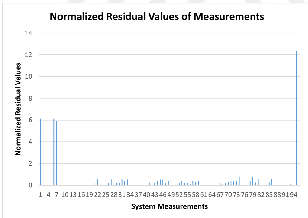
Figure 4.12 Large Scale Substation Scenario Topology Error Detection - Normalized Residual Values of Measurements for Topological Error in Transfer Feeder
