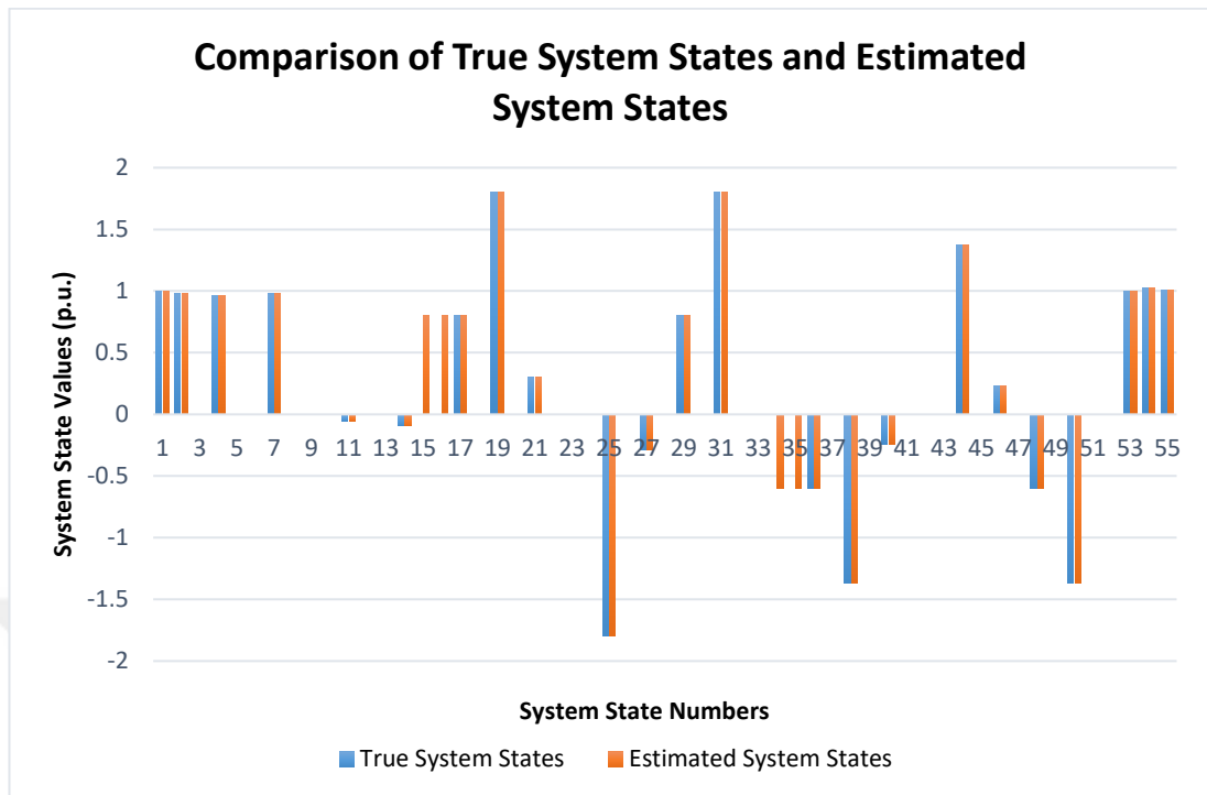
Figure 4.13 Large Scale Substation Scenario Topology Error Detection - Comparison of True System States and Estimated System States for Topological Error in Feeder Bays
