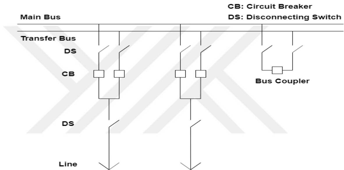
Figure 2.5. Double Busbar Double Breaker Configuration
