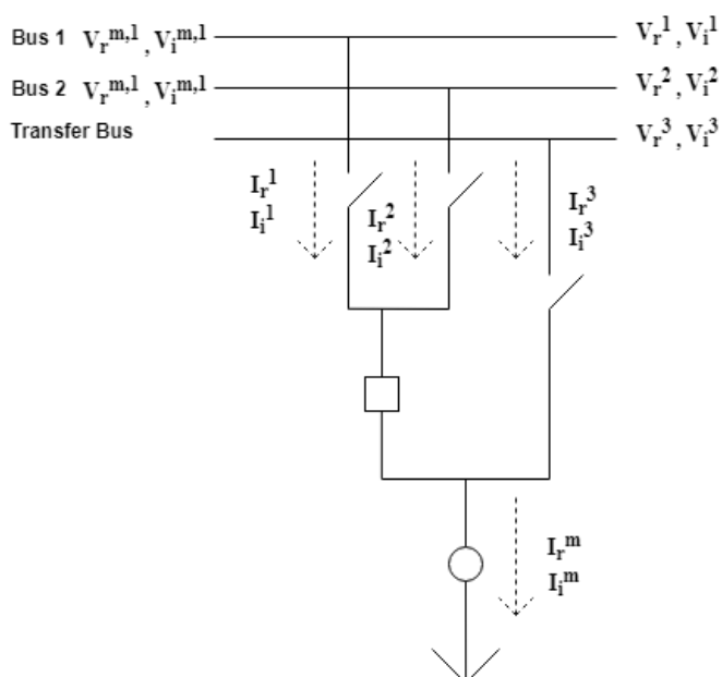
Figure 3.2. Current and Voltage States in a Substation
