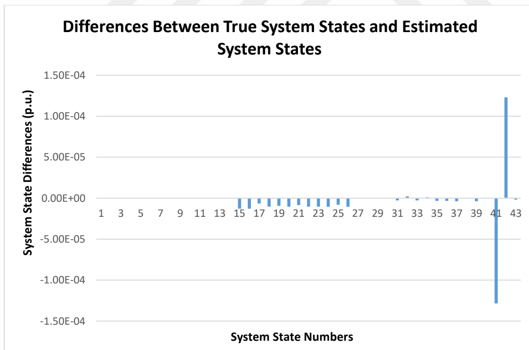
Figure 4.3 Small Scale Scenario Base Case - Differences Between True System States and Estimated System States
