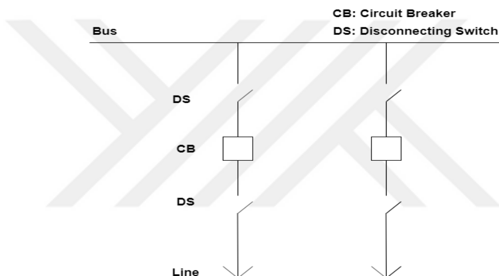
Figure 2.2. Single Busbar Configuration
