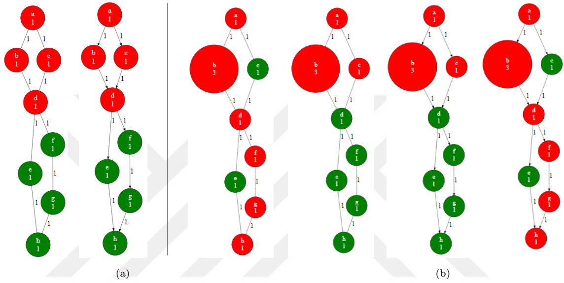
Figure 2.2: (a) Load balancing objective: Graph partitioning Algorithms ideal result (different colors represent partitions or processing elements). When the graph is undirected, loads are balanced and communication is minimized. When the graph is directed, no load balancing is achieved. (b) Communication minimization: when the graph is undirected, the second partitioning (from the left) is better than the first since it has two units of communication as opposed to four in the first. When the graph is directed, the notion of communication hiding is present. This means that the communication taking place while there is a work being done is not considered as it does not impose any latency. Thus the fourth partitioning is better than the third since the communications from a to c, from c to d and from d to e are hidden by the execution of the tasks b, f and g respectively.
