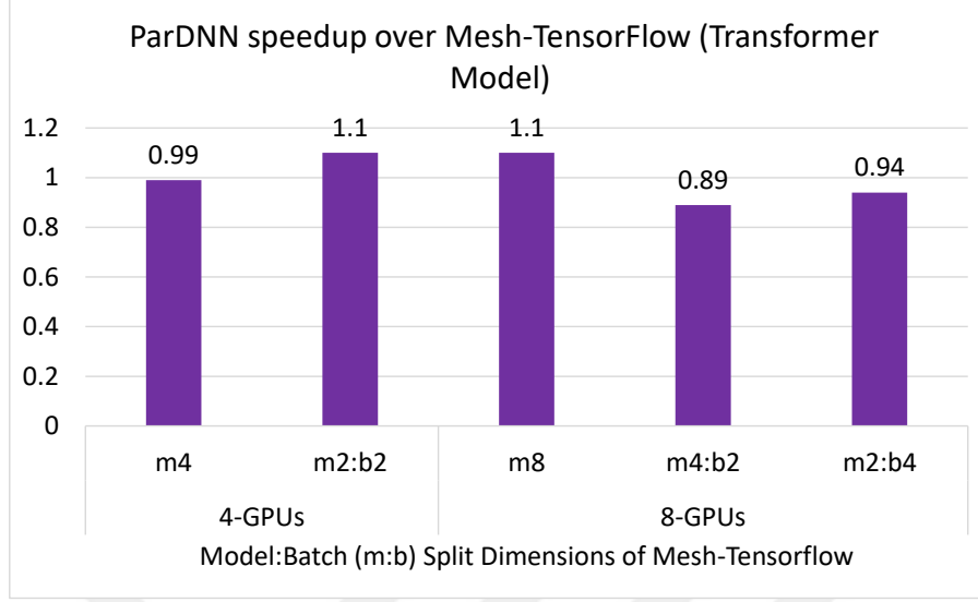
Figure 6.3: PARDDNN speedup over Mesh-TensorFlow using 4 GPUs and Transformer (TRN) model
