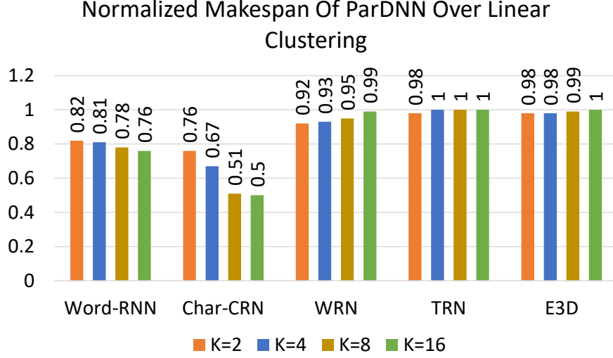
Figure 6.7: Makespan of PARDNN over that of Linear clustering (lower is better). Results are rounded to the 2 nd digit after the decimal point.
