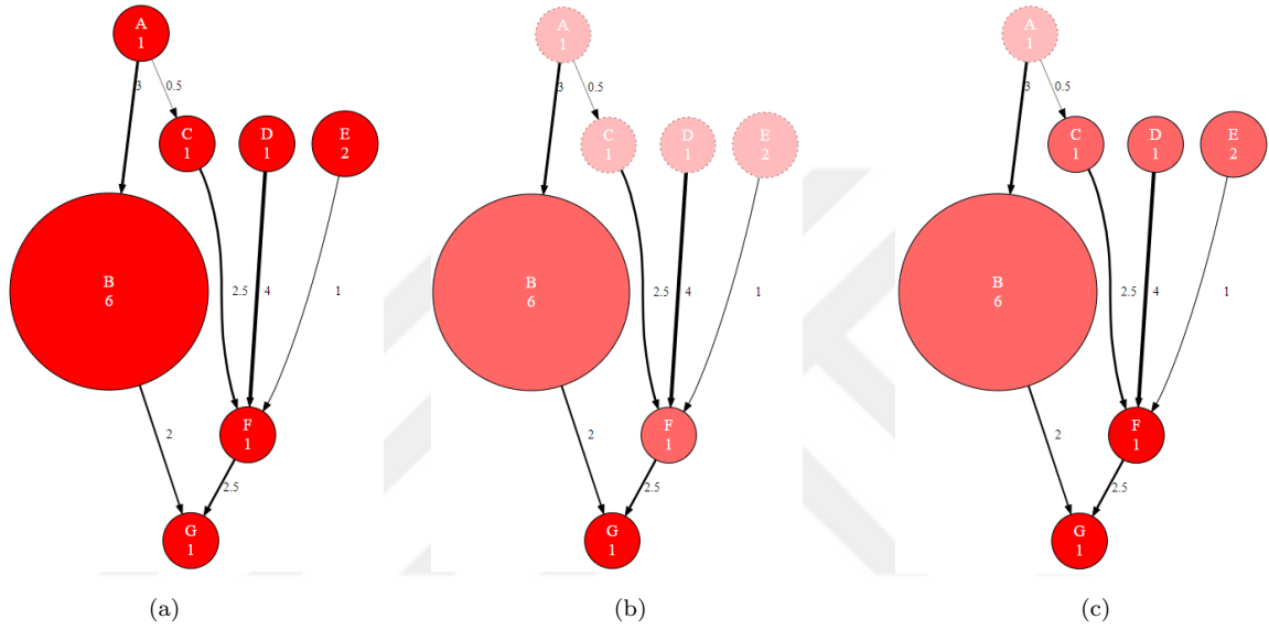
Figure 4.3: (a) a task graph where the numbers inside the nodes indicate the memory required to store the task outputs. (b) assuming the schedule A, C, D, E, F, B, G. When G is scheduled to run we have the outputs of B and F held in the memory plus the newly allocated memory for G output totalling to 8 units; which is the peak memory consumption for this schedule. (c) assuming the schedule A, B, C, D, E, F, G, the peak consumption occurs when F is scheduled totalling to 11 units (coming from B, C, D, E and F). The fading nodes are the ones for which all the dependencies have run, hence their memory is released since it is not needed any more.
