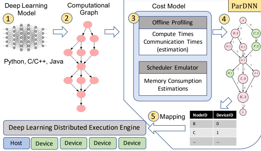
Figure 4.1: PARDDNN Overview
