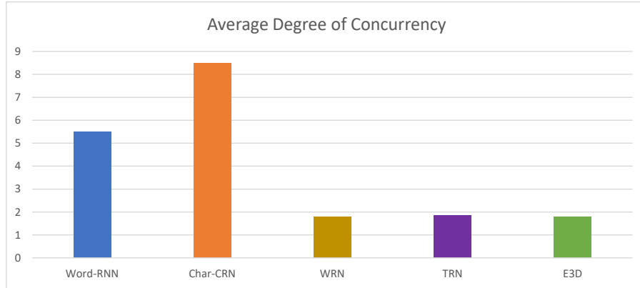
Figure 6.2: The average degree of concurrency, or the degree of parallelism in the graphs.
