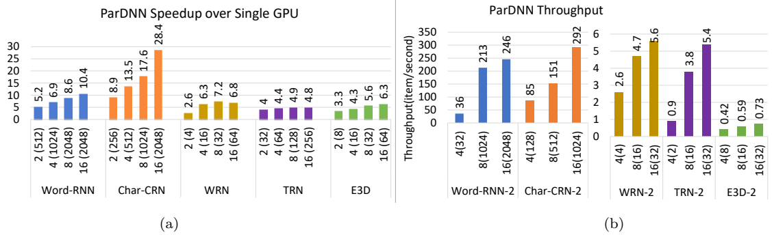
Figure 6.1: (a) PARDNN speedup using 2, 4, 8 and 16 GPUs over one GPU. (b) The throughput scaling of PARDNN with larger models on 4, 8 and 16 GPUs
