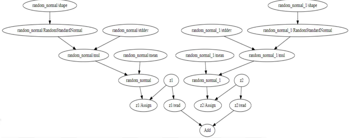
Figure 2.1: Simple code snippet for adding two randomly generated tensors and the corresponding Tensorflow dataflow graph representation
