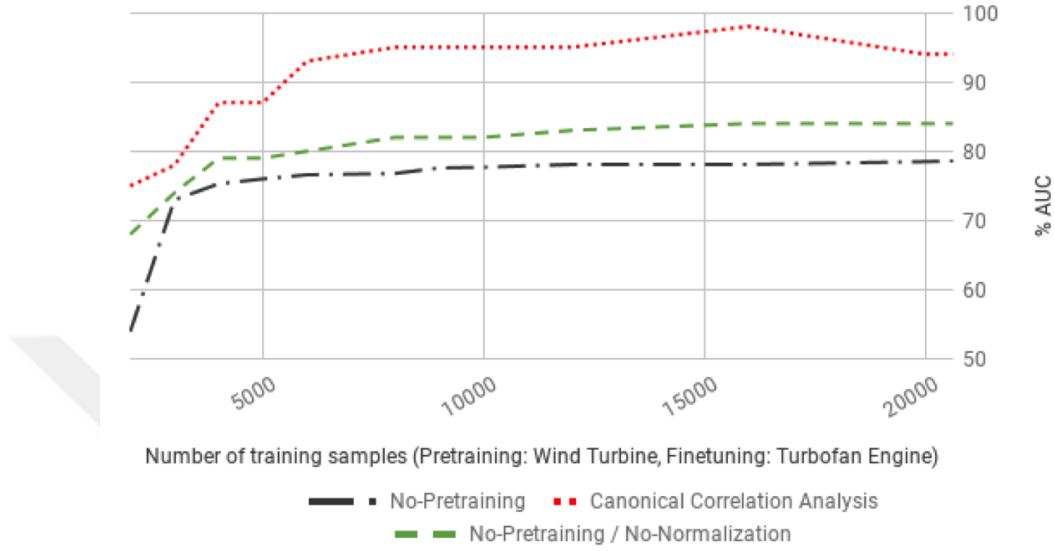
Figure 4.8: CCA for normalization
