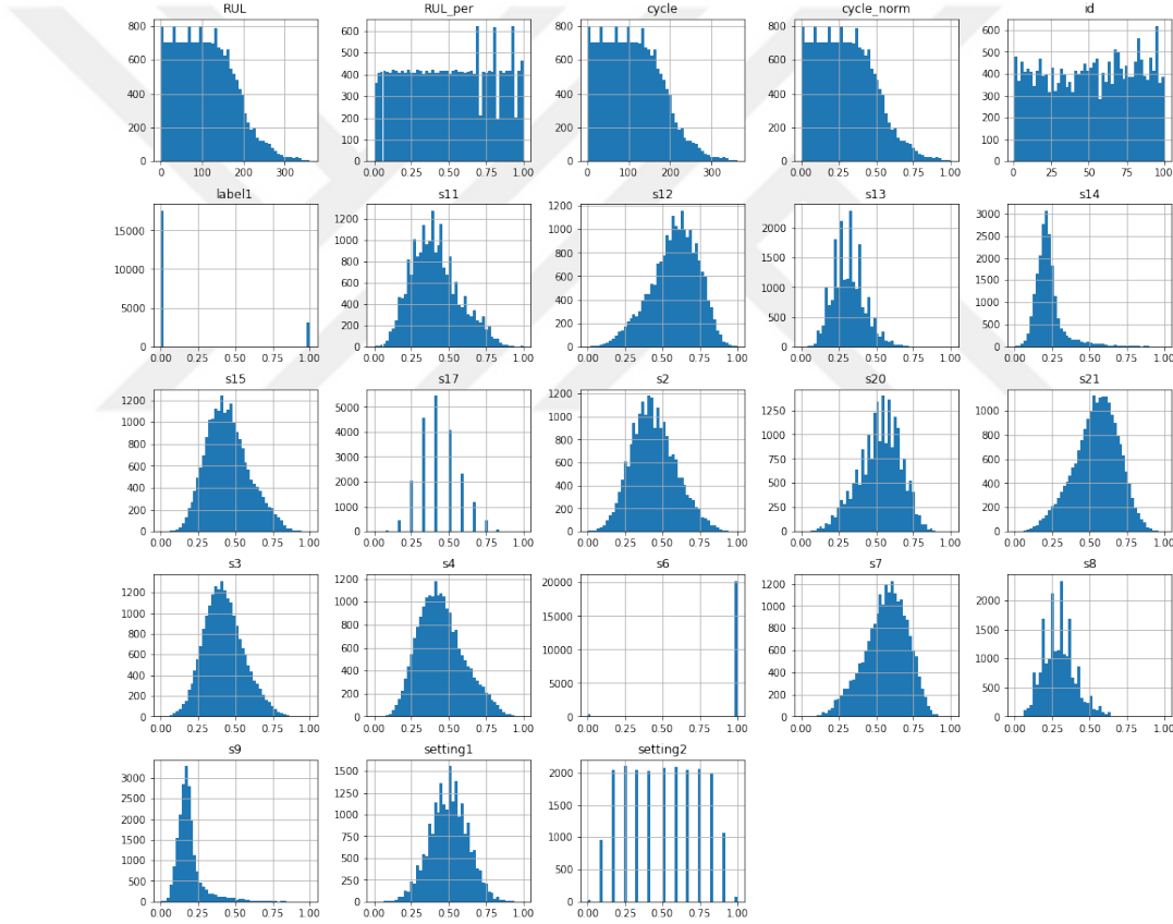
Figure 4.1: Turbofan engine feature distribution
