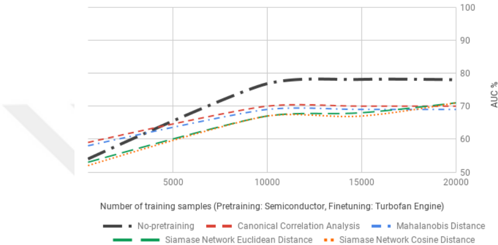
Figure 4.9: The impact of different common representation learnings on transfer learning
