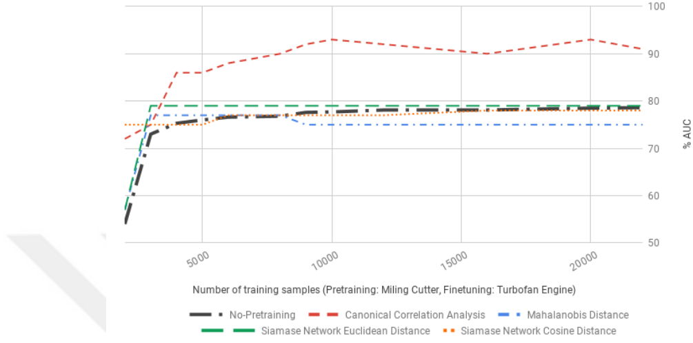
Figure 4.5: The impact of different common representation learnings on transfer learning
