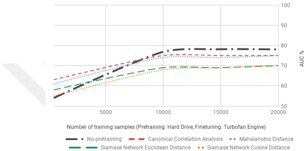
Figure 4.6: The impact of different common representation learnings on transfer learning
