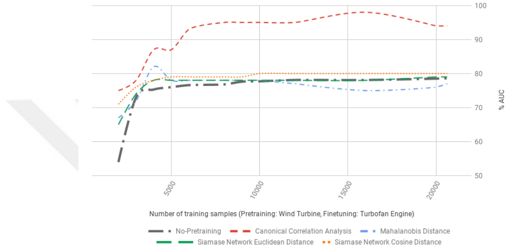
Figure 4.4: The impact of different common representation learnings on Transfer Learning
