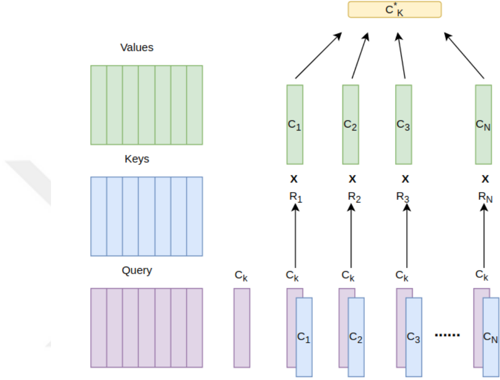
Figure 2.3: C_K^* represent query C_K in terms of weights R_i sum values, with weights define by match between query and keys. i and K is element of N that is the number of words in the context.
