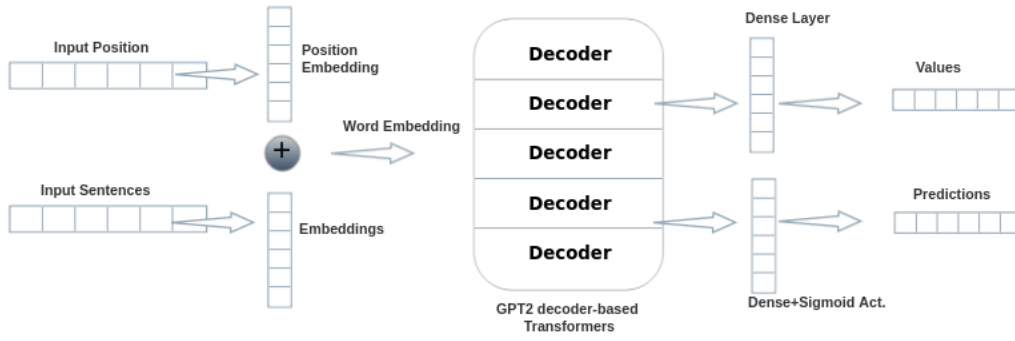
Figure 3.4: Binary classification model based on GPT-2
