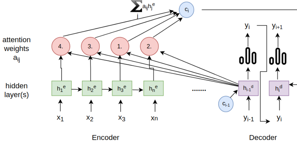
Figure 2.1: All hidden-layer based on RNN and h_i^e are encoder block and h_i^d are decoder block. i is an element of N that is the number of words in the context. (Lam, 2021)
