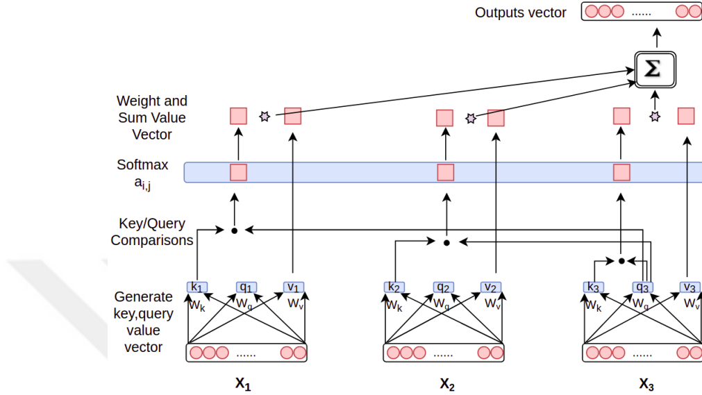
Figure 2.4: Self-attention (Lam, 2021)
