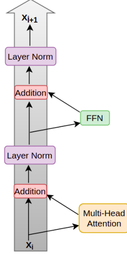
Figure 2.8: Residual blocks (Xiong et al., 2020)
