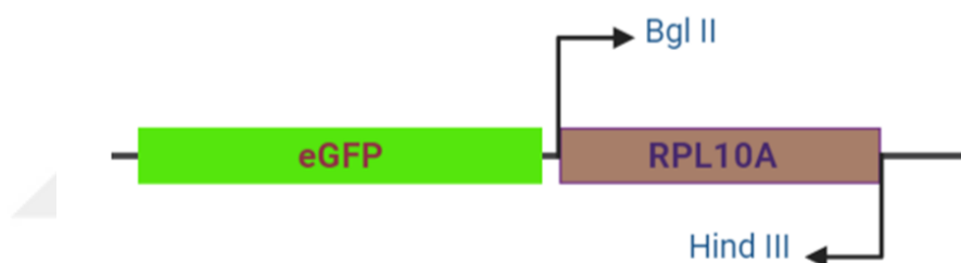
Figure 3.1 Cloning RPL10A coding sequence into pEGFP-C1 vector to synthesize RPL10A N-terminal fusion with eGFP
