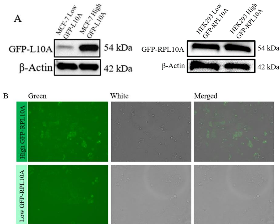
Figure 3.4 High and Low eGFP-L10A expressions. (A) 50 \mu g protein was used for western blotting in both HEK293 and MCF-7 cell lines. GFP Ab: SantaCruz, sc-9996, 1:500 dilution was prepared in 0.5 %TBST with 5% skim-milk. ACTB ( \beta -Actin) Ab: SantaCruz, sc47778 1:4000 dilution was prepared with 0.5% TBST and 3% skim-milk. B) High and Low eGFP-RPL10A expressing MCF-7 cells were observed with Flouid under 20X magnification.
