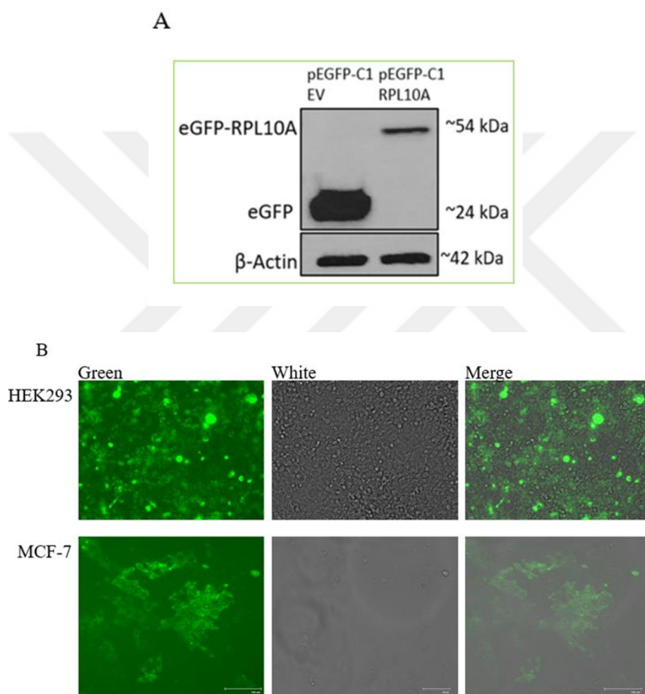
Figure 3.2 eGFP-RPL10A expression in transiently transfected HEK293 and MCF-7 cell lines. (A) eGFP and eGFP-RPL10A expression in HEK293 cell line, isolated proteins (50 µg) were loaded to 10% SDS-polyacrylamide gel GFP Ab: SantaCruz, sc-9996, (1:500 dilution in 0.5 %TBST with 5% skim-milk). ACTB (β-Actin) Ab: SantaCruz, sc47778 1:4000 dilution in 0.5% TBST and 3% skim-
