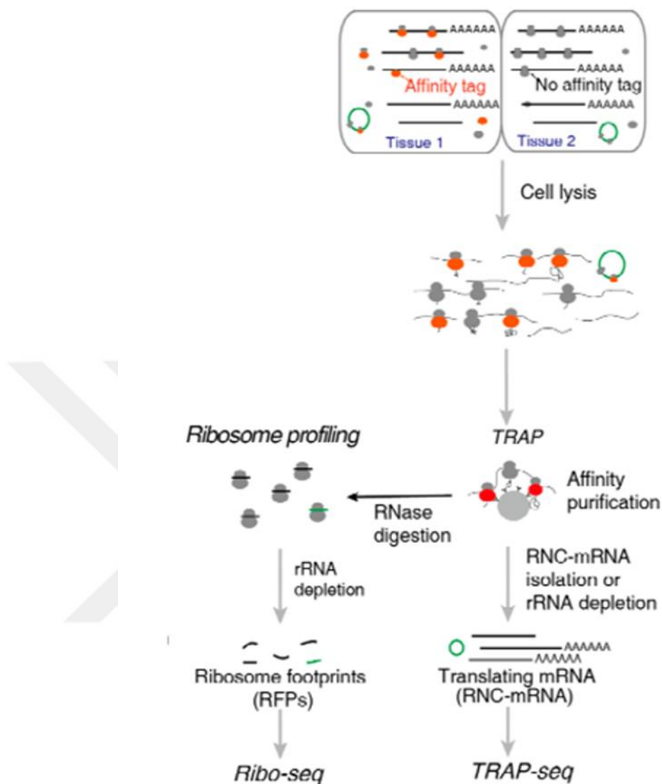
Figure 1.8 Ribosome Profiling and Translating Ribosomal Affinity Purification (TRAP)
