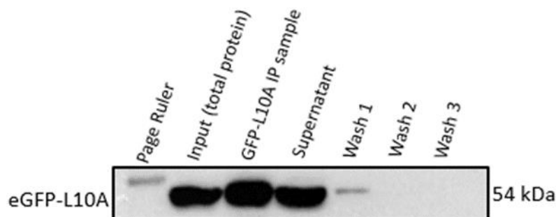
Figure 3.5 Control immunoprecipitation of eGFP-RPL10A in HEK293 cells. Immunoprecipitation was performed with Anti-GFP VHH Single Domain Antibody (Magnetic Beads) (ABCAM, ab-193983). 1000 µg of immunoprecipitated protein was loaded to 10% SDS-polyacrylamide gel and then transferred to the PVDF membrane. GFP Ab: Santa Cruz, sc-9996, 1:500 dilution was prepared in 0.5 %TBST with 5% skim-milk.
