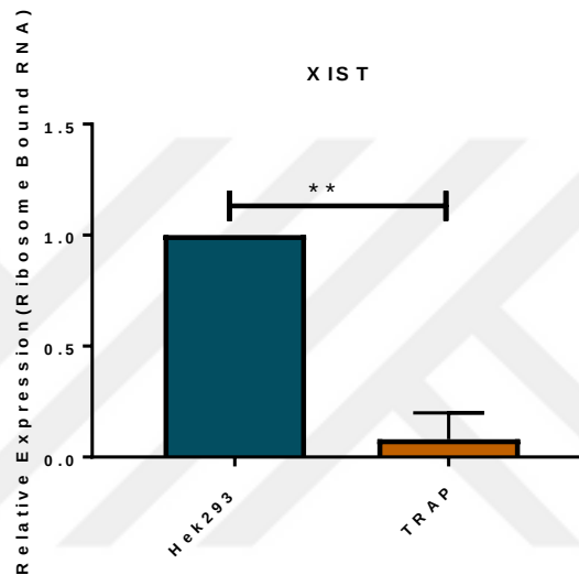
Figure 3.7 lncRNAs as a negative control. (A) conventional PCR with MALAT1 specific primers (35 cycles, annealing temperature is 65°C); product length 167 bp. Samples are untransfected HEK293 cell line cDNA and HEK293 TRAP cDNA. (B) RT-qPCR of XIST transcript. XIST expression level was normalized to that of untransfected HEK293 cell line. N=3 IP, every RT-PCR contains three technical replicates. Welch's t test was applied, p=0.0055 (**)
