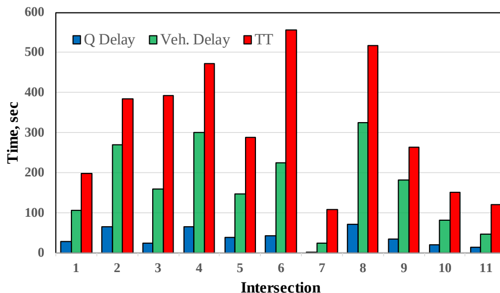
Figure 4.19. Traffic performance metrics for Route1 from Vissim.
