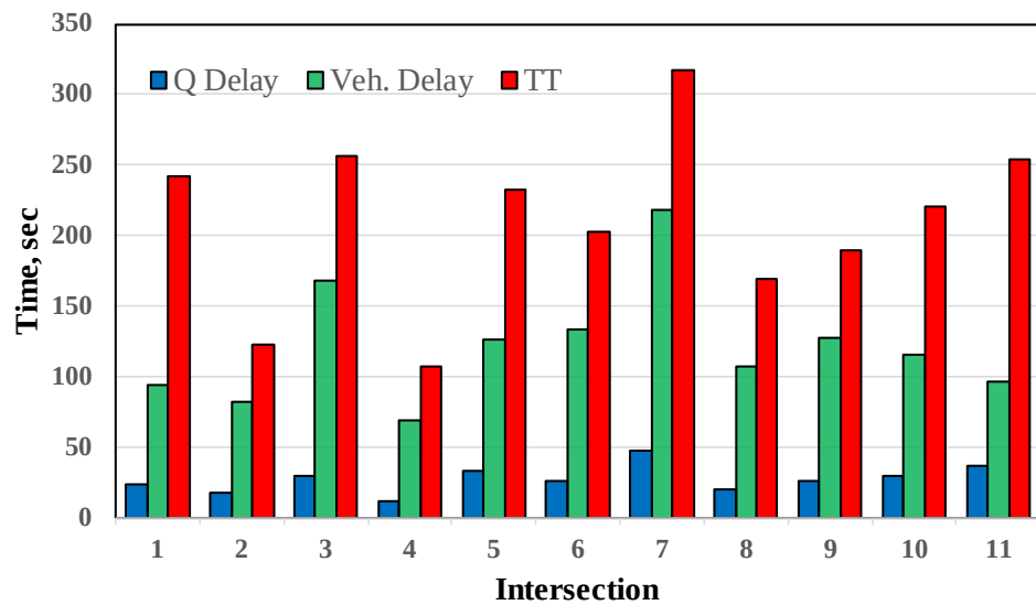
Figure 4.23. Traffic performance metrics for Route3 from Vissim.
