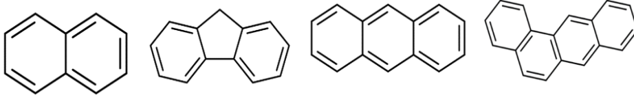
Naphthalene Fluorene Anthracene Benzantracene
