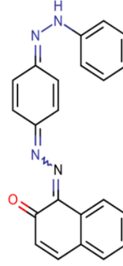
Sudan III
