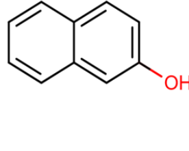
2-Naphtol
