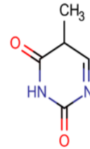
Thymine
