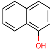
1-Naphtol
