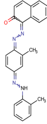
Sudan IV
