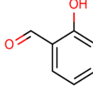
Salicylaldehyde
