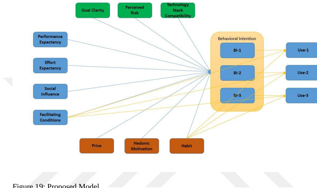
Figure 19: Proposed Model
