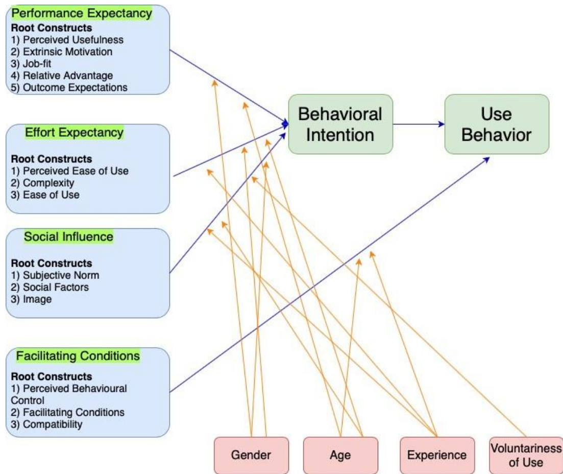
Figure 4: UTAUT Model
