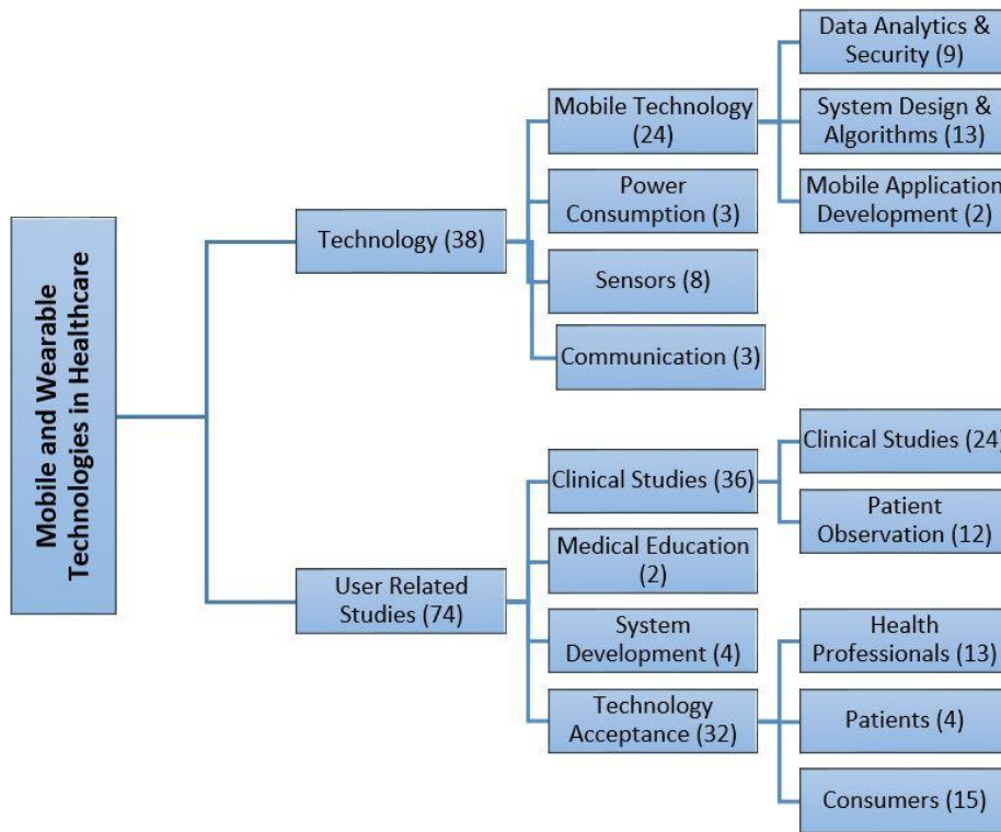
Figure 7: Article Classification
