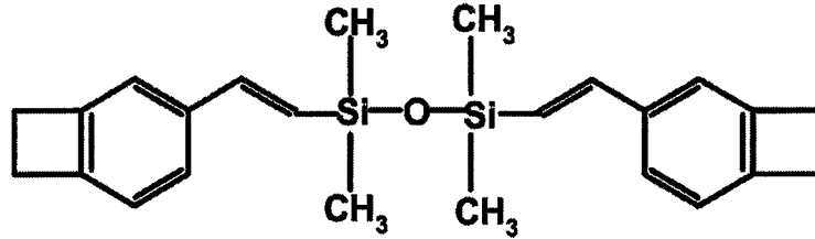
Figure 4. 11: Schematics of BCB monomer.
