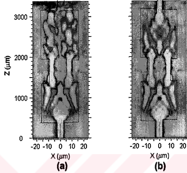
Figure 3. 7: BPM simulation of MMI modulator for off (a) and on state (b).
