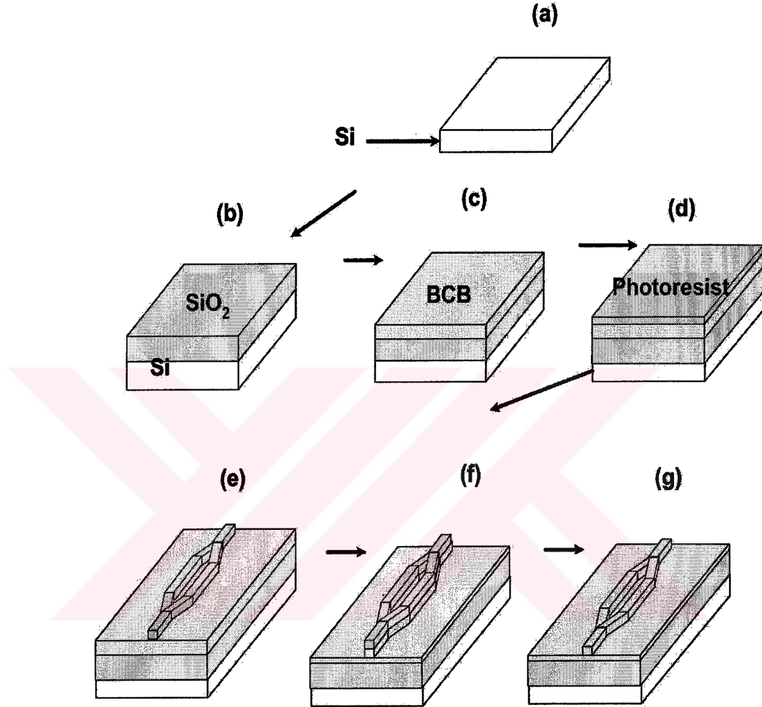
Figure 4. 13: Fabrication procedure of polymer waveguide, (a) Cleaned silicon substrate, (b) PECVD \text{SiO}_2 deposition, (c) BCB Spinning, (d) Photoresist spinning, (e) Photolithography, (f) RIE Etching, (g) Removing PR
