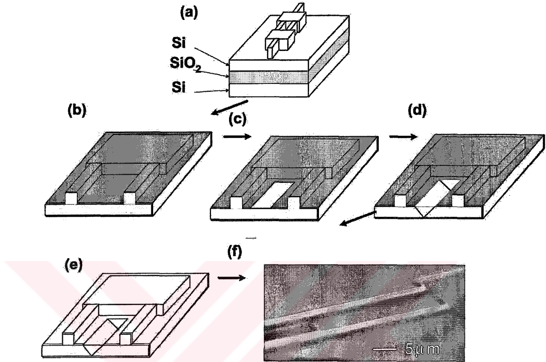
Figure 3. 15: Trench patterning steps of SOI optical waveguides (a) Si MMI waveguide, (b) Si_3N_4 Deposition, (c) Defining trench pattern, (d) KOH Etching, (e) Removing Si_3N_4 , (f) SEM photograph of MMI modulator .
