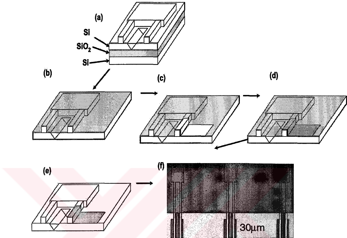
Figure 3. 16: Electrode metallization of thin film heaters (a) Patterned Si waveguide, (b) Spinning PR, (c) Defining heater, (d) Al evaporation, (e) Liftoff, (f) Top view optical microscope photograph of heaters and electrodes.
