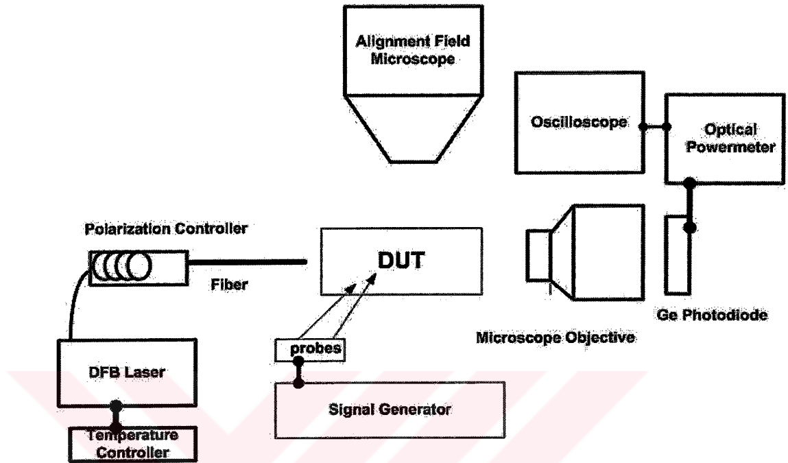
Figure 3. 17: Optical measurement setup.
