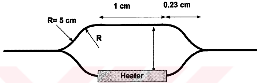
Figure 4. 4: Schematic diagram of MZI structure used in modulator .
