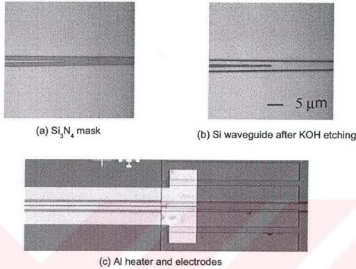
Figure 4. 7: Fabrication steps for MZI
