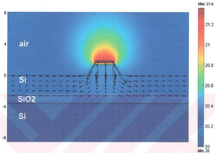
Figure 4. 5: Simulated 2D temperature profile of MZI.
