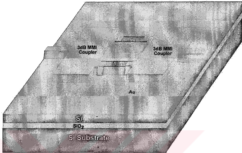
Figure 3. 8: Sidewiew of MMI modulator
