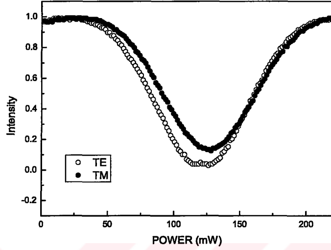
Figure 3. 19: Normalized output light intensity as function of applied electrical power.
