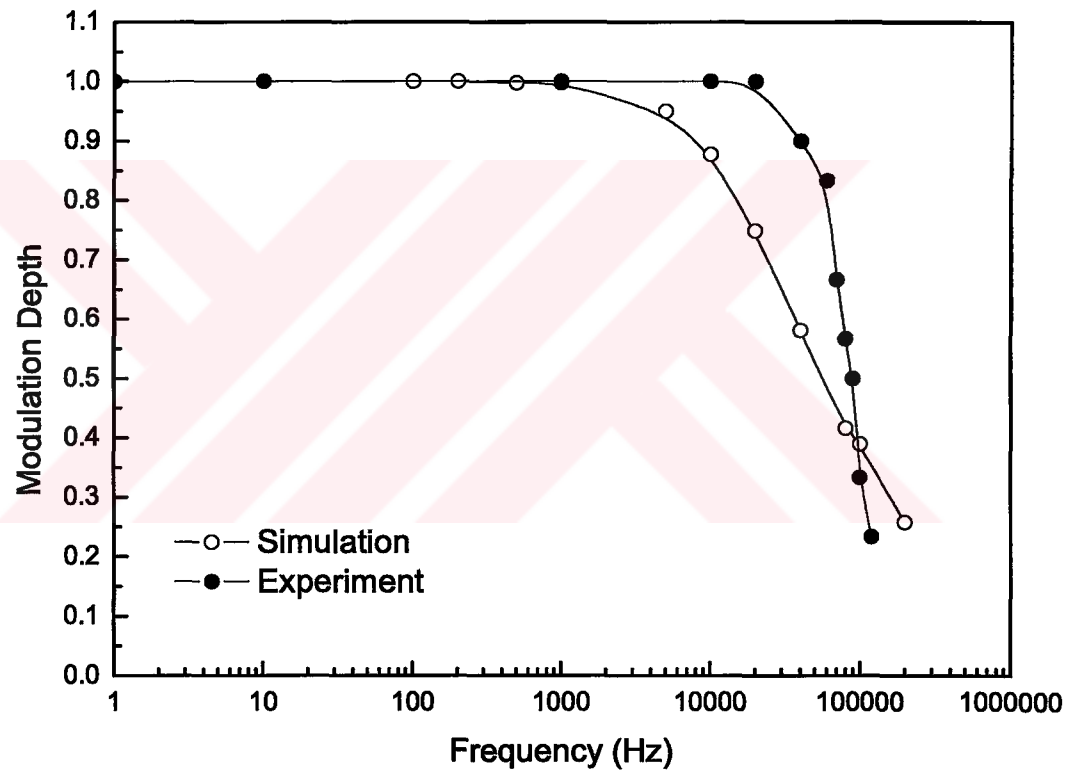
Figure 3. 21: Normalized modulation depth as a function of frequency.
