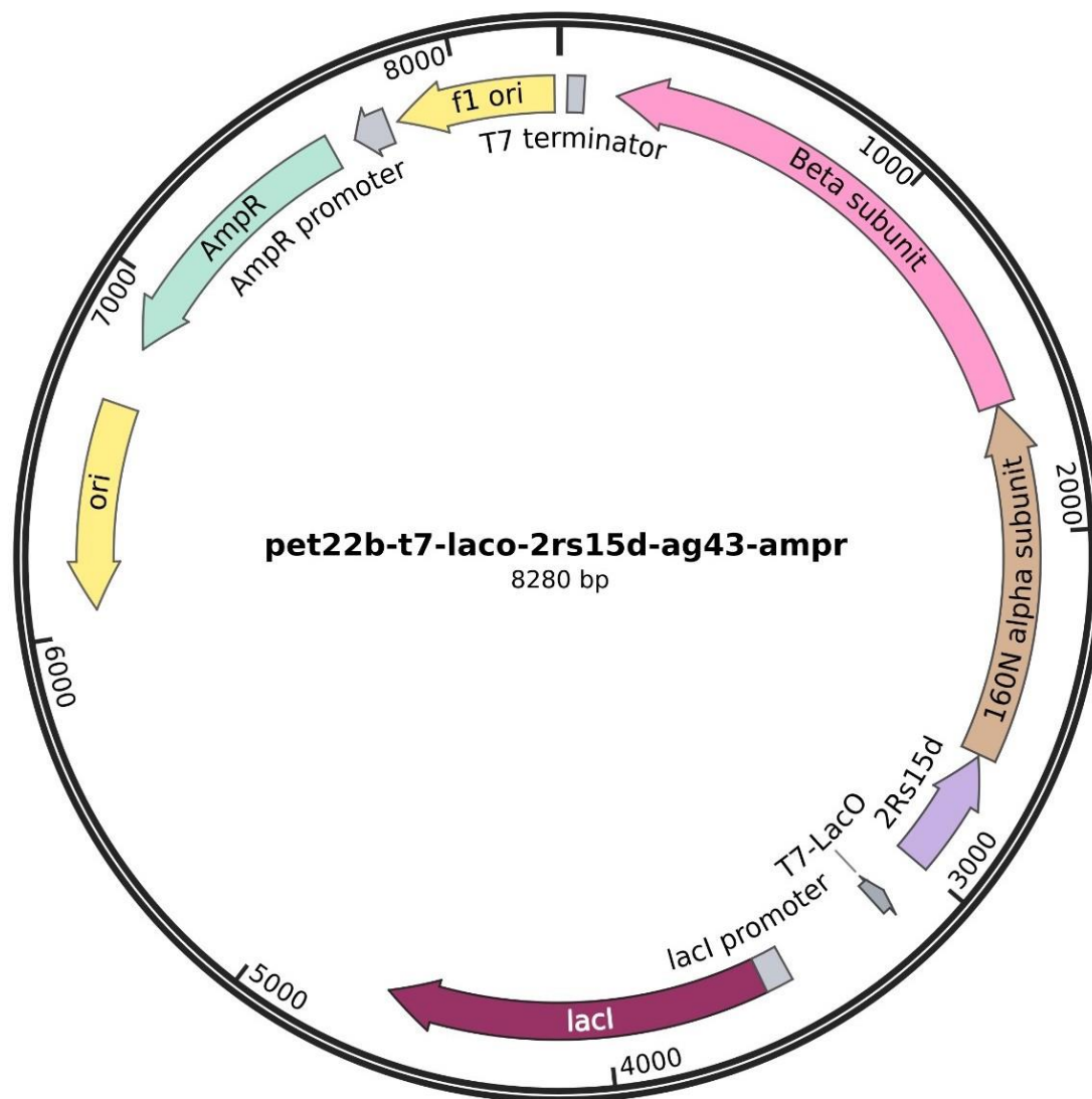
Figure 53. Plasmid map of pET22b T7 lacO 2Rs15d Ag43 AmpR vector.
