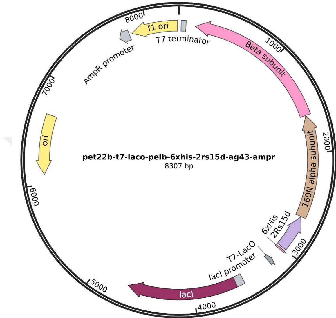
Figure 54. Plasmid map of pET22b T7 lacO 6xhis 2Rs15d Ag43 AmpR vector.
