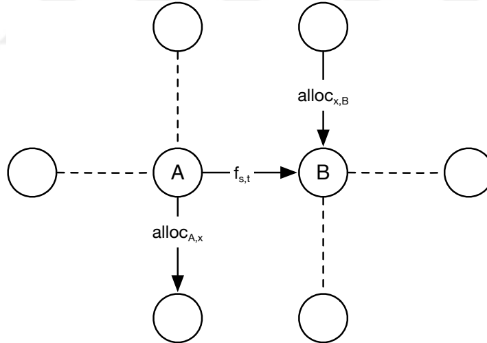
Figure 5.9: Potential cost of assigning (A, B) to flow (s, t) : \text{Potential-cost}(s, t, A, B, \text{alloc}) .
