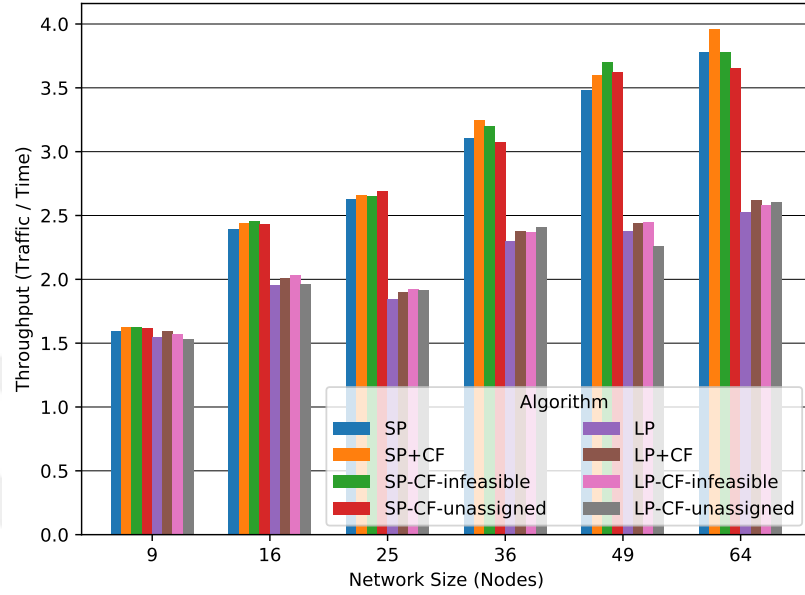
Figure 6.15: Effective bandwidth.
