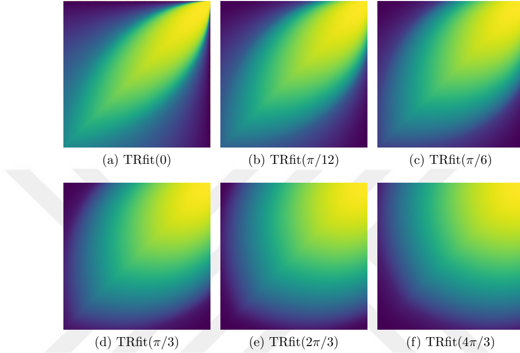
Figure 3.5: Visualization of TRfit for different parameter values.
