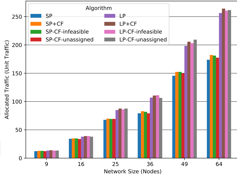
Figure 6.11: Allocated traffic.
