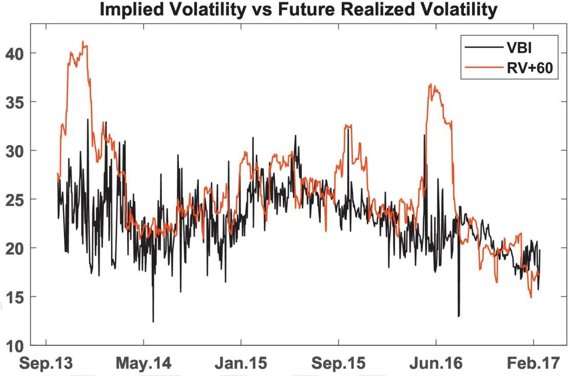
Figure 2.2: Implied volatility vs realized volatility in the next 60 calendar (44 trading) days.
