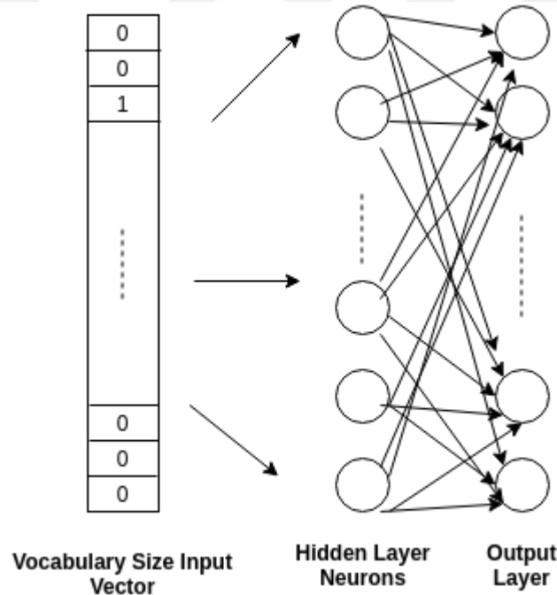
Figure 3.1: Example Representation of One Layer Neural Network
