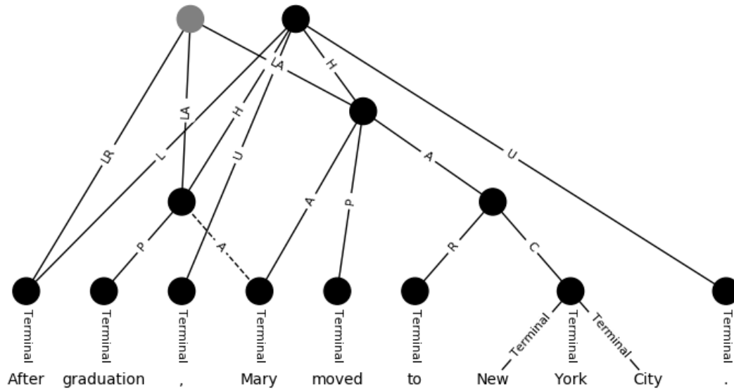
Figure 2.1 An Example of UCCA annotation for the sentence “After graduation, Mary moved to New York City.”
