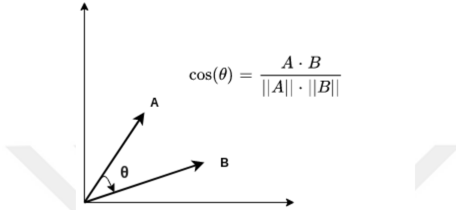
Figure 3.2: Representation of Cosine Similarity
