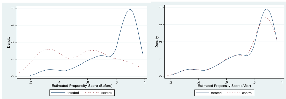
Figure 17. Kernel Density Estimates of Propensity Score Distributions
