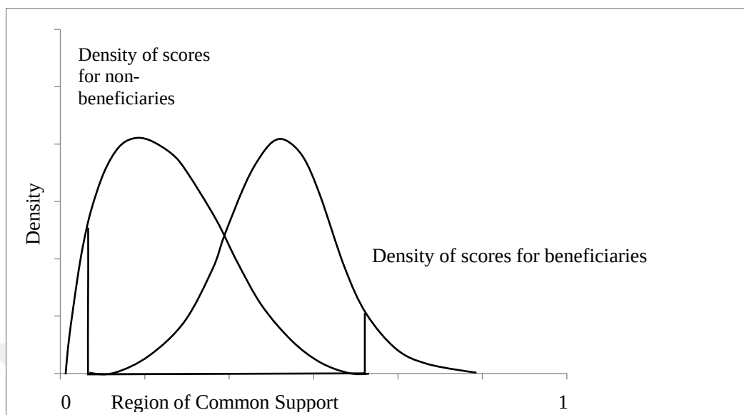
Figure 14. Example of Common Support Region (Source: Khandker et al., 2010, “Handbook on Impact Evaluation: Quantitative Methods and Practices”, p.57)
