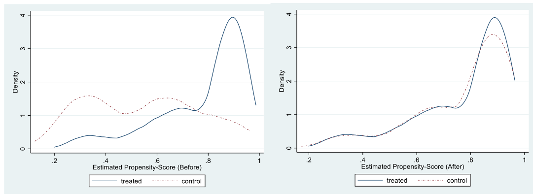
Figure 19. Kernel Density Estimates of Propensity Score Distributions (Second model with Financial Conditions)
