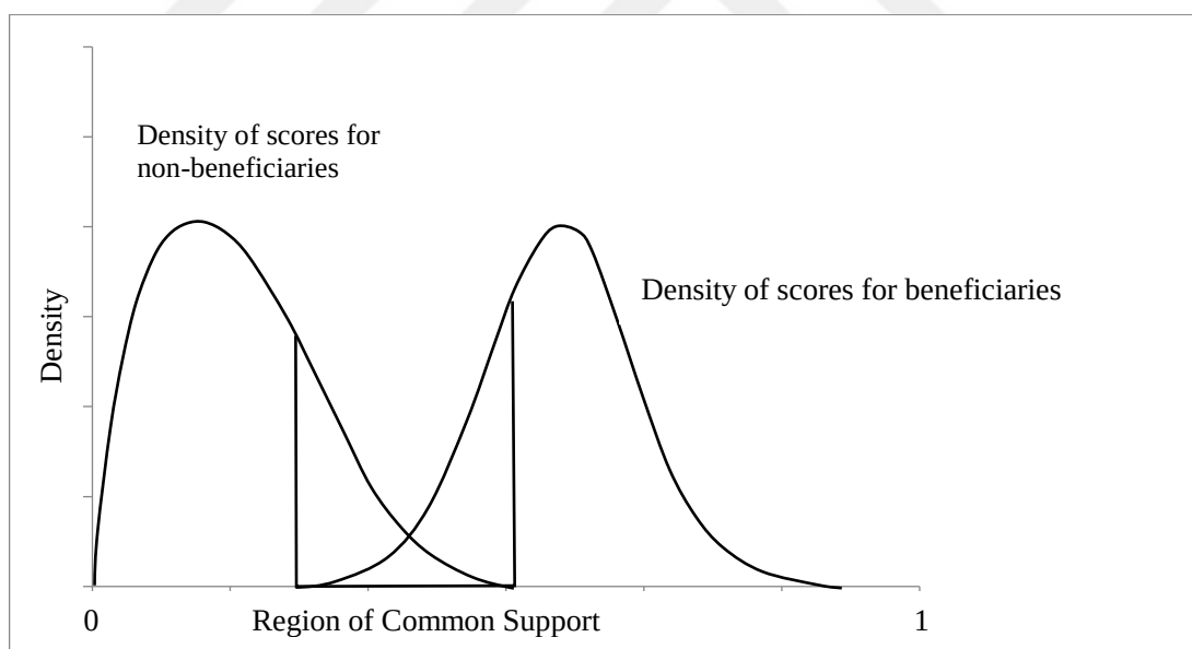
Figure 15. Example of The Poor Common Support Case (Source: Khandker et al., 2010, “Handbook on Impact Evaluation: Quantitative Methods and Practices”, p.57)
