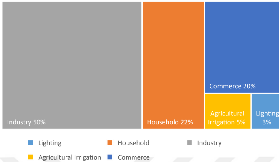
Figure 3.5. Electricity consumption of Kayseri by Consumer (EPDK, 2020)
