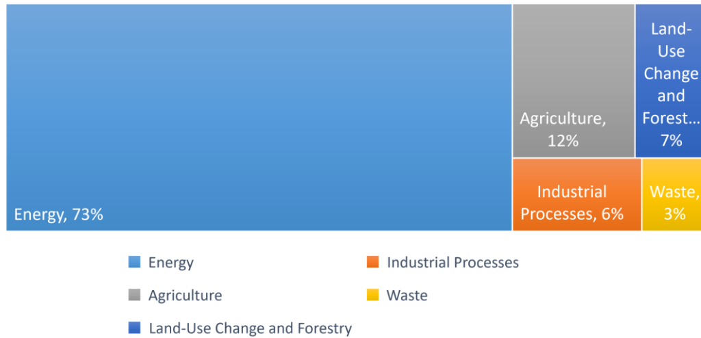
Figure 3.1. Global Greenhouse Gas Emissions by Sectors (Climate Watch, n.d.)
