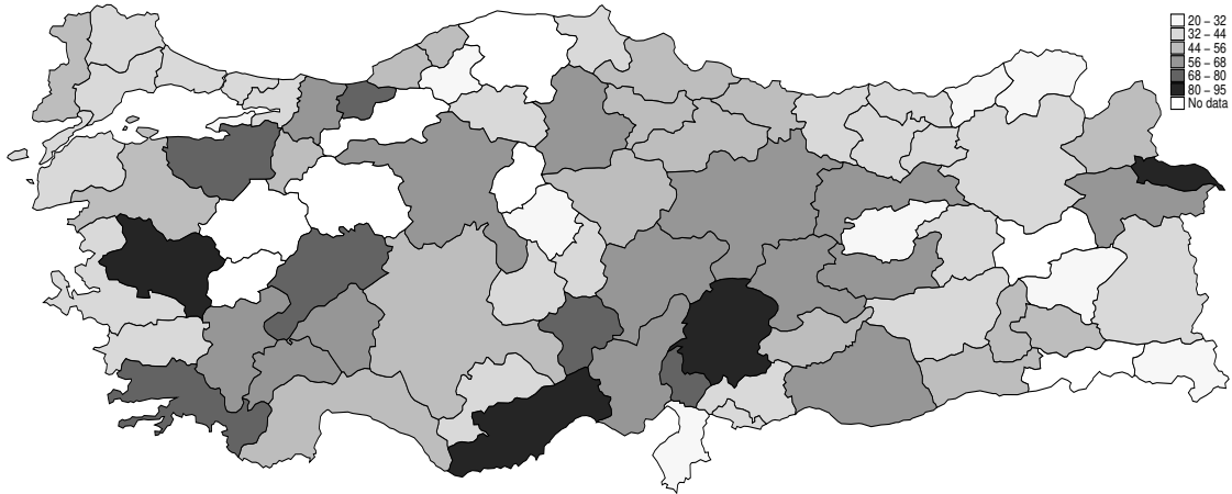
Figure 3.7 PM_{10} levels, 2018
