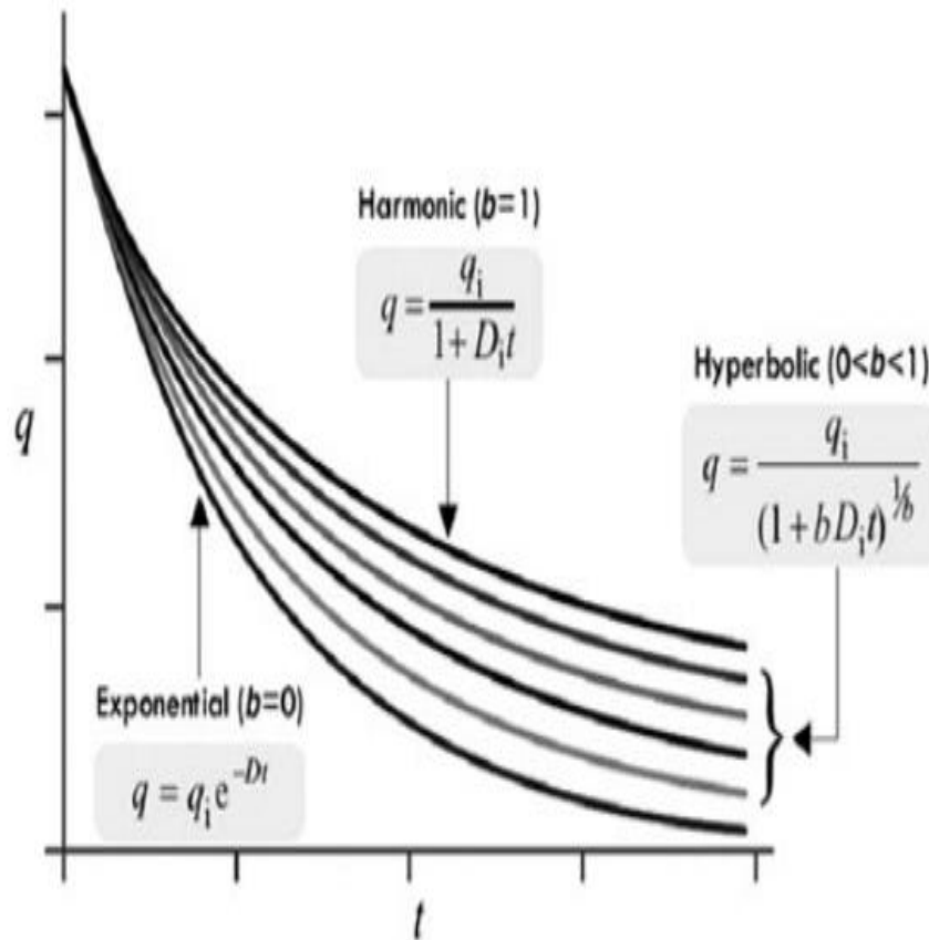
Figure 4.1 Comparison of Exponential, Hyperbolic, and Harmonic Relations (Shin et al., 2014)
