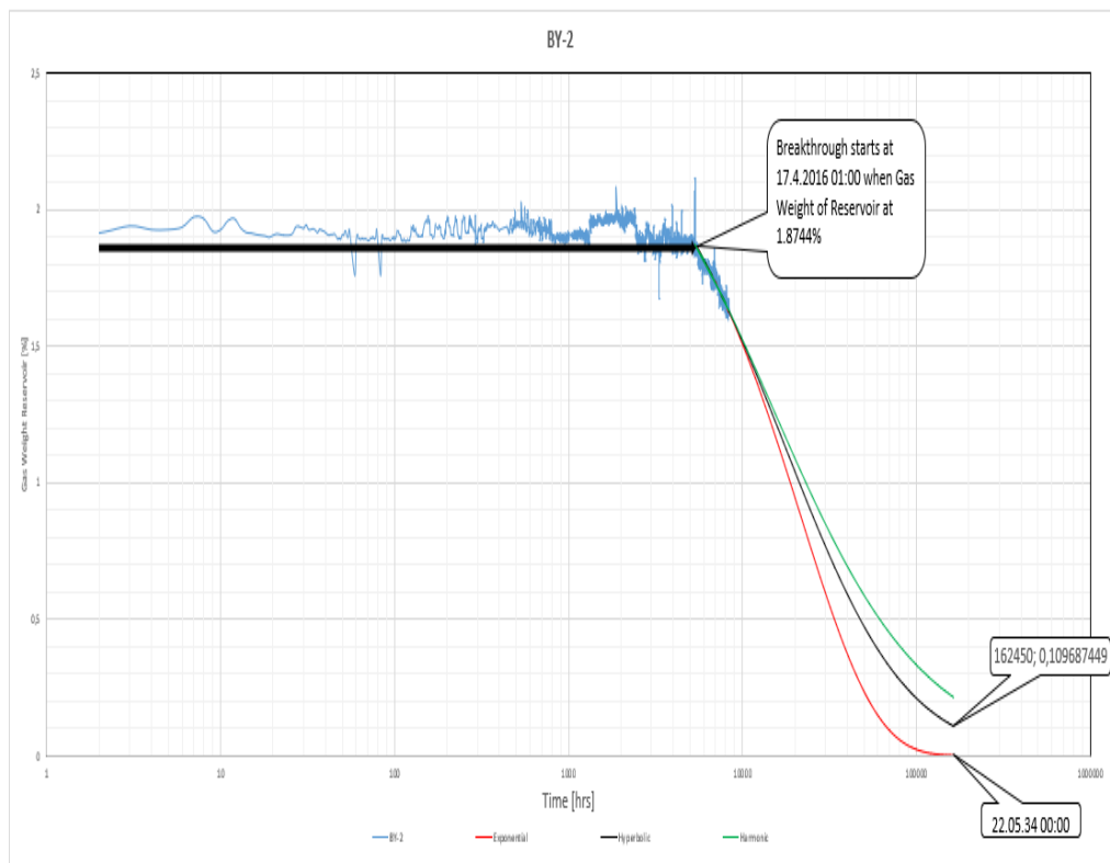
Figure 6.6 Semi-log Analysis of Well BY-2
