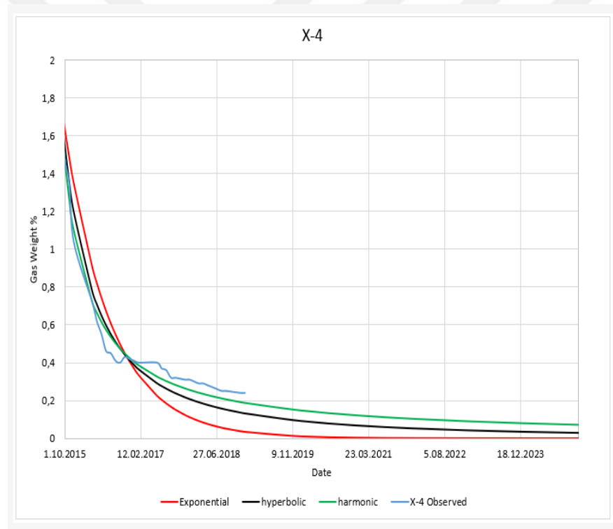
Figure 6.10 Decline Curve Analysis of Well X-4
