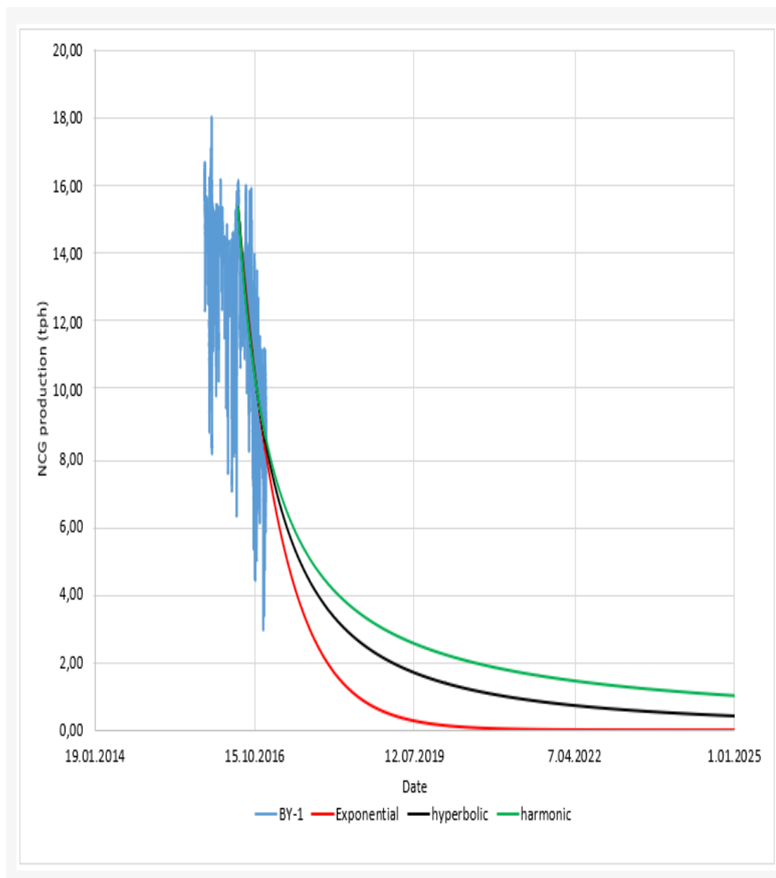
Figure 6.2 Decline Curve Analysis of Well BY-1
