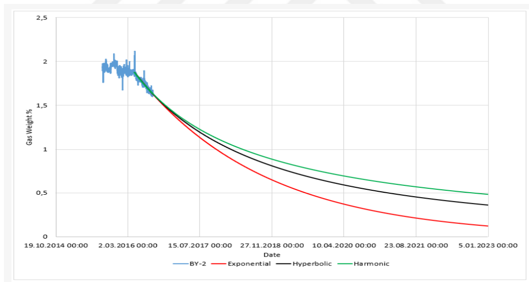
Figure 6.5 Decline Curve Analysis of Well BY-2
