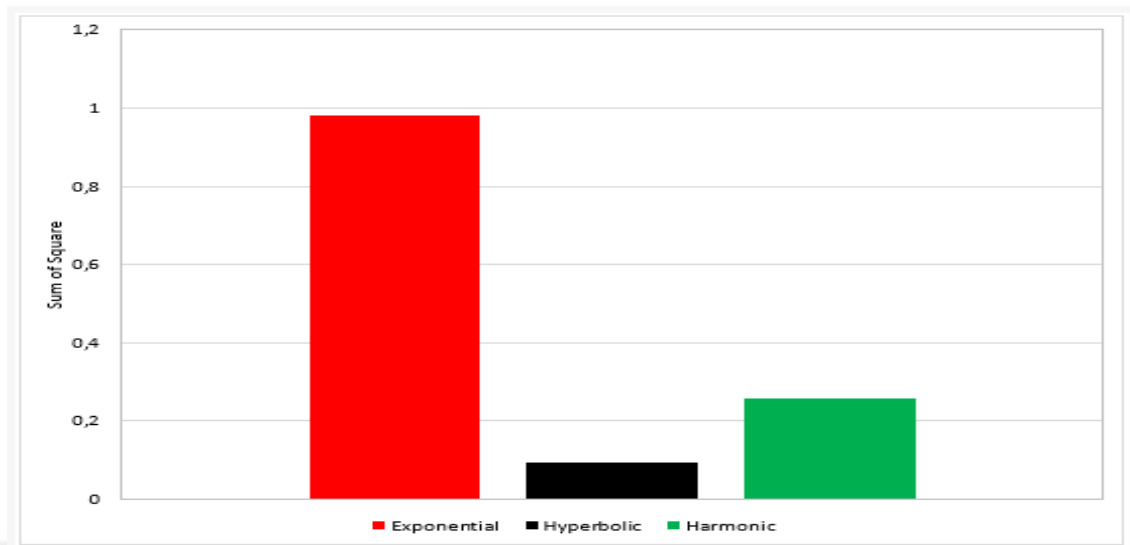
Figure 6.11 Sum of Square Bar Chart for X-4 Well
