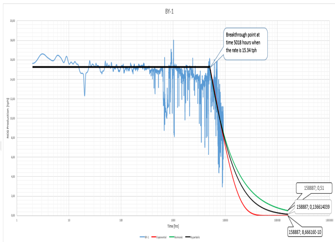
Figure 6.3 Semi-log Analysis of Well BY-1
