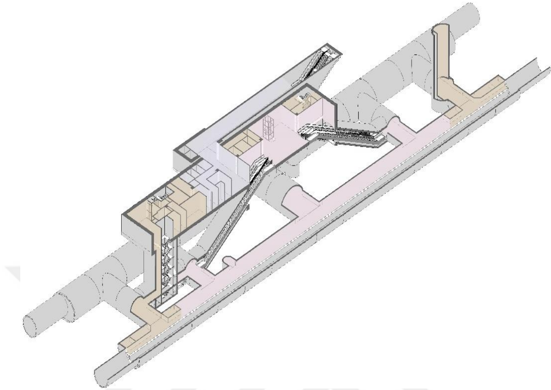
Figure 17. Mixed Type Metro Station (Yüksel Proje, 2016).
