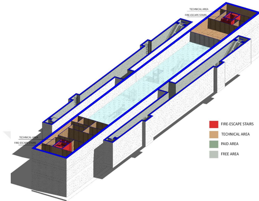
Figure 25. Functional Organization of Technical Floor.
