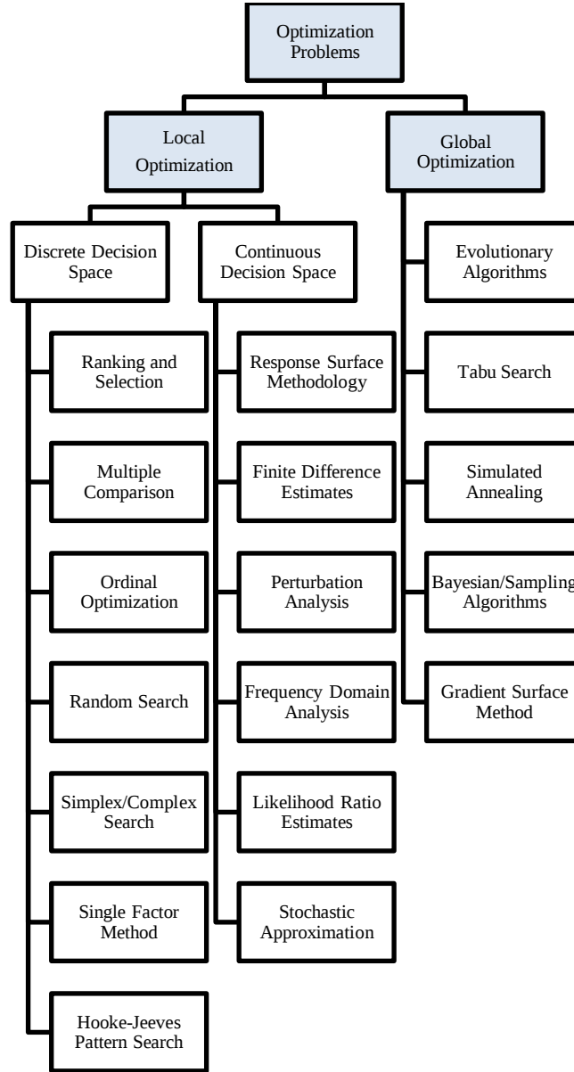
Figure 3: Classification Structure for Simulation Optimization Problems (adapted from [24])
