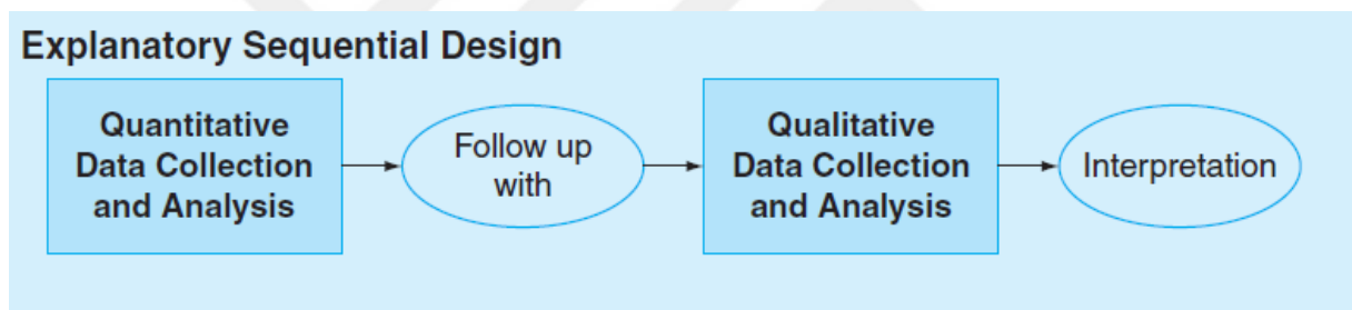
Figure 3.1. The Explanatory Sequential Design of the Present Study (Creswell, 2012, p. 541)
