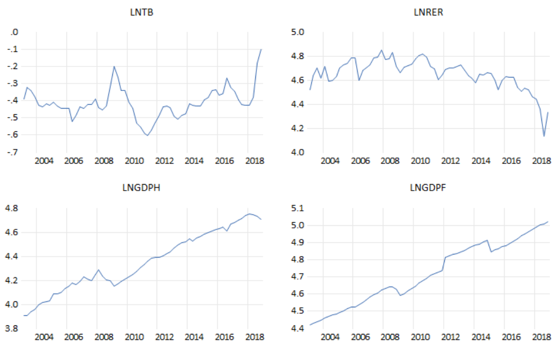
Figure 3.1. Graph of Series Level for Model 1
