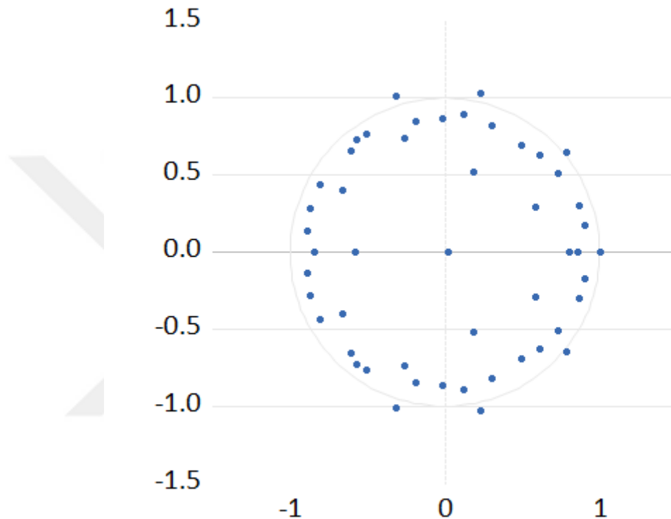
Figure 3.17 Inverse Roots of AR Characteristic Polynomial for Model 3
