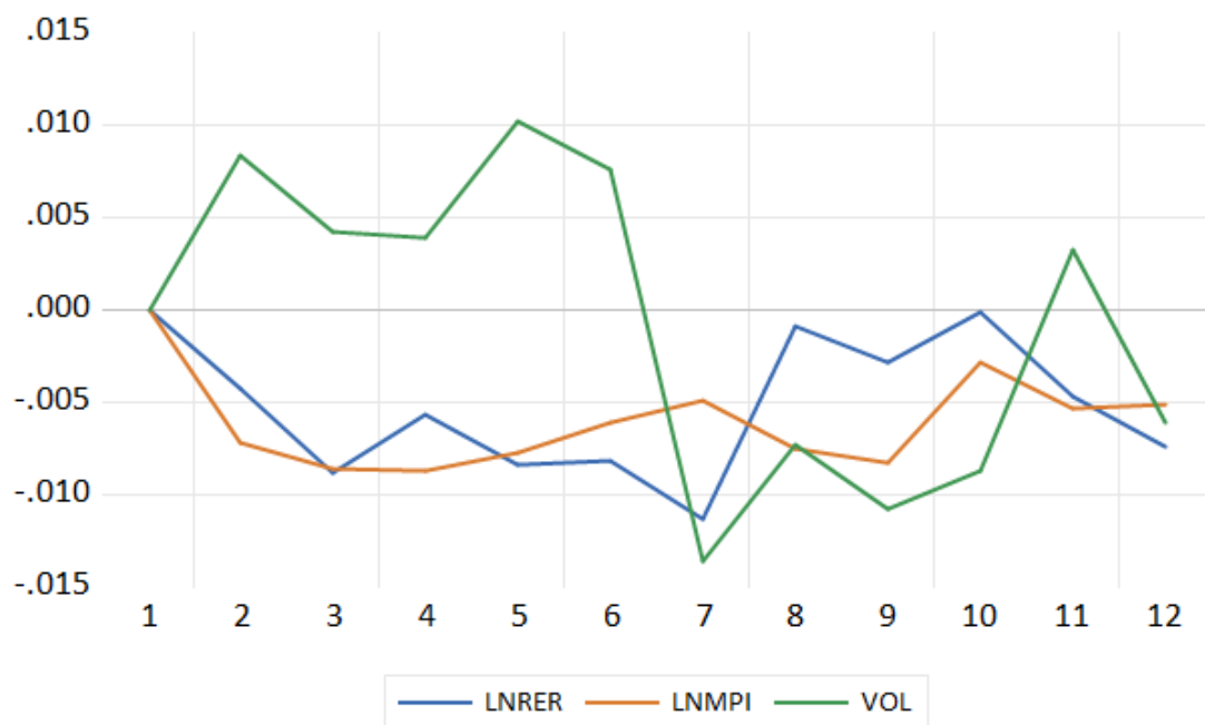
Figure 3.16 Impulse-Response Graphs for Model 3
