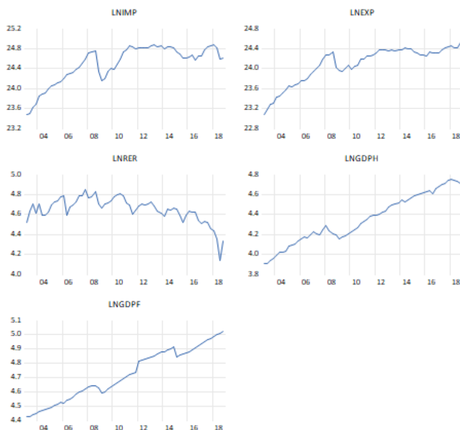
Figure 3.9 Graph of Series Level for Model 2
