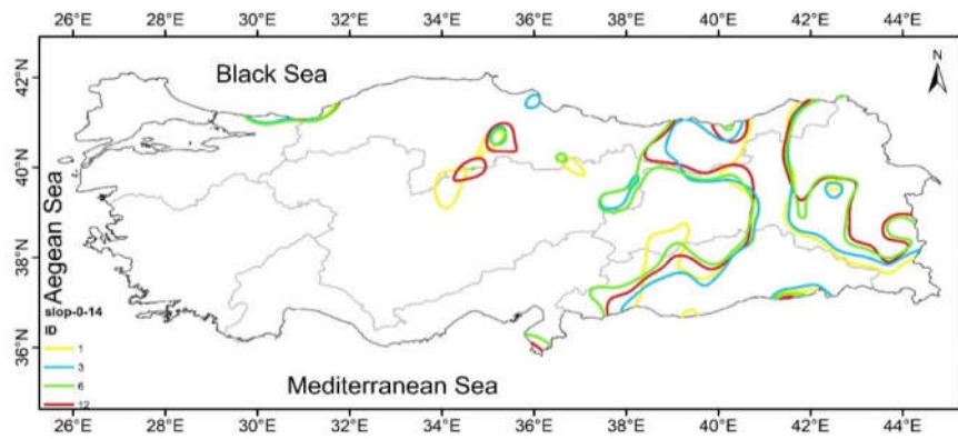
Figure 3.12. The zero-value Contour lines of the Theil-Sen test for the 1982–2015 period showing how they shift according to the time-scal
