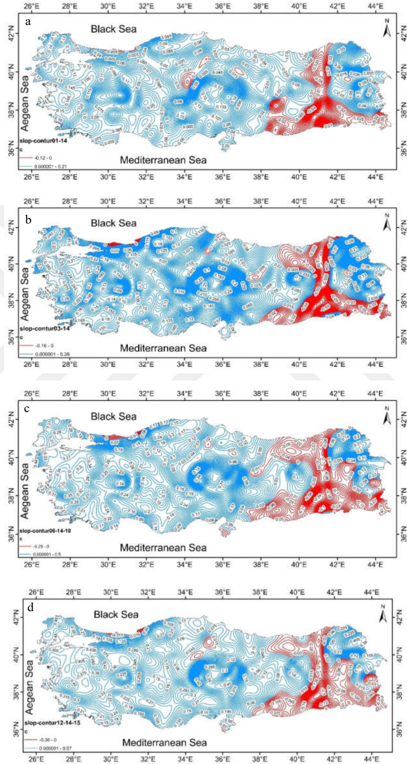
Figure 3.10. Contour lines for the spatial distribution of the Theil-Sen test slope values ( \times 10^{-2} ) of the SPEI trend test data for the 1982–2015 period (a: 1-month, b: 3-month, c: 6-month, d: 12-month).
