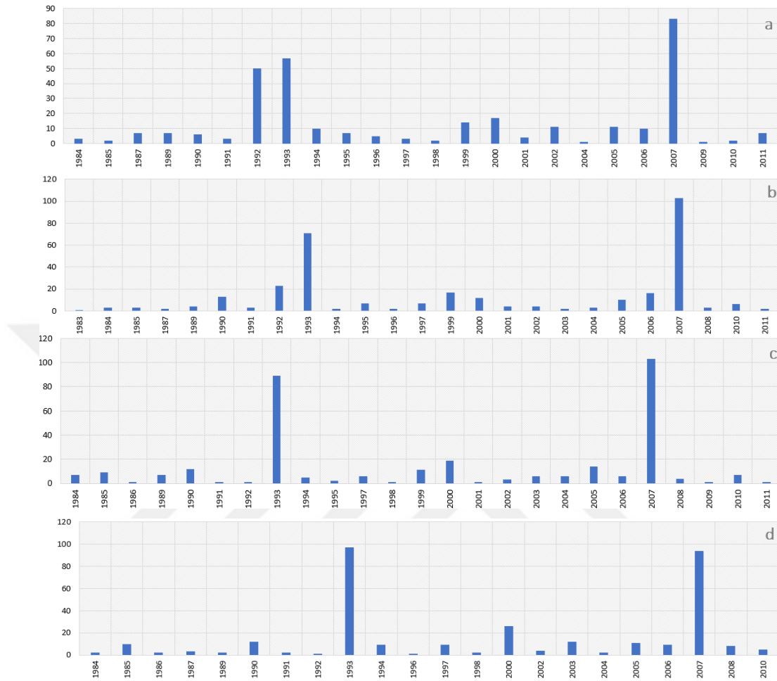
Figure 3.11. Results of the Pettitt's test on SPEI trend test data for the 1982–2015 period).
