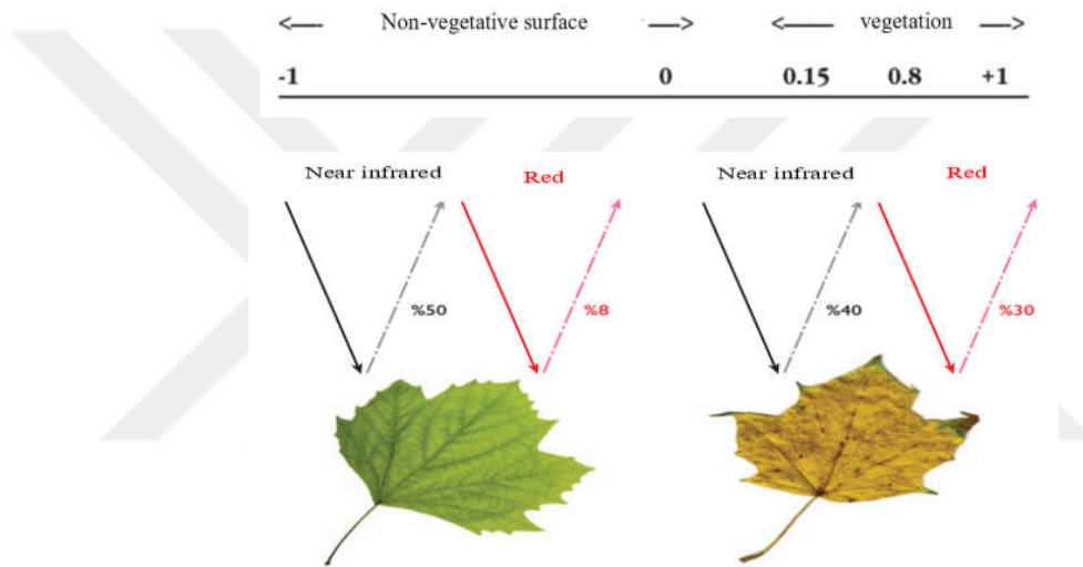
Figure 2.4. Values of NDVI for different leaf reflectors(Sunar Filiz, 2011)
