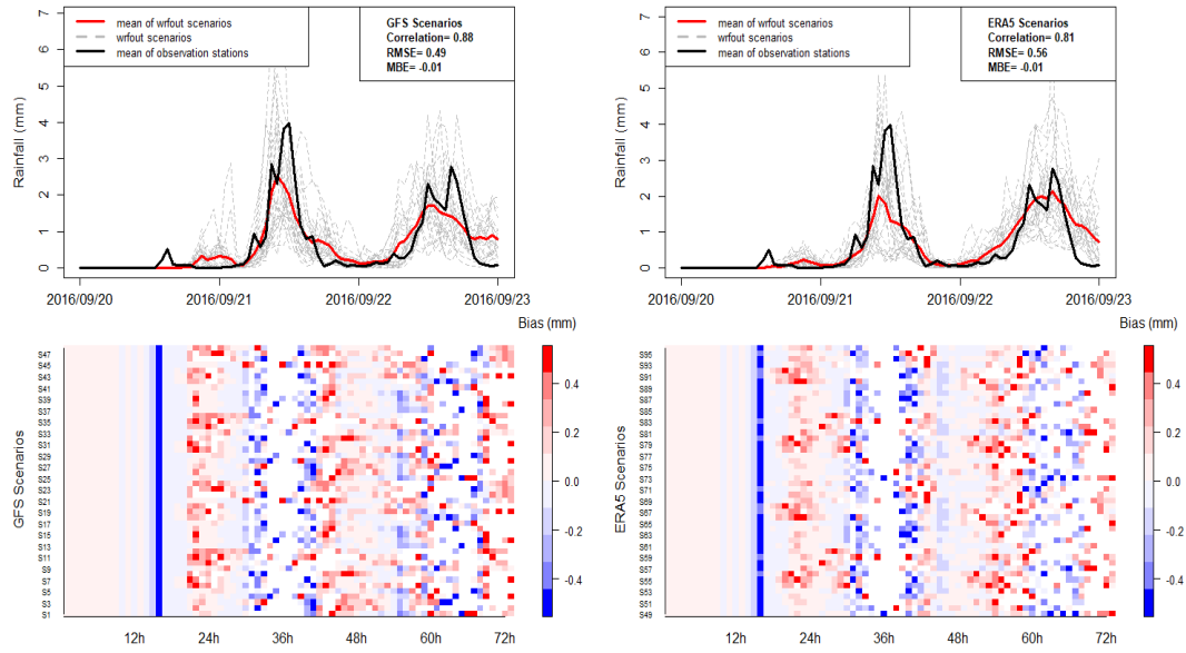
Figure 4.5.2 Average precipitation and bias raster plots of observation and model forecasts throughout the run period. The dashed gray lines represent the each model prediction scenario while the red line indicates the mean of these model scenarios and the solid black line shows the mean of observed precipitation regime in 3 days. The left column illustrates the results for GFS source used model predictions, the right column demonstrates the ERA5 source used model predictions
