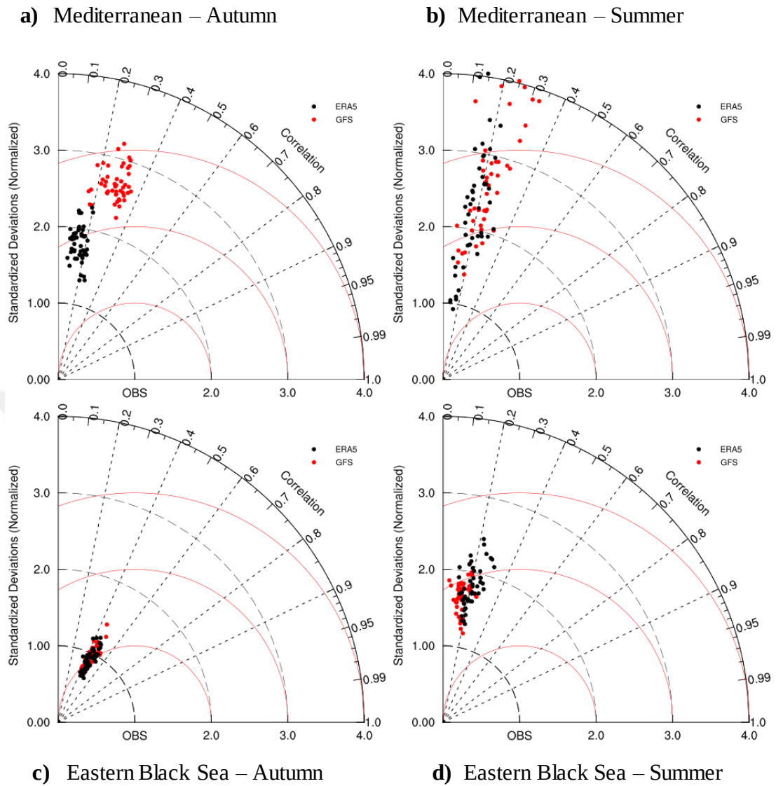
Figure 4.6.4 Taylor Diagrams of the model scenarios according to the input meteorological sources they use in each event case. The scenarios worked with the datasets: ERA5 Reanalysis by black and GFS by red dots, have shown on the graphs
