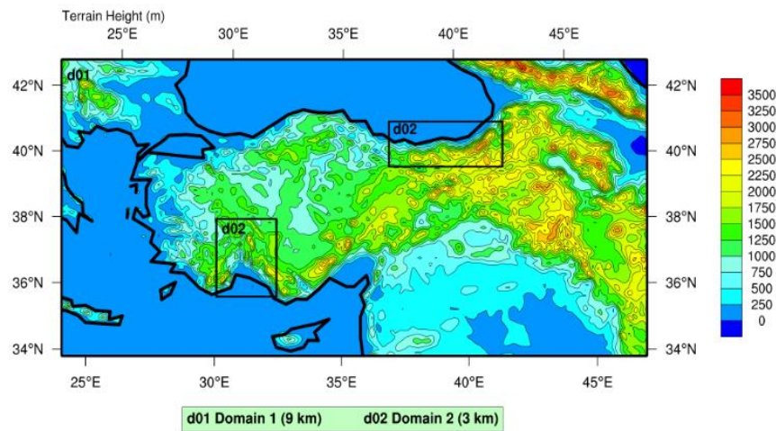
Figure 3.3.1 The representation of determined domains to be used in WRF model configuration for each region. d01 at the top left corner, represents Domain 1 with 9 km grid size (common for both Mediterranean and Eastern Black Sea regions), d02 indicates Domain 2 with 3 km grid size for each region, respectively
