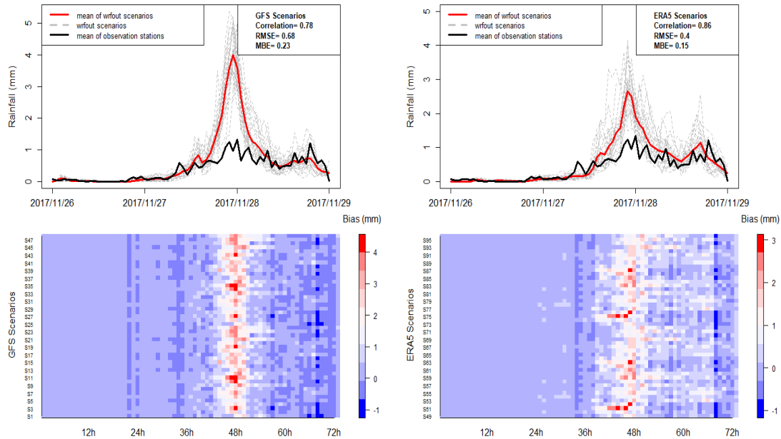
Figure 4.2.2 Average precipitation and bias raster plots of observation and model forecasts throughout the run period. The dashed gray lines represent the each model prediction scenario while the red line indicates the mean of these model scenarios and the solid black line shows the mean of observed precipitation regime in 3 days. The left column illustrates the results for GFS source used model predictions, the right column demonstrates the ERA5 source used model predictions
