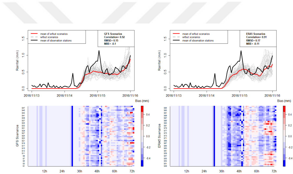
Figure 4.4.2 Average precipitation and bias raster plots of observation and model forecasts throughout the run period. The dashed gray lines represent the each model prediction scenario while the red line indicates the mean of these model scenarios and the solid black line shows the mean of observed precipitation regime in 3 days. The left column illustrates the results for GFS source used model predictions, the right column demonstrates the ERA5 source used model predictions
