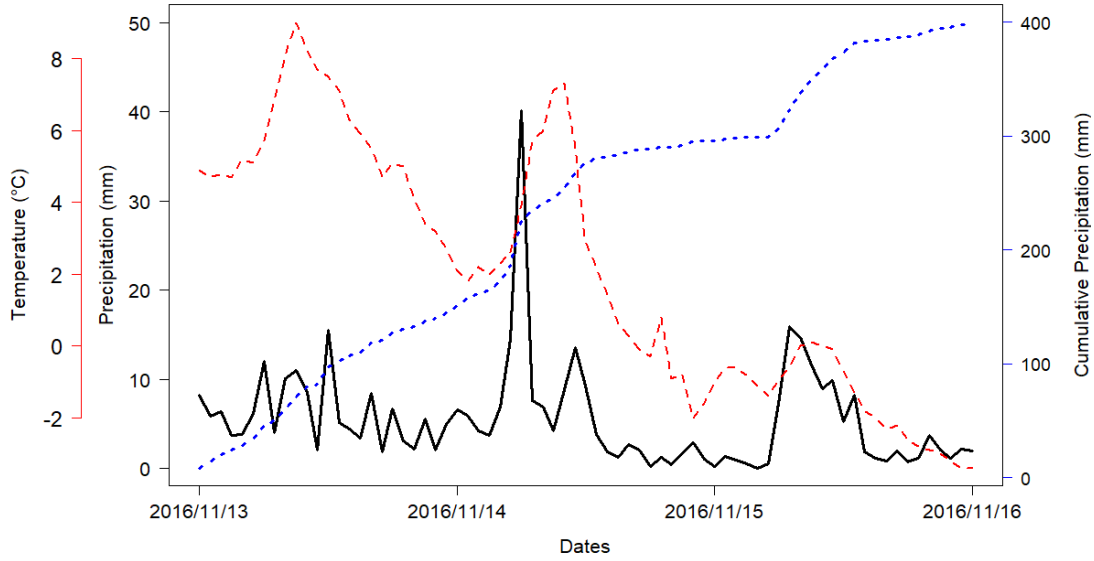
Figure 4.4.1 Precipitation and Temperature time series of the main station (Camlihemsin – Rize) for Eastern Black Sea – Autumn event through the model run period between 2016/11/13 – 2016/11/16. Black solid line refer precipitation amounts dropped over the station while the dashed red line indicates recorded temperature of the station. Dashed blue line represents the cumulative precipitation amounts through the time
