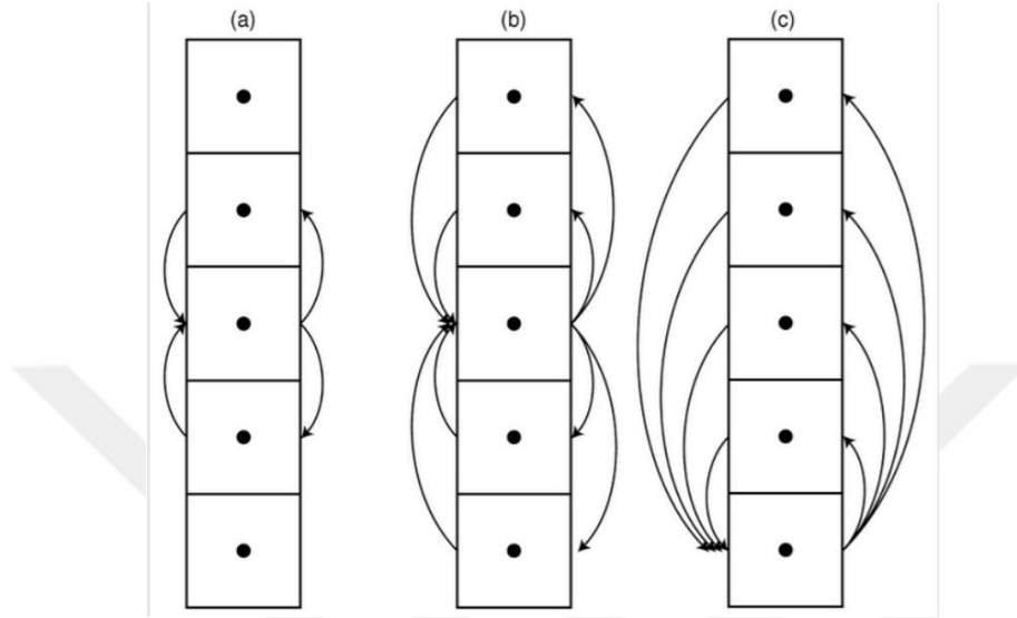
Figure 3.2.7 Representation of the mechanics of the local and non-local closures a) interactions in local closures b) and c) interactions in non-local closures
