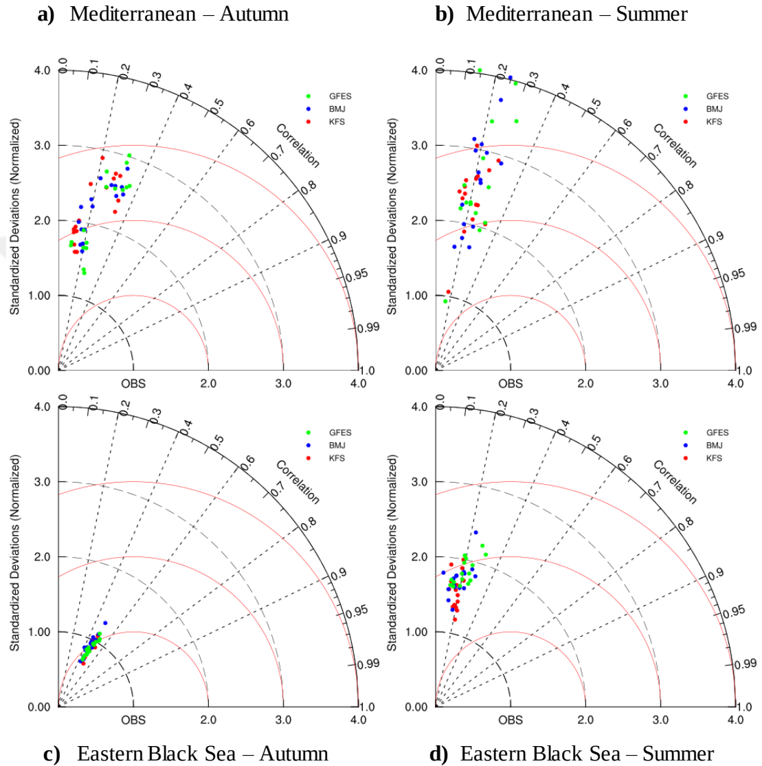
Figure 4.6.2 Taylor Diagrams of the model scenarios according to the cumulus schemes they use in each event case. The scenarios worked with the schemes: Grell Freitas (GFES) by green, Betts Miller Janjic (BMJ) by blue, Kain Fritsch (KFS) by red dots, have shown on the graphs
