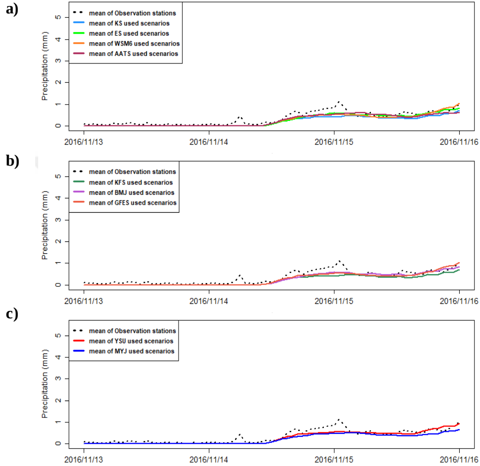
Figure 4.4.7 Variance analysis of the physical parameter schemes based on the observation stations' and model scenarios' precipitation data through the run period of autumn event of Eastern Black Sea region. The dashed black line indicates the observed data. The colorful lines in each plot, refer the model precipitation patterns according to the schemes they used. The plots: a,b and c are prepared to represent the scenario performances on microphysics, cumulus and PBL physics, respectively
