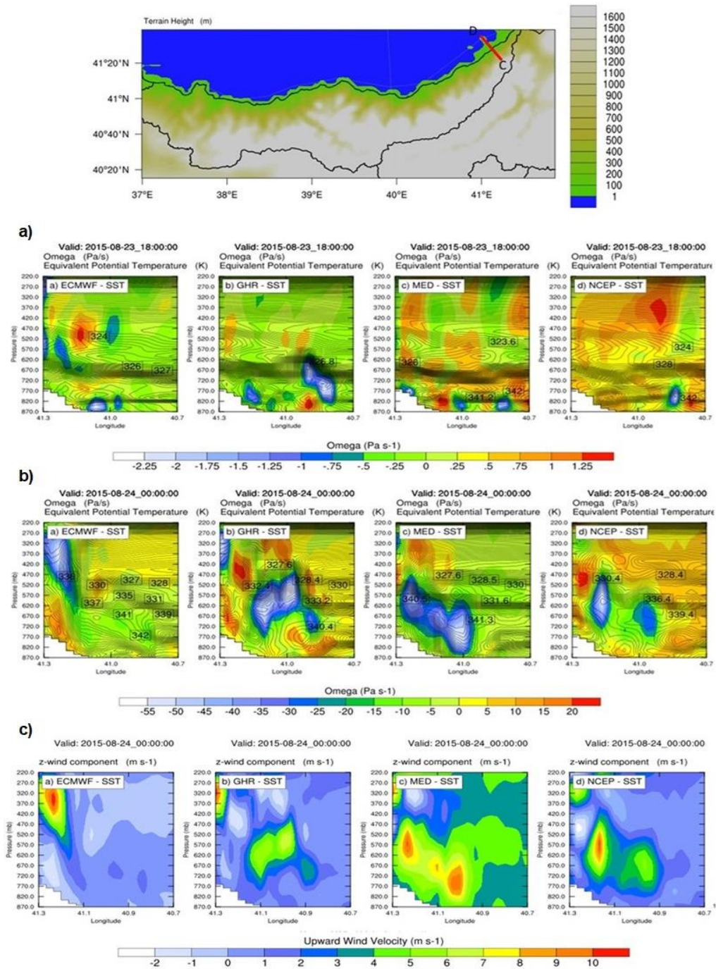
Figure 4.8.7 2015.08.17_00:00:00 – 2015.08.27_00:00:00 run period. The map at the top, shows the location and the terrain height that the CD line covers, the rest demonstrates the model forecasts by the vertical profile of atmosphere along CD line.
