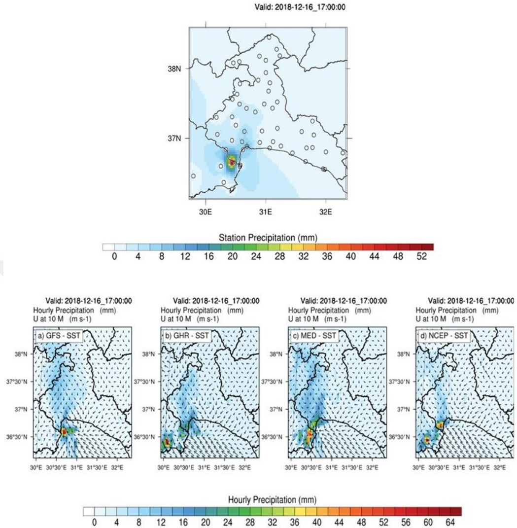
Figure 4.7.4 2018.12.10_00:00:00 – 2018.12.20_00:00:00 run period. The precipitation maps with 3 km horizontal resolution at the peak hour when the highest rain dropped over the Mediterranean region. The map at the top shows the stations' precipitation data (m) and their interpolation throughout the whole domain once again for the peak time (17:00 UTC of December 16). The black circles indicate the locations of observation stations and the color scale of label bar determined according to the stations and their interpolated rain data together). The four maps at the bottom refer the WRF model precipitation forecasts (m) for the peak hour by working with different SST data sources: a) GFS, b) GHR SST, c) Medspiration and d) NCEP, respectively. Black colored vectors on each of these maps, demonstrate the wind speed (m/s) vector at 10 m above the ground
