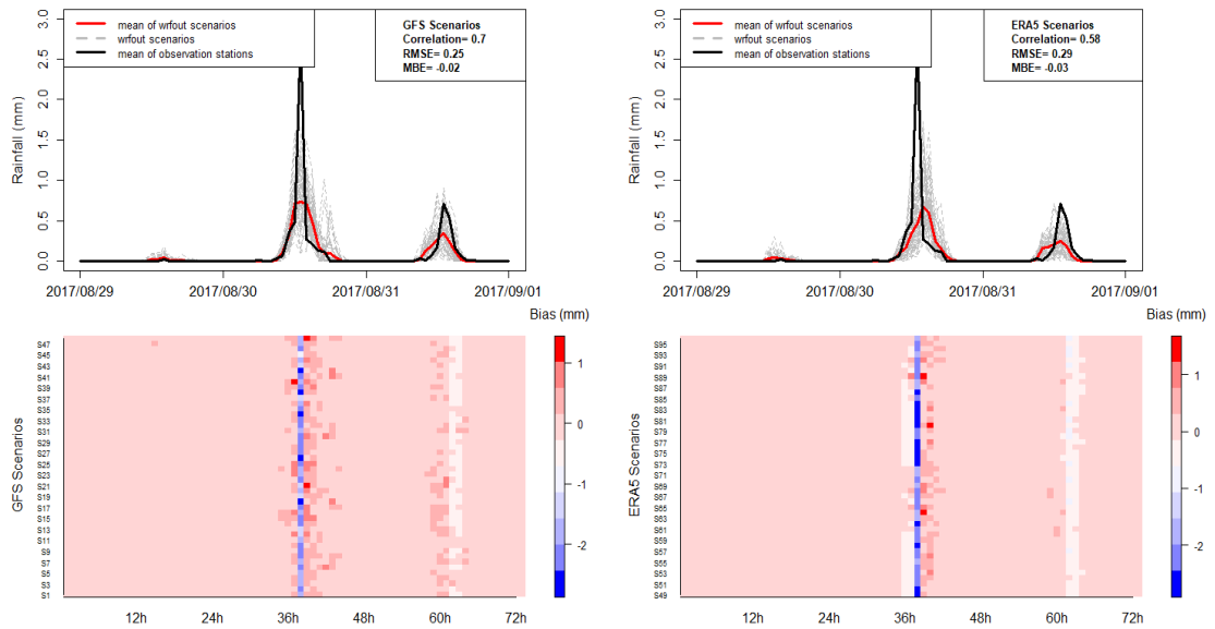
Figure 4.3.2 Average precipitation and bias raster plots of observation and model forecasts throughout the run period. The dashed gray lines represent the each model prediction scenario while the red line indicates the mean of these model scenarios and the solid black line shows the mean of observed precipitation regime in 3 days. The left column illustrates the results for GFS source used model predictions, the right column demonstrates the ERA5 source used model predictions
