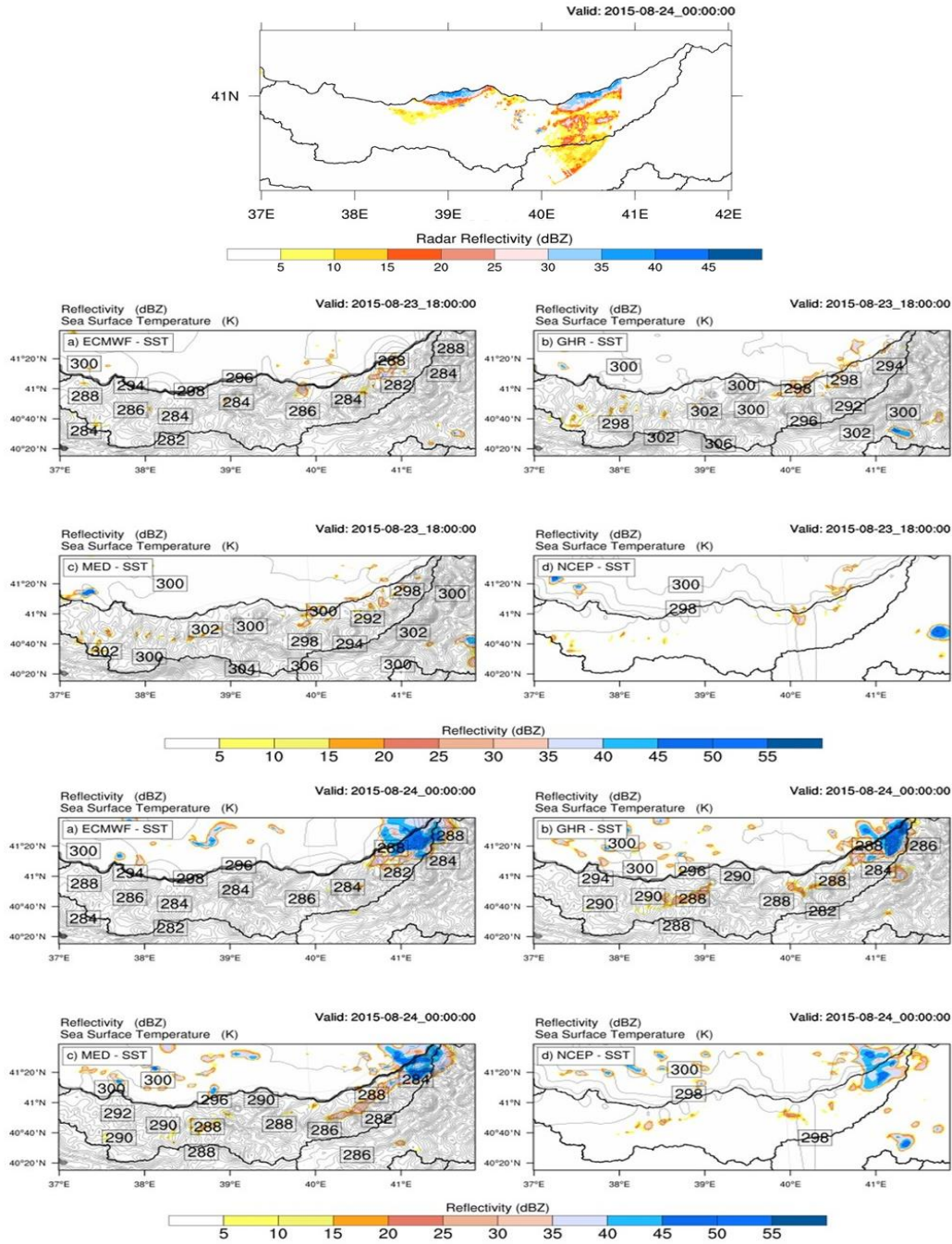
Figure 4.8.5 2015.08.17_00:00:00 – 2015.08.27_00:00:00 run period. The reflection and sea surface temperature (SST) maps with 3 km horizontal resolution of Eastern Black Sea region. The map at the top shows the radar reflectivity data (dBZ) only at the peak hour (00:00 UTC of August 24) whereas the four maps of last two rows refer the WRF model predictions for both at 18:00 UTC and 00:00 UTC to observe the atmospheric evolution within the six hours. The shaded contours represent the reflection (dBZ) and the solid black contours indicate the SST (K). Each map in a row, illustrates the model forecast of the different SST data source: a) GFS, b) GHRSSST, c) Medspiration and d) NCEP, respectively
