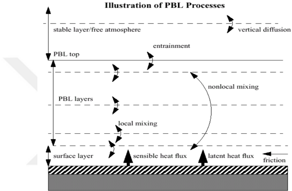
Figure 3.2.6 General Representation of the PBL Interactions and Related Processes (Dudhia, n.d.)
