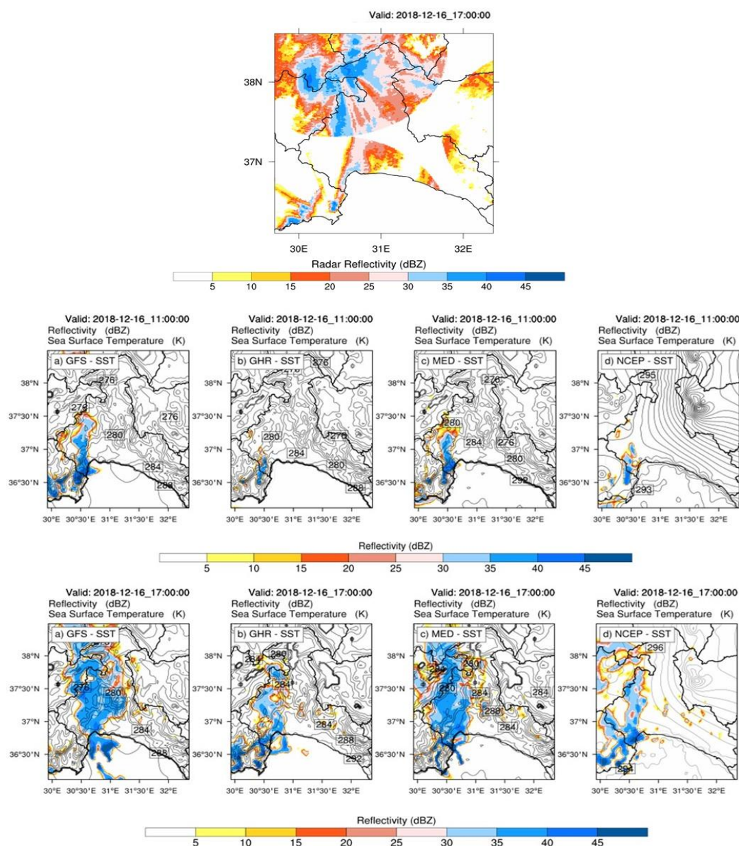
Figure 4.7.5 2018.12.10_00:00:00 – 2018.12.20_00:00:00 run period. The reflection and sea surface temperature (SST) maps with 3 km horizontal resolution of Mediterranean region. The map at the top shows the radar reflectivity data (dBZ) only at the peak hour (17:00 UTC of December 16) whereas the four maps of last two rows refer the WRF model predictions for both at 11:00 UTC and 17:00 UTC to observe the atmospheric evolution within the six hours. The shaded contours represent the reflection (dBZ) and the solid black contours indicate the SST (K). Each map in a row, illustrates the model forecast of the different SST data source: a) GFS, b) GHRSSST, c) Medspiration and d) NCEP, respectively
