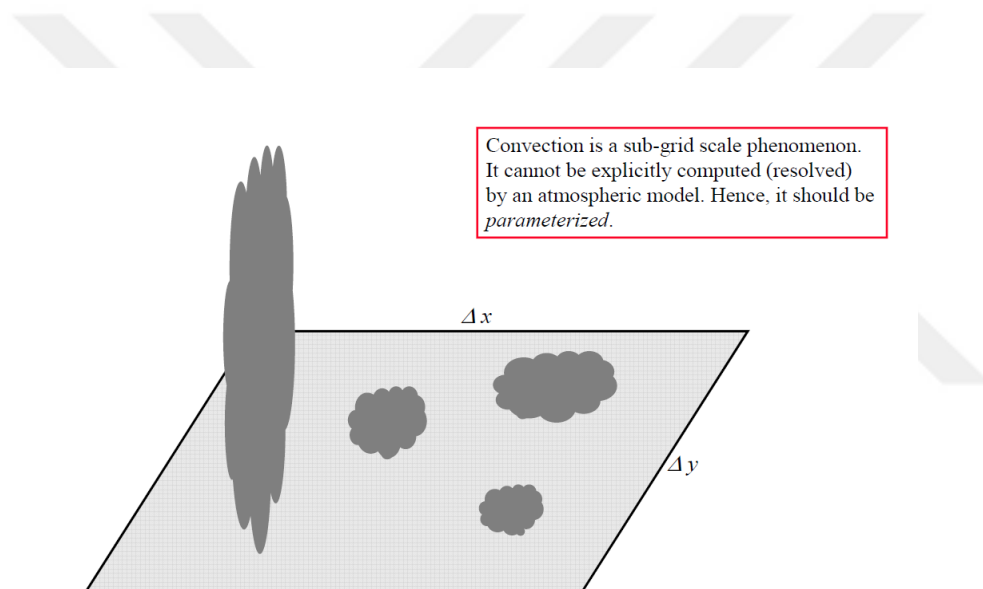
Figure 3.2.2 The need for cumulus parameterization
