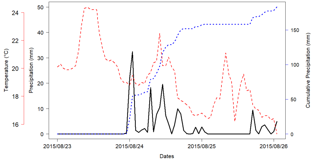
Figure 4.8.1 Precipitation and Temperature time series of the main station (Arhavi – Artvin) for Eastern Black Sea – Summer between 2015/08/23 – 2015/08/26. Black solid line refer precipitation amounts dropped over the station while the dashed red line indicates recorded temperature of the station. Dashed blue line represents the cumulative precipitation amounts through 3 days from total event period
