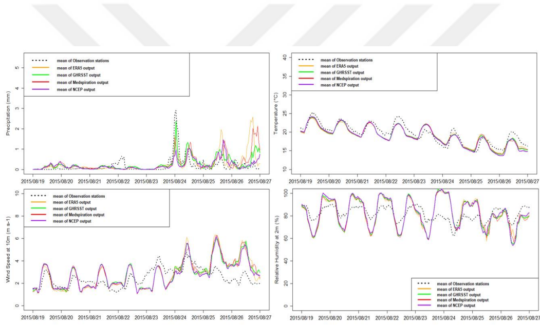
Figure 4.8.2 2015-08-19_00:00:00 – 2015-08-27_00:00:00 run period. The timeseries graphs of observation and SST model forecasts in terms of precipitation (mm), temperature (°C) , wind speed (m/s) and relative humidity (%). The solid colorful lines represent the each model prediction scenario while the dashed black line indicates the mean of observed precipitation regime in 10 days
