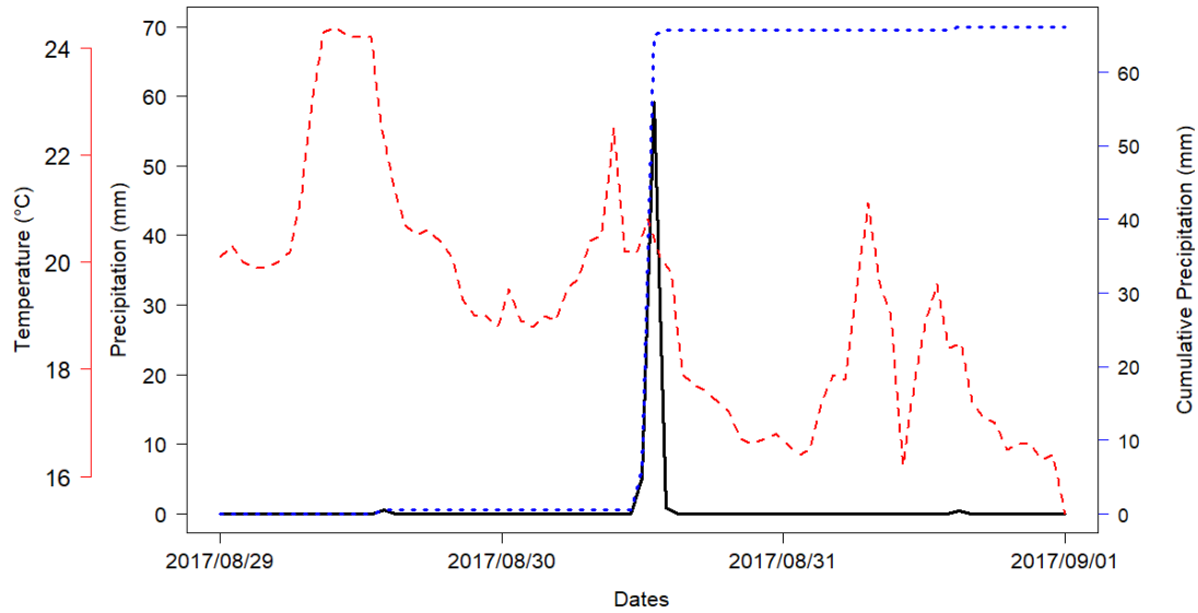
Figure 4.3.1 Precipitation and Temperature time series of the main station (Sutculer – Isparta) for Mediterranean – Summer event through the model run period between 2017/08/29 – 2017/09/01. Black solid line refer precipitation amounts dropped over the station while the dashed red line indicates recorded temperature of the station. Dashed blue line represents the cumulative precipitation amounts through the time
