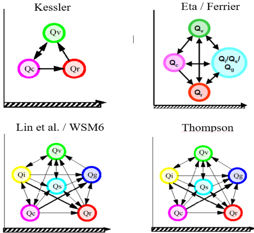
Figure 3.2.5 Microphysics Parameterization Schemes. Mixing ratios Q_v (water vapor), Q_c (cloud water), Q_i (cloud ice), Q_r (rain), Q_s (snow) and Q_g (graupel) are modeled
