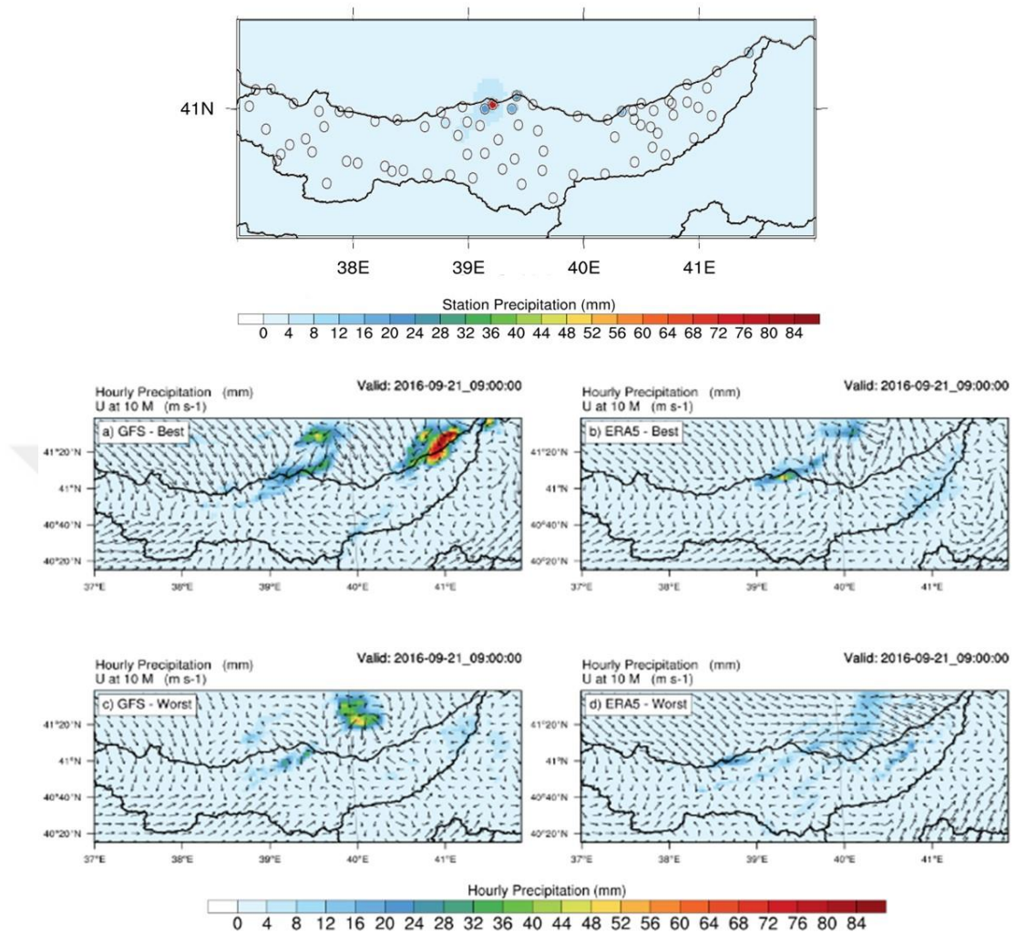
Figure 4.5.4 Precipitation maps of observation and model predictions at the peak hour of Eastern Black Sea summer event (2016.09.21_09:00:00). The map at top illustrates the interpolated station precipitation contours whereas the black circles refer the locations of these stations. The graphs at bottom represent the forecasted precipitation contours and wind speed vectors at 10 m for both best and worst performances of GFS and ERA5 source used scenarios (These scenarios are determined from Table 4.1.4 )
