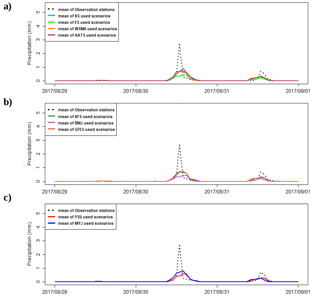
Figure 4.3.6 Variance analysis of the physical parameter schemes based on the observation stations' and model scenarios' precipitation data through the run period of autumn event of Mediterranean region. The dashed black line indicates the observed data. The colorful lines in each plot, refer the model precipitation patterns according to the schemes they used. The plots: a, b and c are prepared to represent the scenario performances on microphysics, cumulus and PBL physics, respectively
