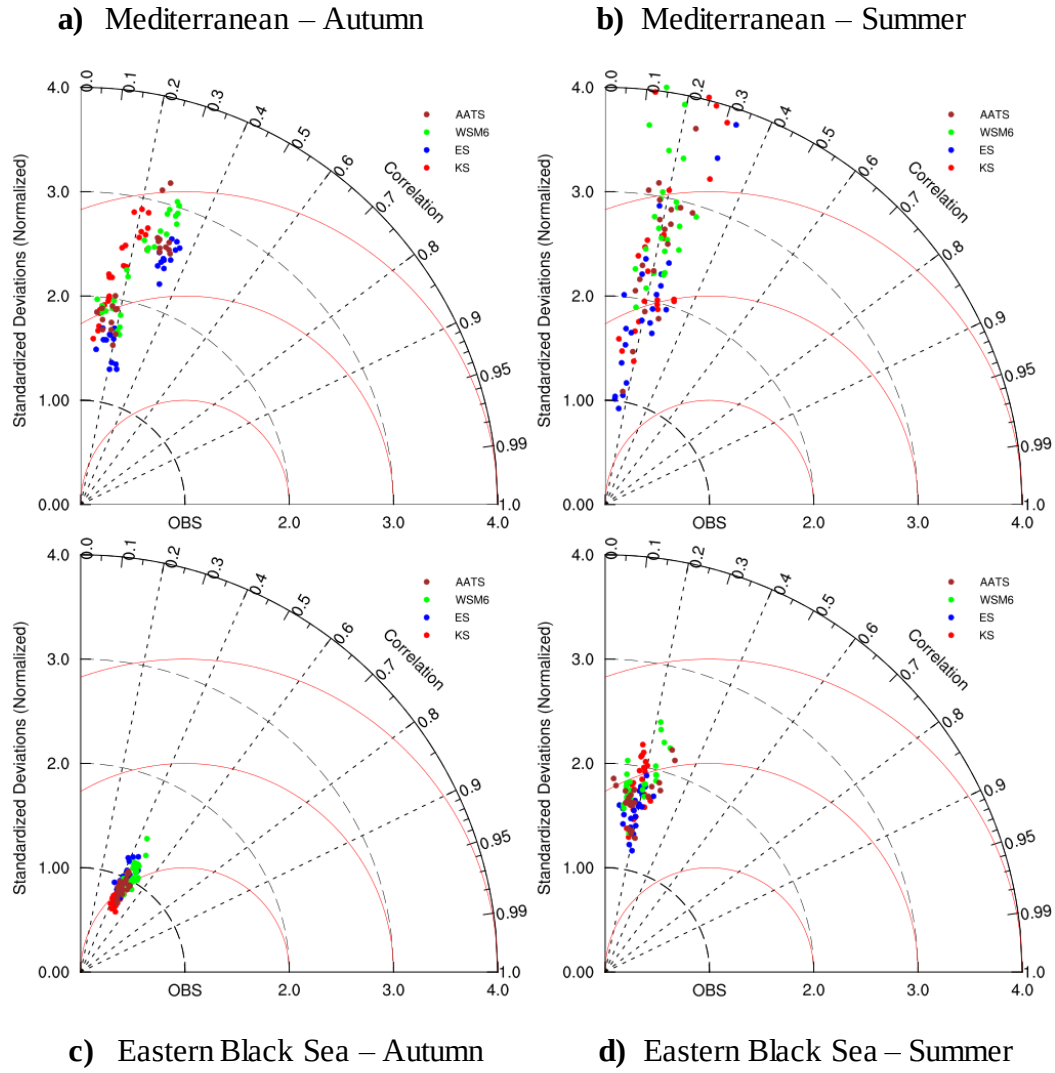
Figure 4.6.1 Taylor Diagrams of the model scenarios according to the microphysics schemes they use in each event case. The scenarios worked with the schemes: Aerosol Aware Thompson (AATS) by burgundy, WRF Single Moment 6 by green, Eta / Ferrier (ES) by blue and lastly Kessler (KS) by red dots, have shown on the graphs
