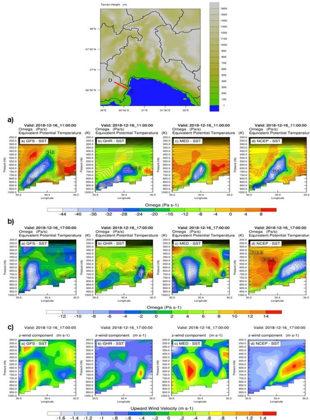
Figure 4.7.7 2018.12.10_00:00:00 – 2018.12.20_00:00:00 run period. The map at the top, shows the location and the terrain height that the CD line covers, the rest demonstrates the model forecasts by the vertical profile of atmosphere along CD line.
