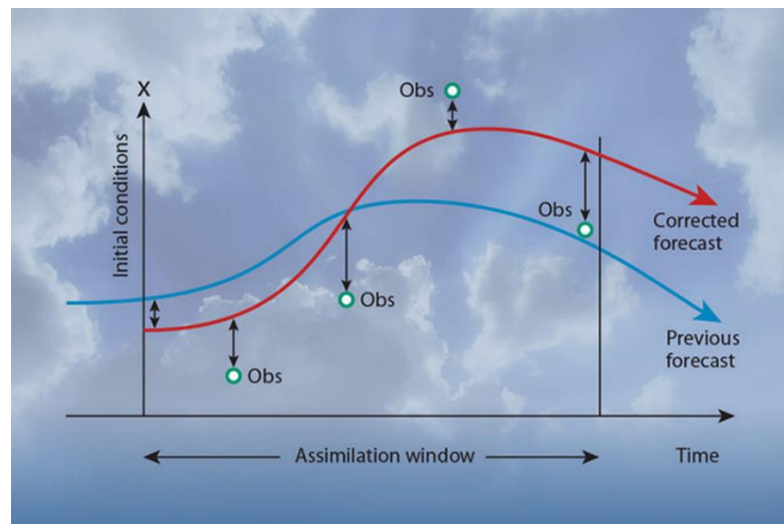
Figure 3.1.1 The mechanism of how ERA5 Reanalysis dataset has obtained by ECMWF (Hersbach et al., 2020)
