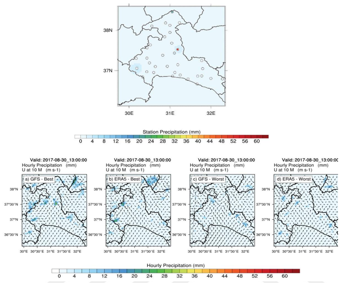
Figure 4.3.4 Precipitation maps of observation and model predictions at peak hour (and also the maximum mean precipitation hour) of Mediterranean summer event (2017.08.30_13:00:00). The map at top illustrates the interpolated station precipitation contours whereas the black circles refer the locations of these stations. The graphs at bottom represent the forecasted precipitation contours and wind speed vectors at 10 m for both best and worst performances of GFS and ERA5 source used scenarios (These scenarios are determined from Table 4.1.4 )
