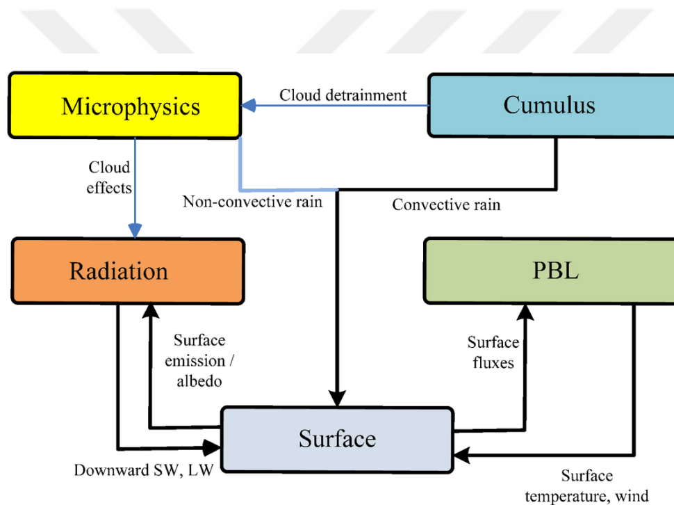
Figure 3.2.3 Main physical components of the atmospheric system and their relations with each other
