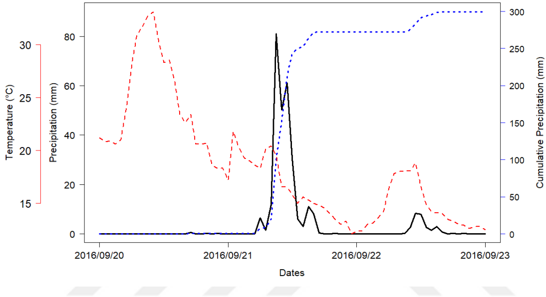
Figure 4.5.1 Precipitation and Temperature time series of the main station (Besikduzu – Trabzon) for Eastern Black Sea – Summer event through the model run period between 2016/09/20 – 2016/09/23. Black solid line refer precipitation amounts dropped over the station while the dashed red line indicates recorded temperature of the station. Dashed blue line represents the cumulative precipitation amounts through the time
