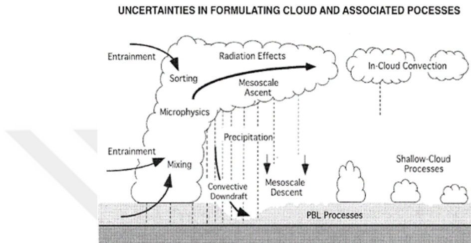
Figure 3.2.1 General Representation of the clouds and their related processes (Arakawa, 2004)
