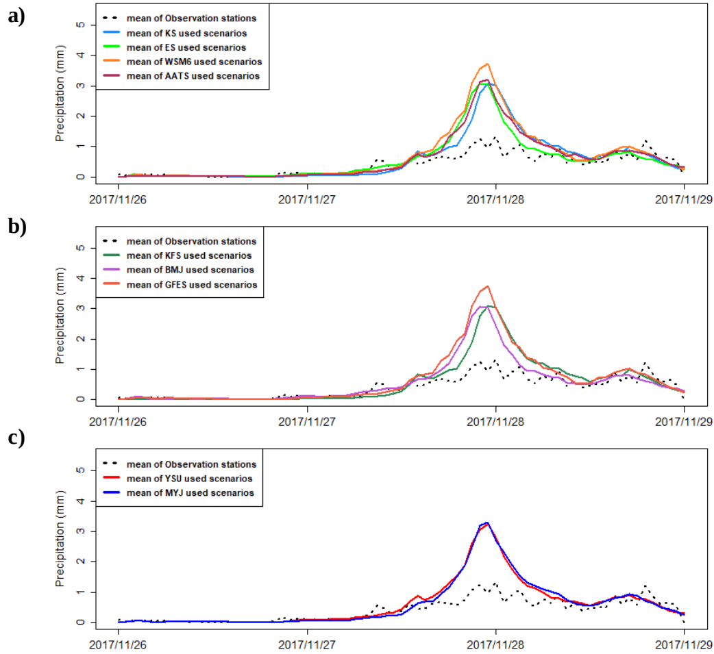
Figure 4.2.7 Variance analysis of the physical parameter schemes based on the observation stations' and model scenarios' precipitation data through the run period of autumn event of Mediterranean region. The dashed black line indicates the observed data. The colorful lines in each plot, refer the model precipitation patterns according to the schemes they used. The plots: a,b and c are prepared to represent the scenario performances on microphysics, cumulus and PBL physics, respectively
