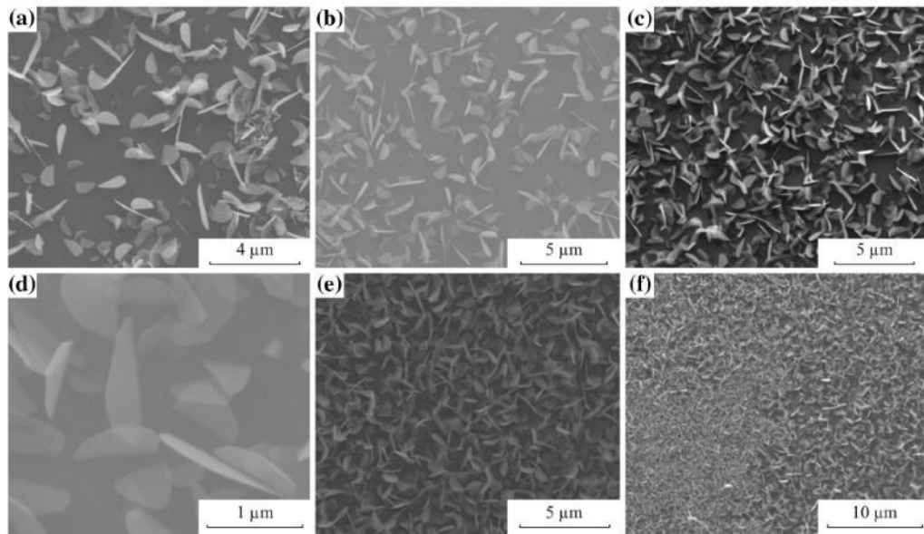
Figure 4-5 SEM Images for CVD MoS 2 when D_s = a) 9 cm, b) 10 cm, c), d) 11 cm, e) 12 cm, and f) 13 cm with a reaction period of 5 minutes [55]
