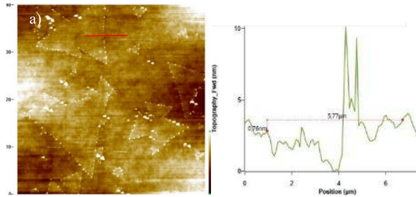
Figure 6-10 AFM measurement of NaCl assisted MoSe 2 flake (thickness=0.76 nm)
