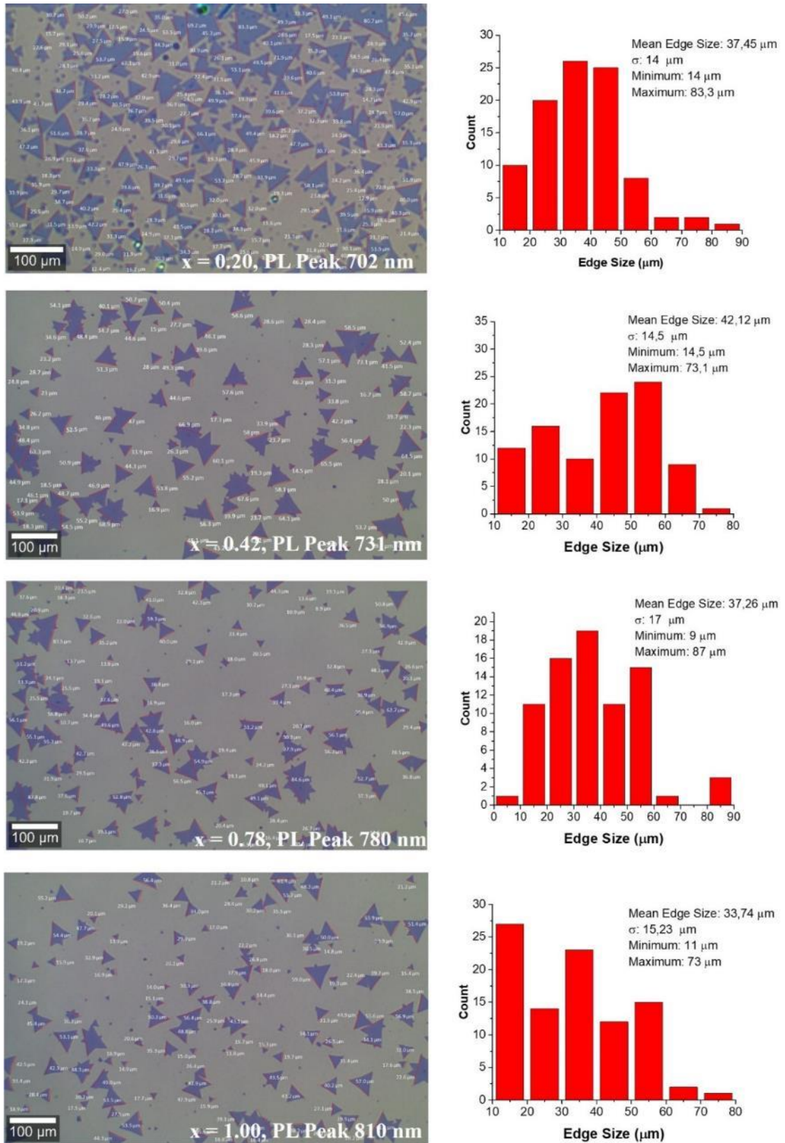
Figure 5-2 Left column is region of interest for the statistical analysis and right column is the frequency count of the flakes' edge size together with mean, standard deviation ( \sigma ) minimum and maximum sizes.
