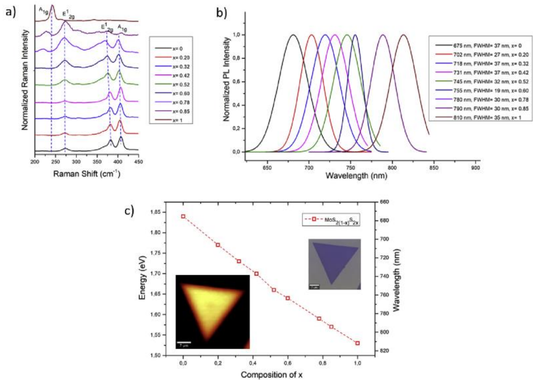
Figure 5-5 a) Raman and b) PL spectra of \text{MoS}_{2(1-x)}\text{Se}_{2x} ( x=0, 0.20, 0.32, 0.42, 0.52, 0.60, 0.78, 0.85, 1 ) flakes. C) PL peak position (nm) versus x value of \text{MoS}_{2(1-x)}\text{Se}_{2x} flakes. Inset: Optical image and PL imaging measurement of x=0.2 [29]
