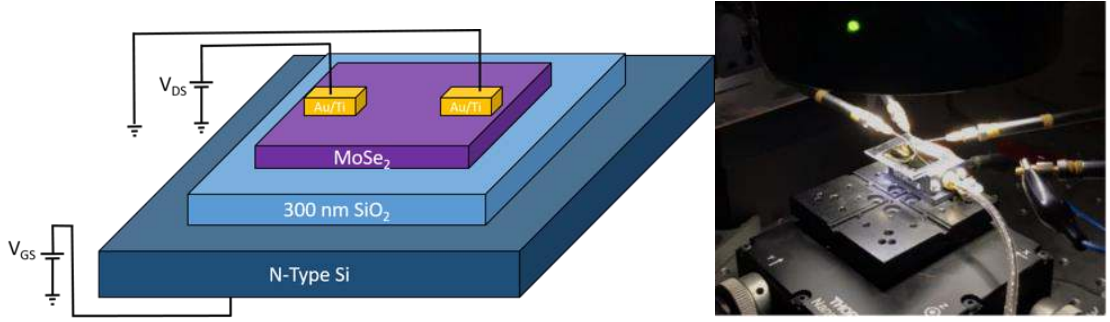
Figure 7-12 a) Back gate configuration of MoSe 2 FET b) Electrical measurements of FET
