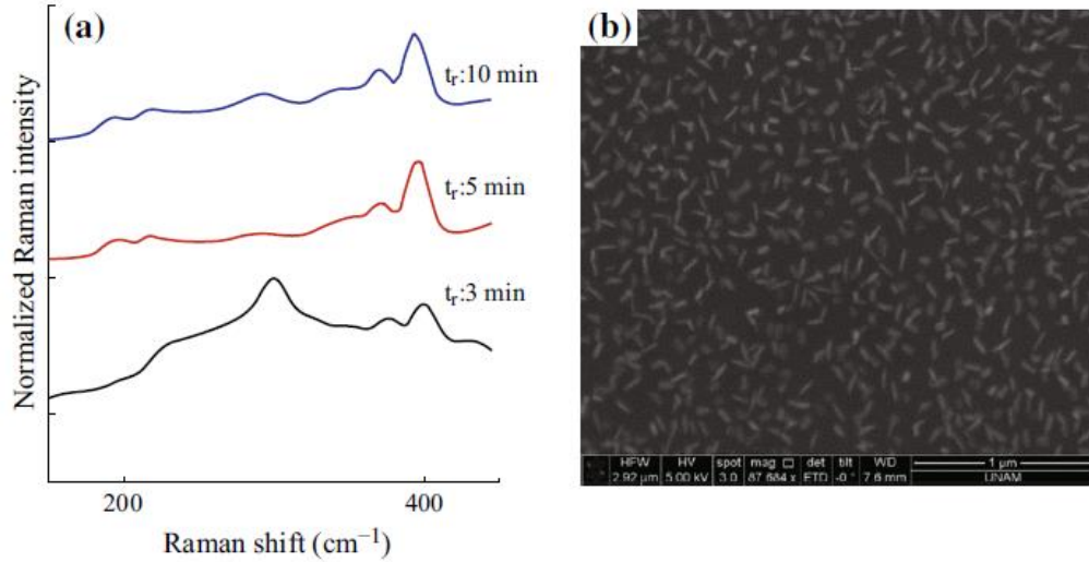
Figure 4-6 a) Raman spectra for CVD \text{MoS}_2 the reaction period is fixed to 3, 5, and 10 minutes when D_S=11 cm; b) SEM image with a reaction period of 3 minutes [55]
