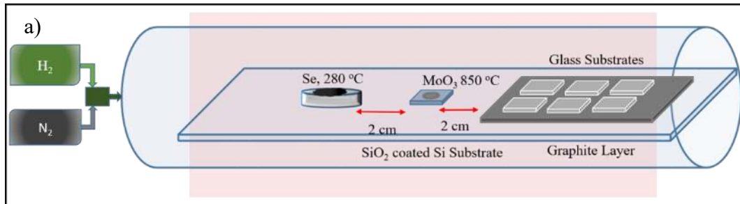
Figure 6-2 CVD scheme for MoSe 2 .Optical image Raman and PL measurements
