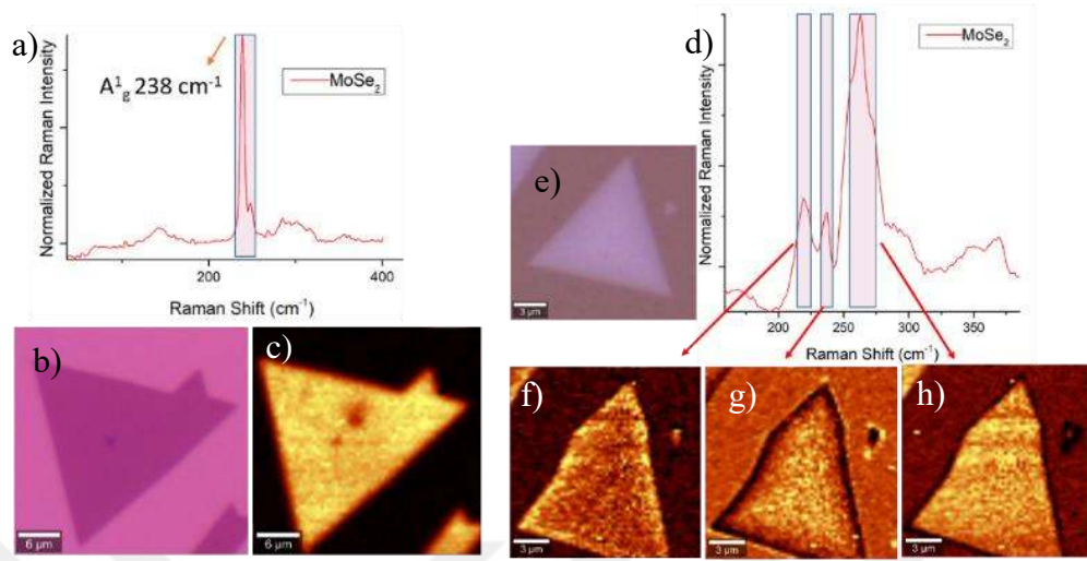
Figure 6-7 a) Raman spectra NaCl salt assisted MoSe 2 . b) Optical image of NaCl salt assisted MoSe 2 . c) Raman imaging of NaCl salt assisted MoSe 2 (centered at 238 cm -1 ). d) Raman spectra of MoSe 2 flakes grown on glass. e) Optical image of MoSe 2 flakes grown on glass. f) Raman imaging of MoSe 2 flakes grown on glass (centered at 220 cm -1 ). g) Raman imaging of MoSe 2 flakes grown on glass (centered at 240 cm -1 ). h) Raman imaging of MoSe 2 flakes grown on glass (centered at 270 cm -1 ).
