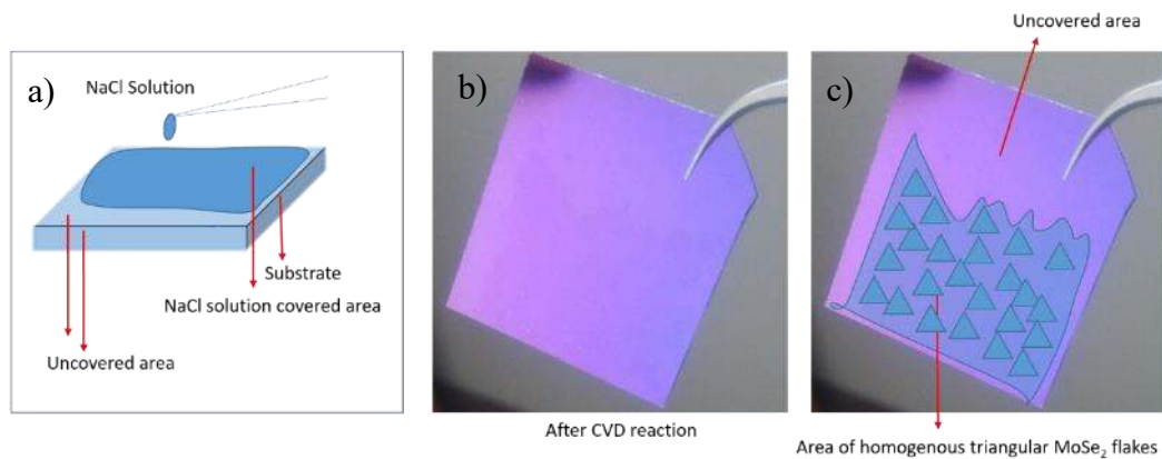
Figure 6-8 a) Demonstration of NaCl solution on SiO 2 substrate b) SiO 2 substrate after CVD growth c) Demonstration of growth location
