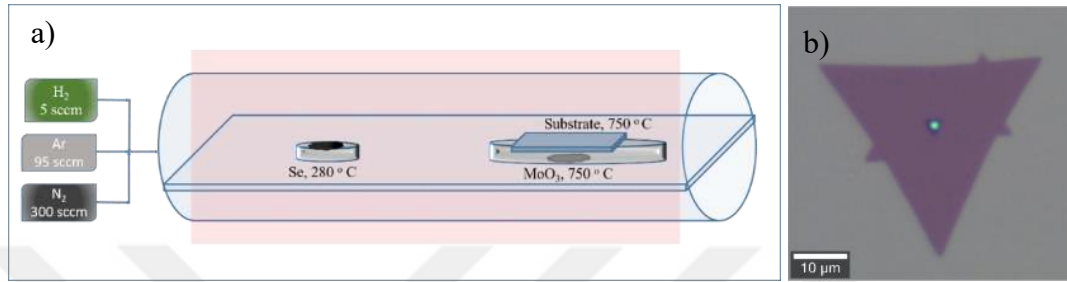
Figure 6-1 a) CVD scheme for MoSe 2 b) Optical image of the largest produced MoSe 2 by flake face down configuration
