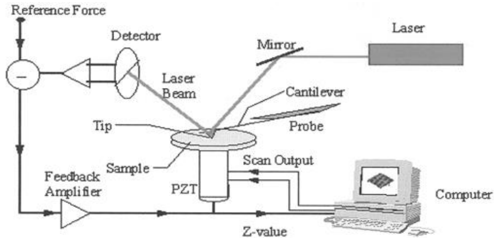
Figure 2-12 AFM scheme [71]
