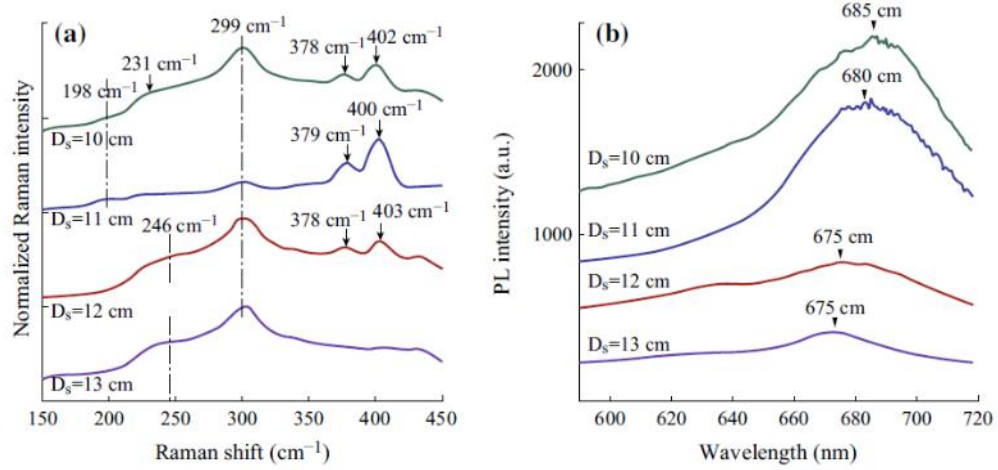
Figure 4-2 a) Raman scattering spectra and b) PL spectra of \text{MoS}_2 the reaction period is 10 minutes [55]
