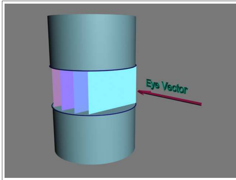
Figure 5.3: Slicing between the contours of a generalized cylinder
