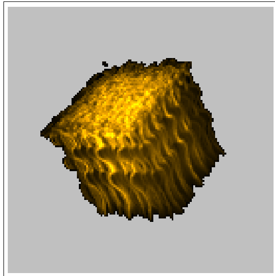
Figure 7.3: A 3D fuzzy texture with clustering in the unit cube
