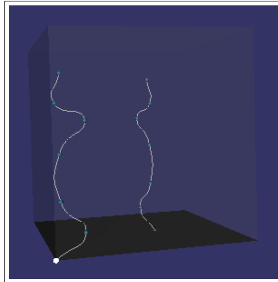
Figure 3.4: Some seed strands for the unit cube
