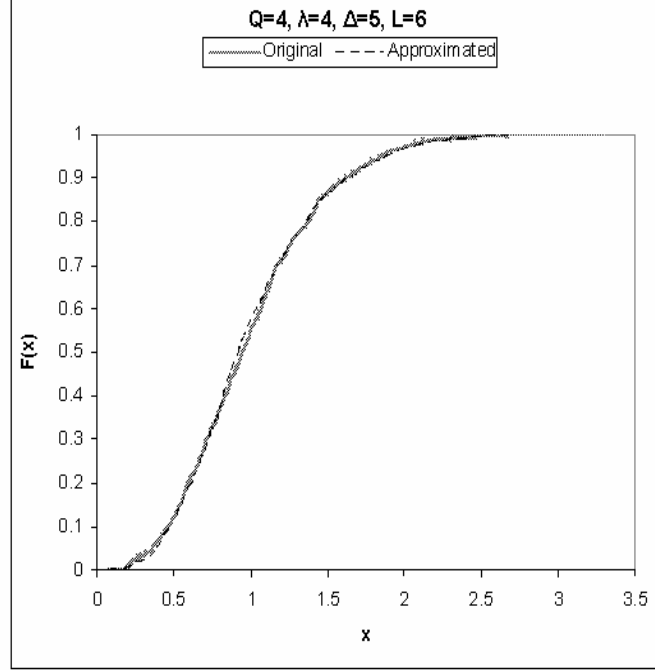
Figure 3.5: Comparison of the Erlang Approximation with the Queue Inter-arrival Times
